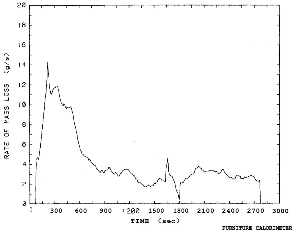
Figure 14. Rate of mass loss plot for easy chair Test 49
