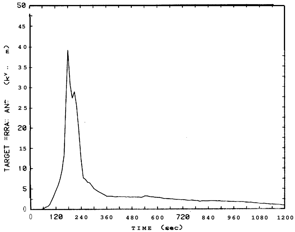
Figure 115. Target irradiance plot for 3.2 mm plywood painted inside and out with two coats of fire-retardant latex paint, Test 44
