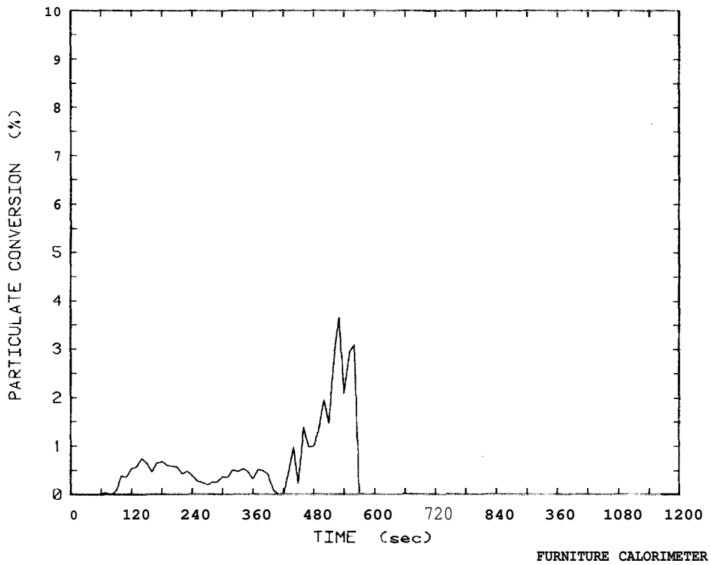
Figure 89. Smoke particulate conversion plot for metal wardrobe, Test 21
