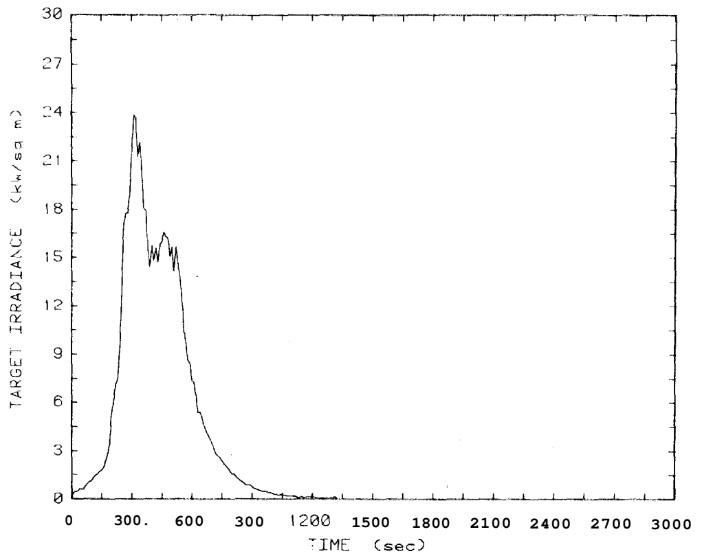
Figure 10: Target irradiance plot for easy chair, Test 48
