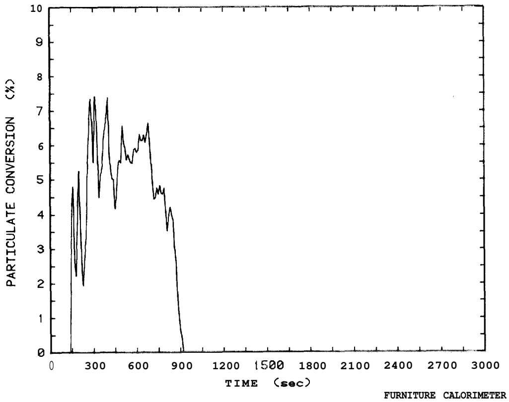
Figure 72. Smoke particulate conversion plot for metal. frame loveseat, Test 54
