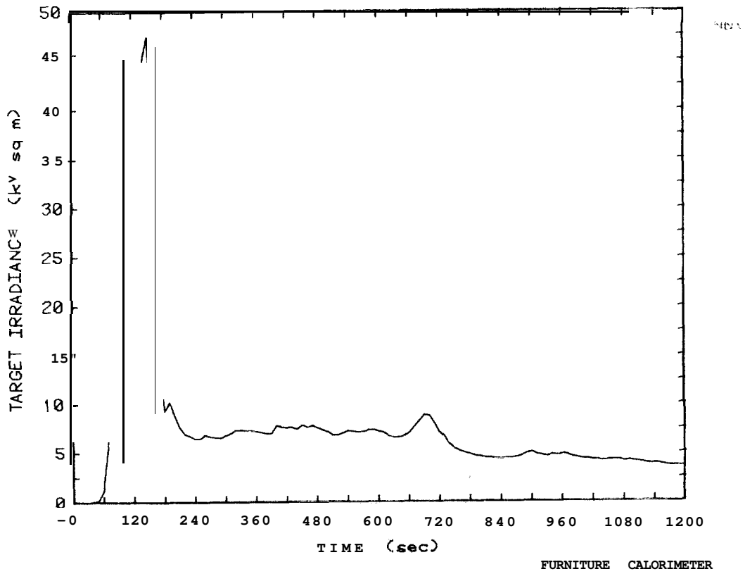
Figure 93. Target irradiance plot for 12.7 mm plywood wardrobe Test 39
