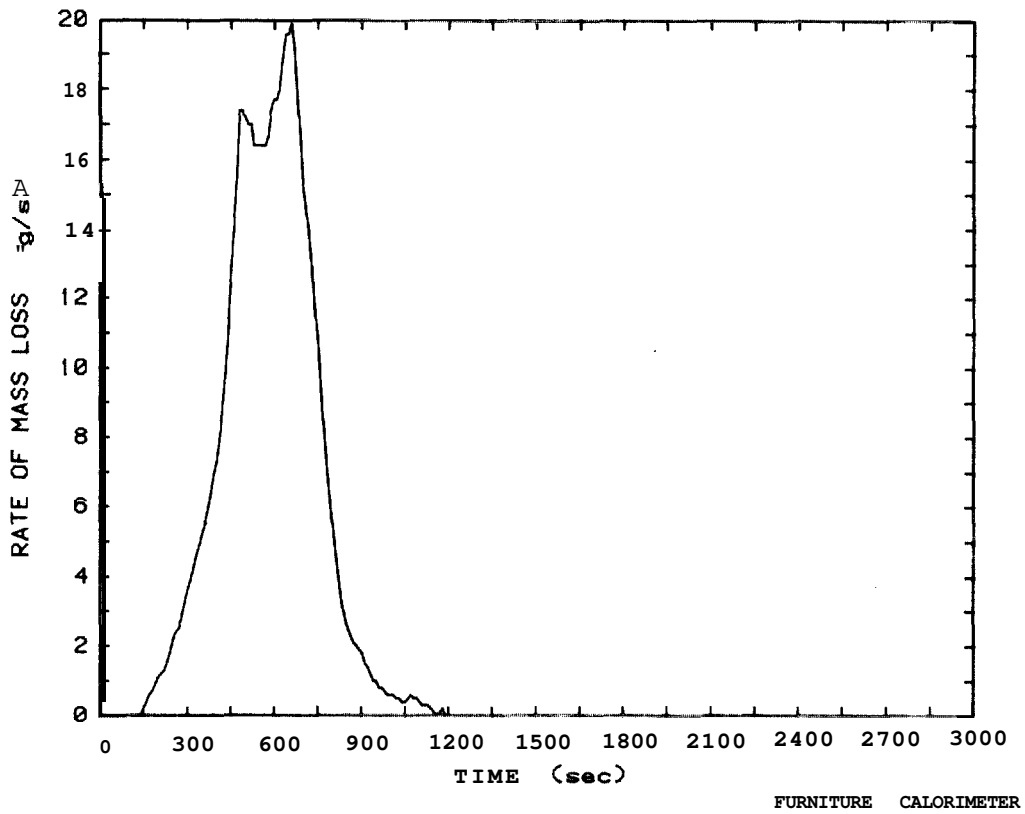
Figure 70. Rate of mass loss plot for metal loveseat, Test 54
