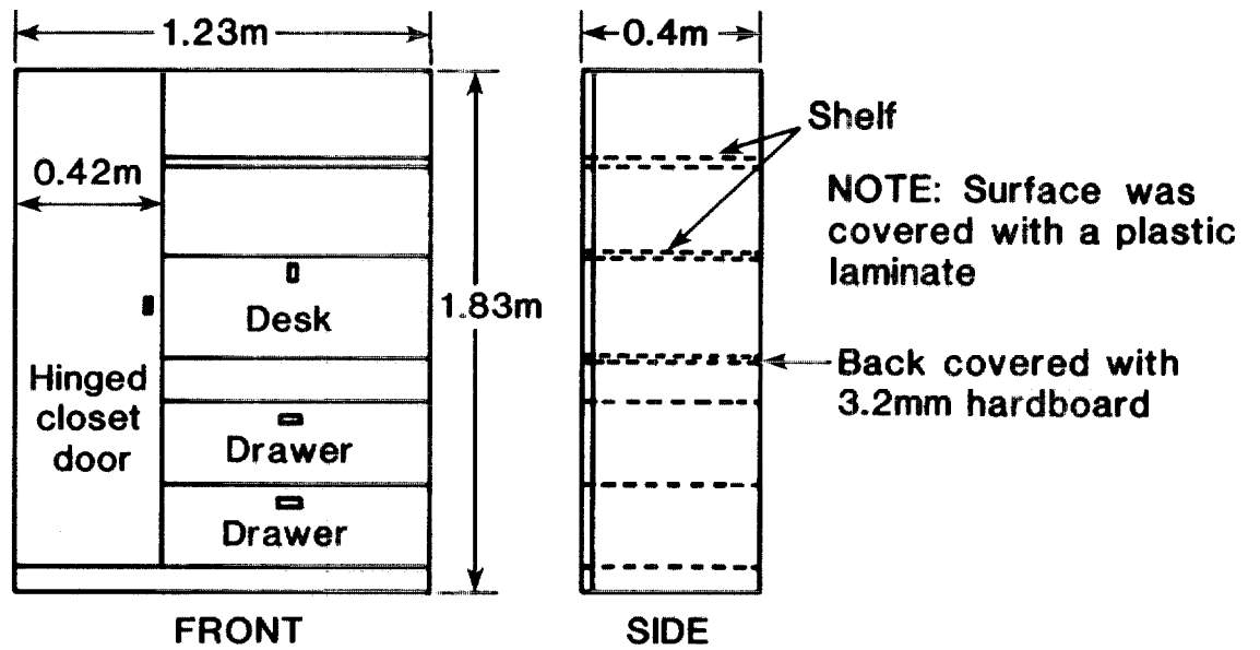
Figure 120. Photograph and sketch of .9.1 mm particleboard wardrobe, test 61
