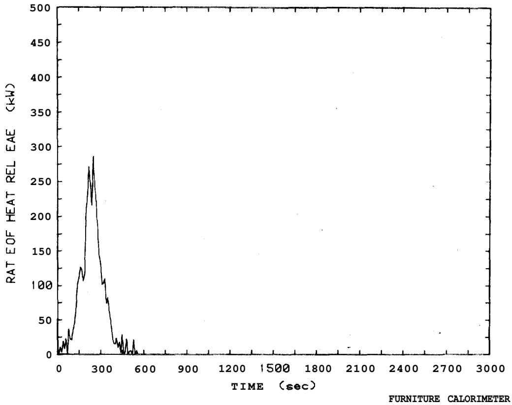
Figure 44: Rate of heat release plot for metal frame chair, Test 53
