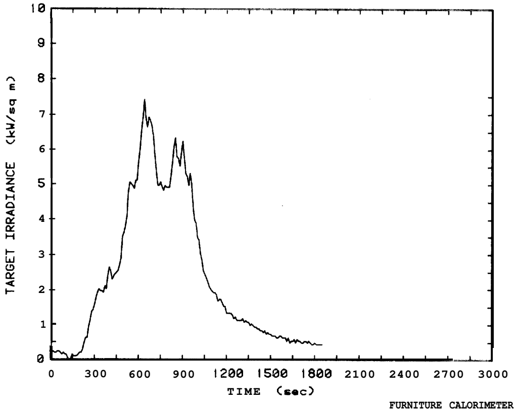
Figure 80. Target irradiance plot for mattress and boxspring, Test 67
