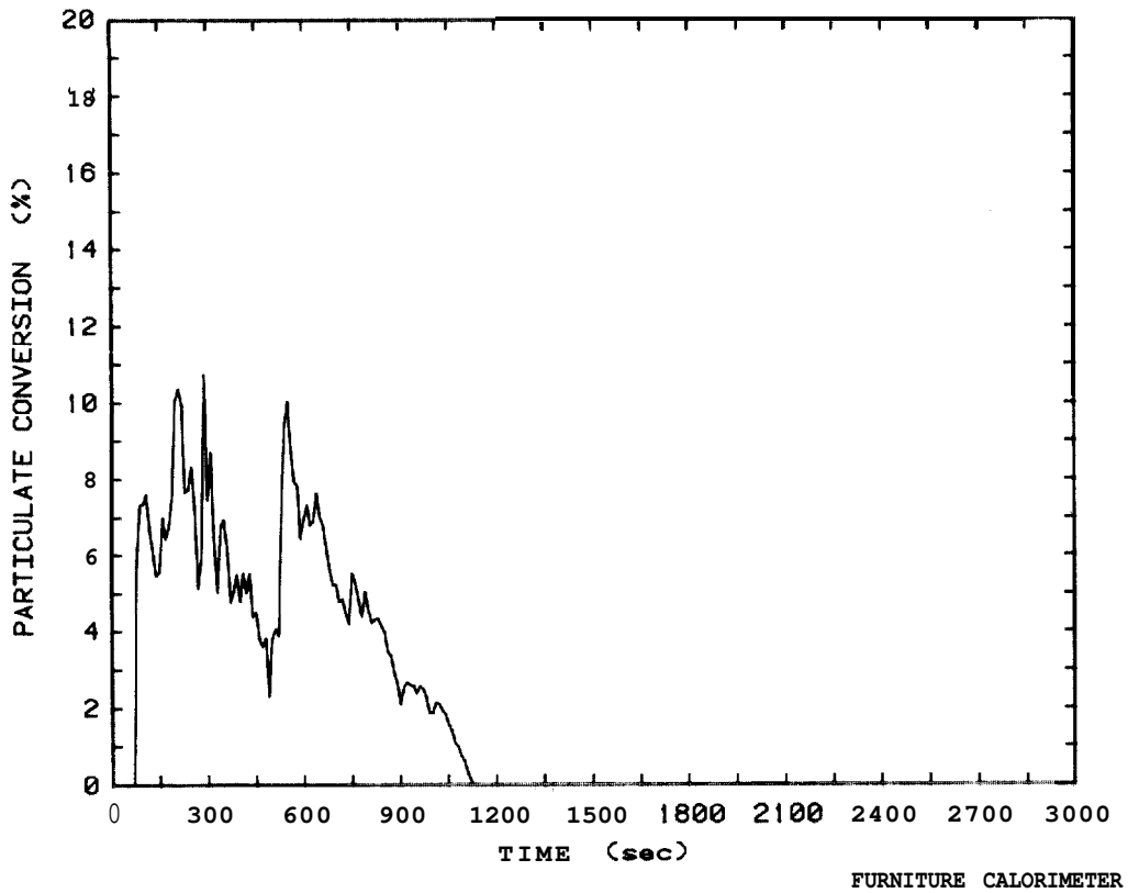
Figure 77. Smoke particulate conversion plot for wood frame loveseat, Test 57
