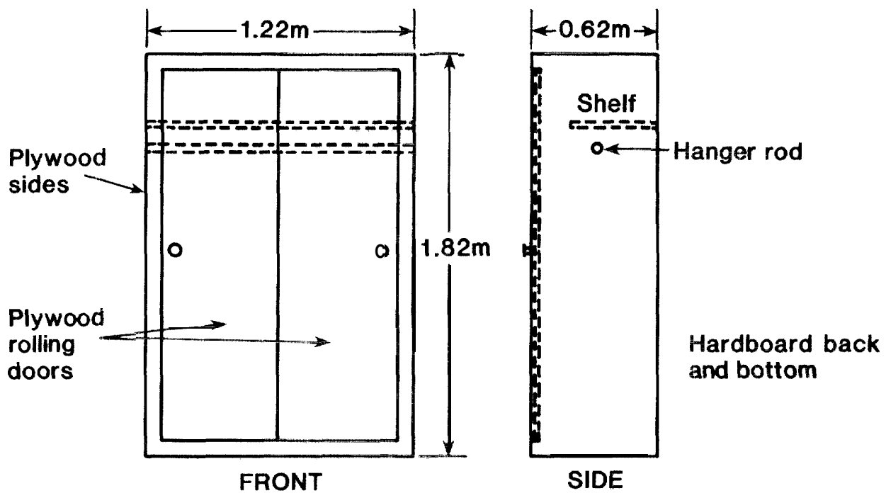
Figure .03. Photograph and sketch of 3.2 mm plywood wardrobe
