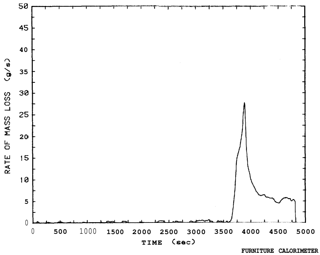
Figure 24: Rate of mass loss plot for easy chair Test 66
