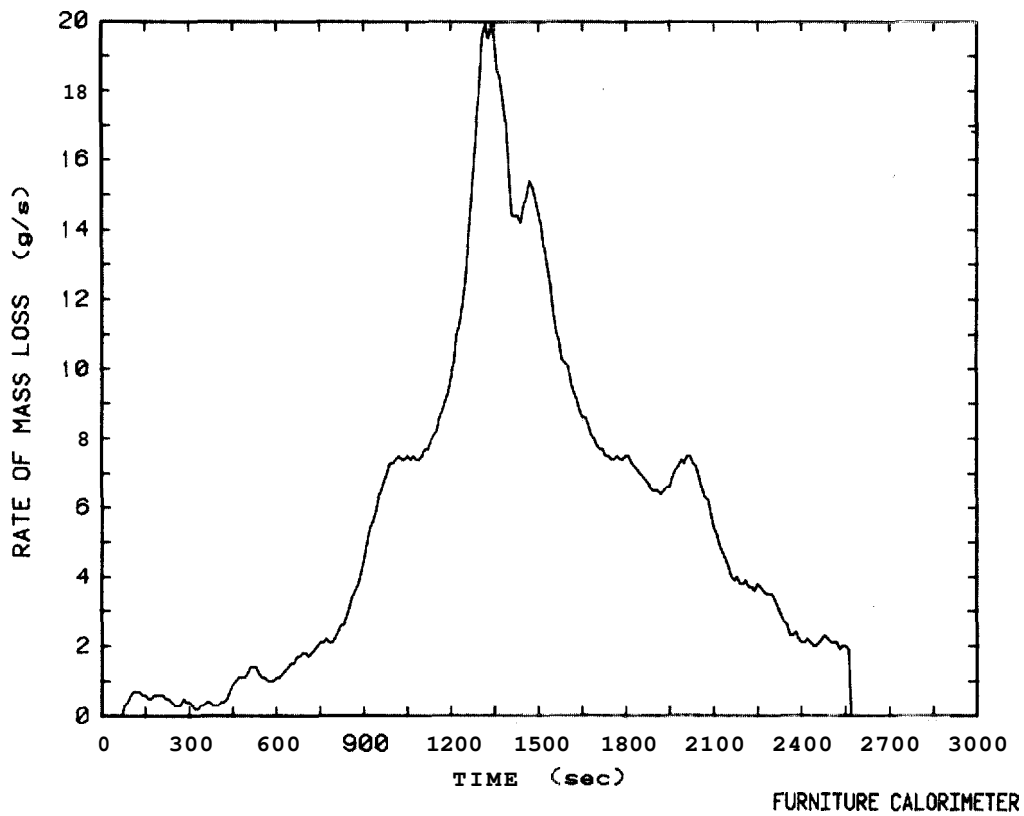
Figure 19. Rate of mass loss plot for easy chair Test 64
