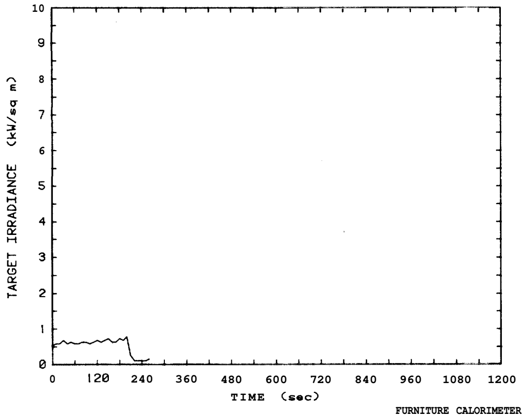
Figure 33: Target irradiance plot for minimum cushion chair, Test 50
