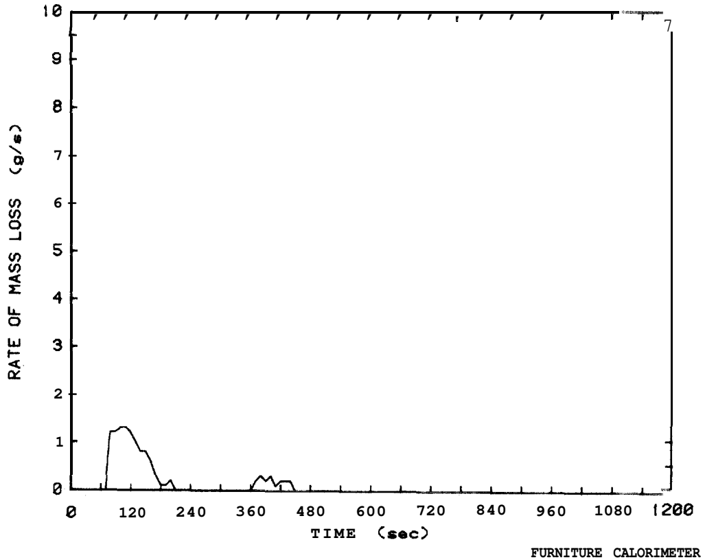
Figure 36: Rate of mass loss plot for molded fiberglass chair, Test 51
