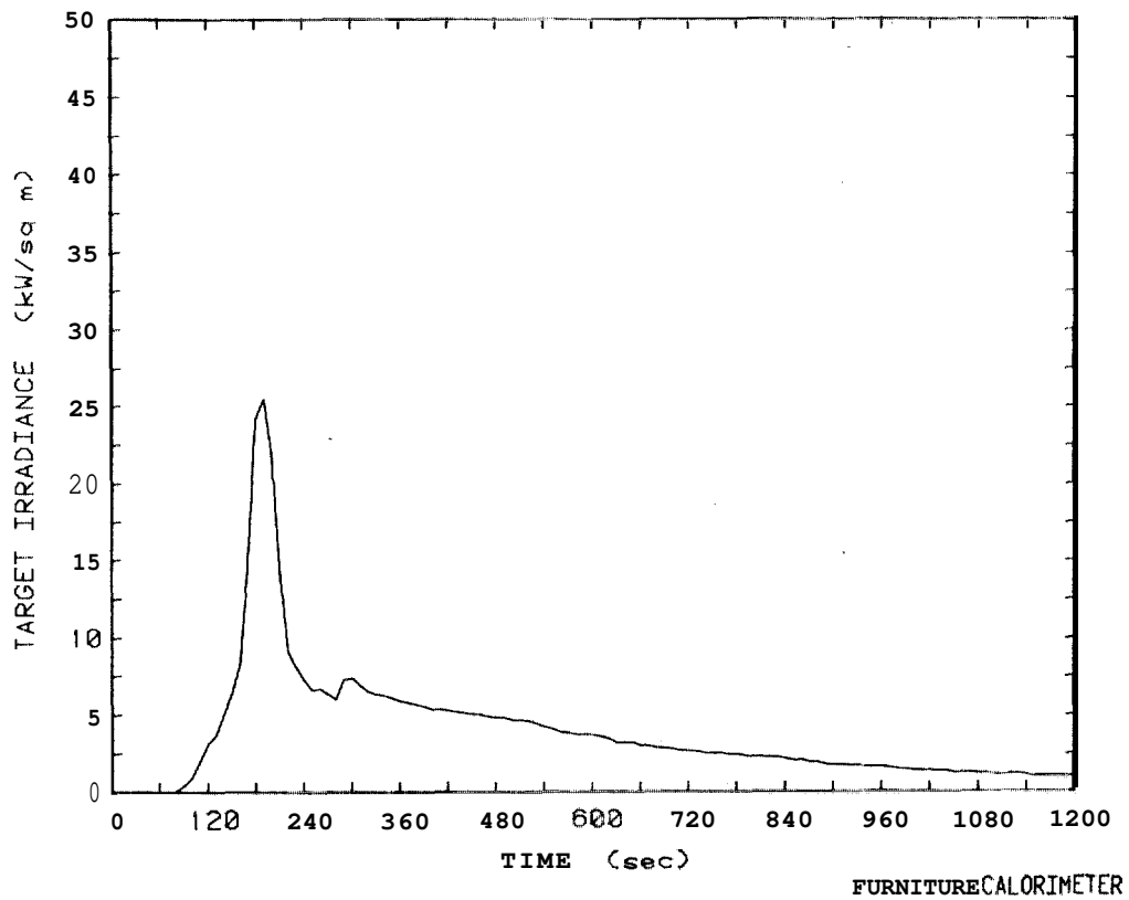
Figure 110. Target irradiance plot for 3.2 mm plywood wardrobe painted inside with one coat of fire-retardant paint, Test 42
