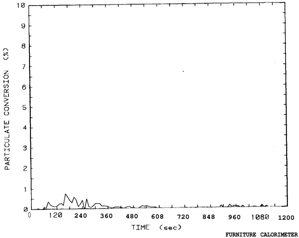
Figure 107. Smoke particulate conversion for 3.2 mm plywood wardrobe, Test 41
