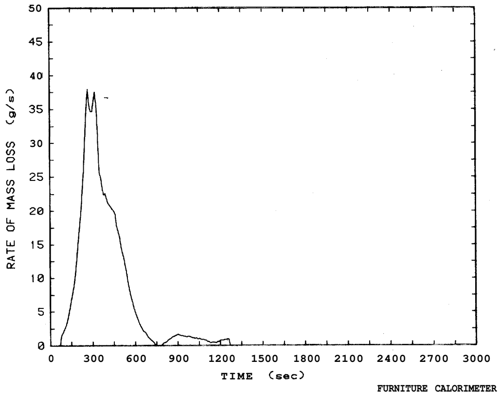
Figure 9: Rate of mass loss plot for easy chair, Test 48
