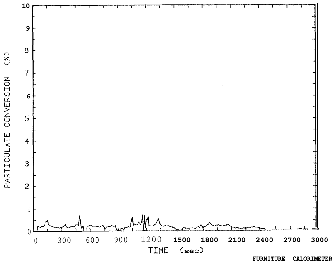
Figure 124: Smoke particulate conversion plot for 19.1 mm particleboard wardrobe, Test 61
