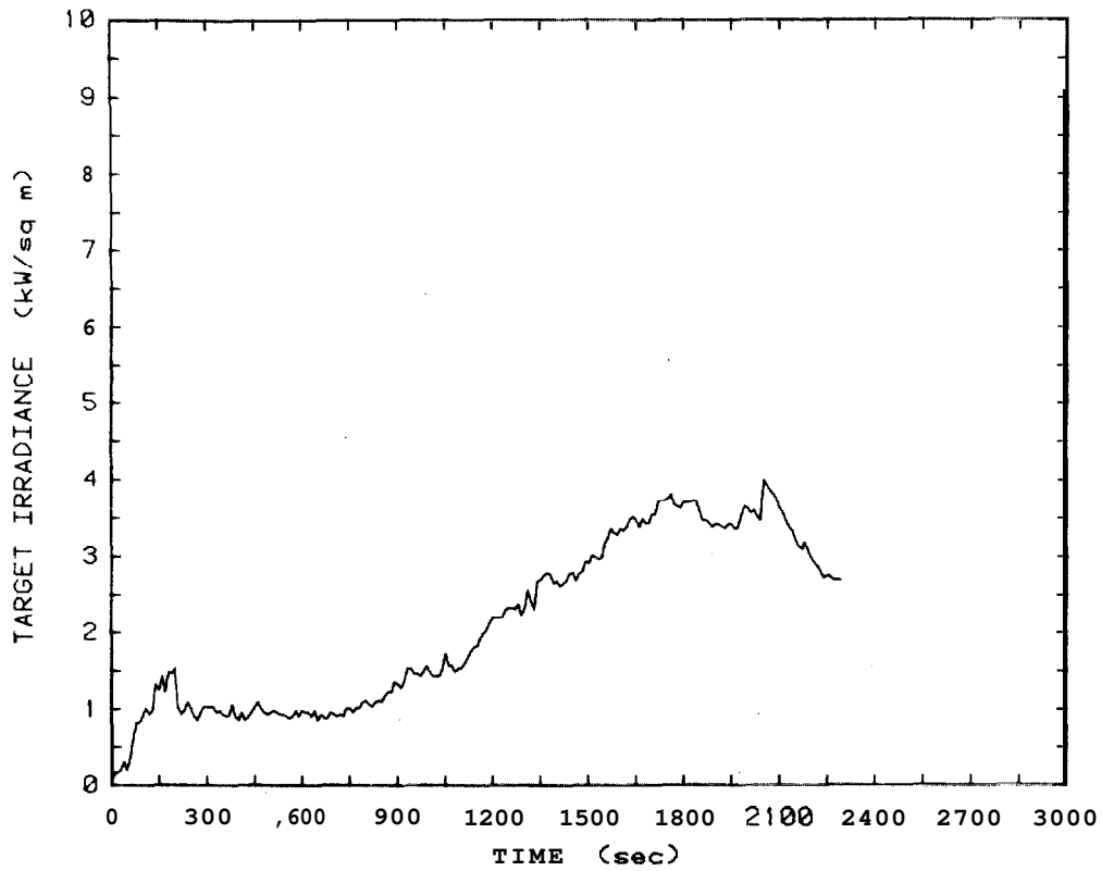
Figure 61. Target irradiance plot for metal frame stackable chairs, Test 75
