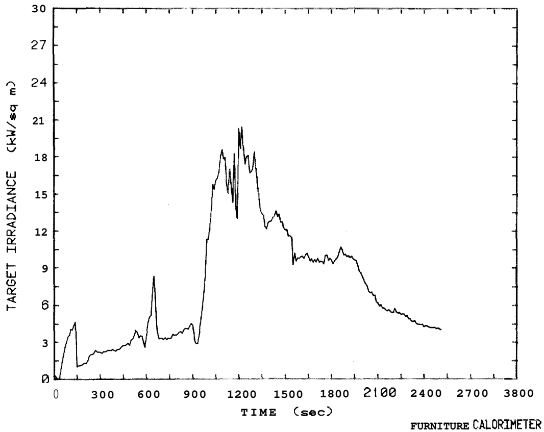
Figure 123: Target irradiance plot for 19.1 mm particleboard wardrobe, Test 61
