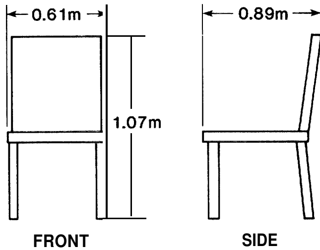
Figure 26. Photograph and dimensions of adjustable back patient chair, test 47
