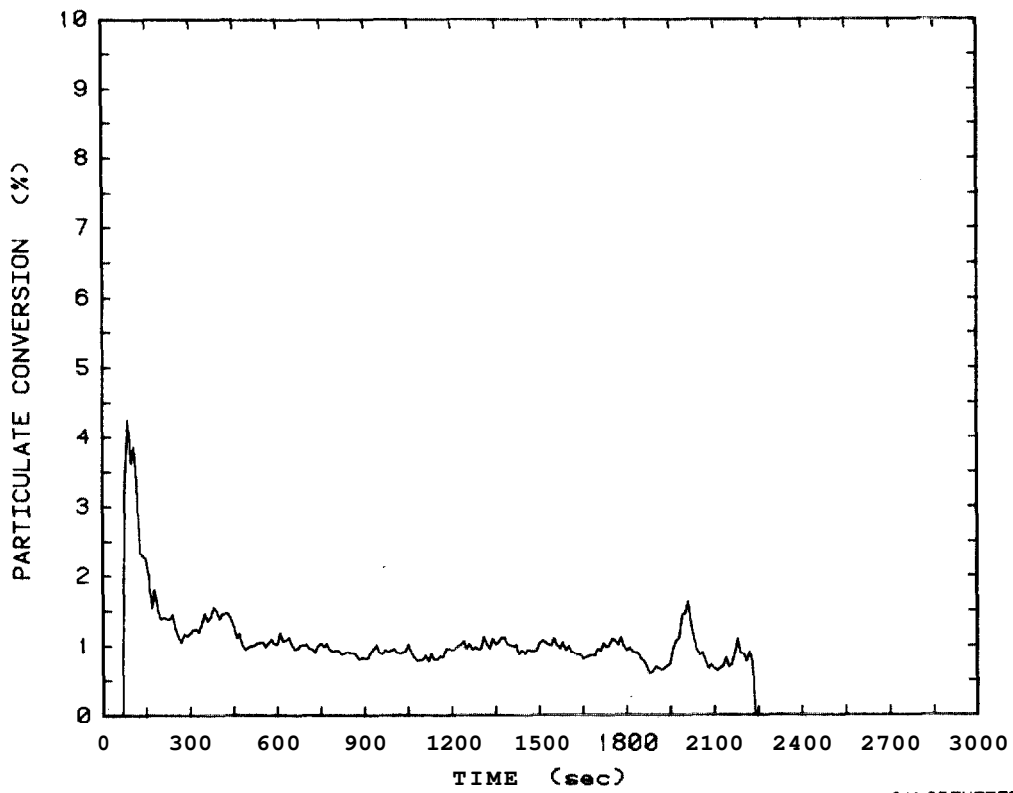
Figure 62. Smoke particulate conversion plot for metal frame stackable chairs, Test 75
