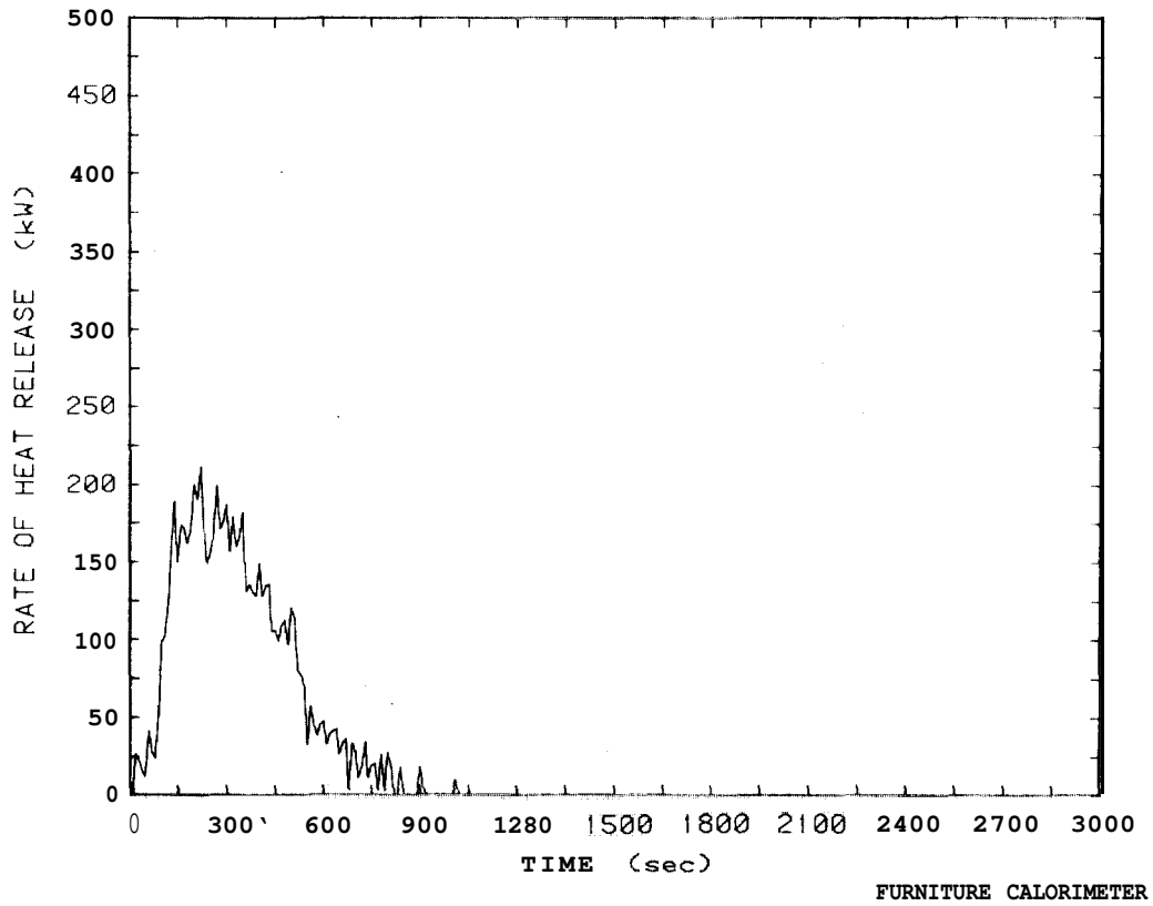
Figure 13. Rate of heat release plot for easy chair Test 49
