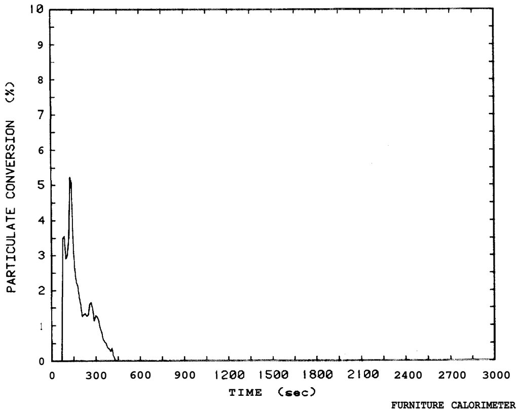
Figure 30: Smoke particulate conversion plot for patient chair Test 47
