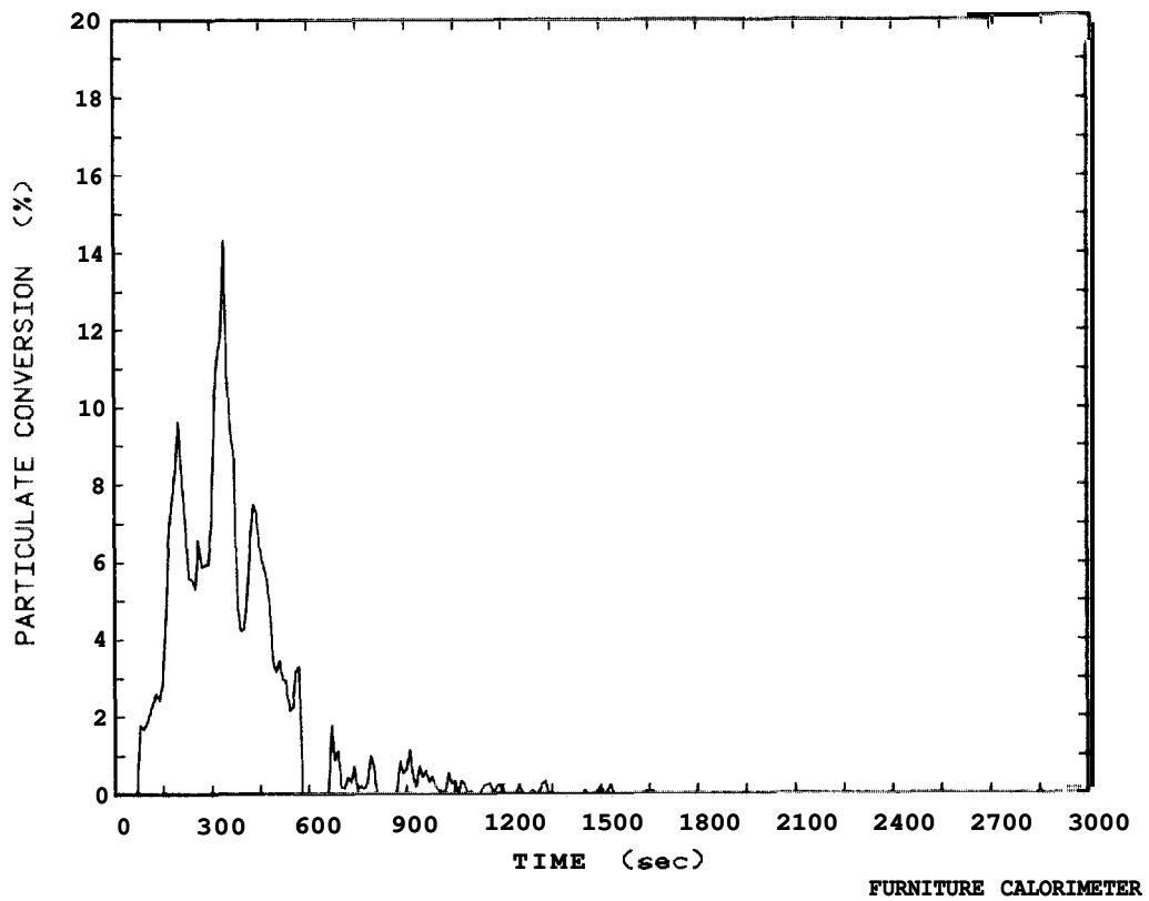
Figure 57: Smoke particulate conversion plot for chair with latex foam cushions, Test 56
