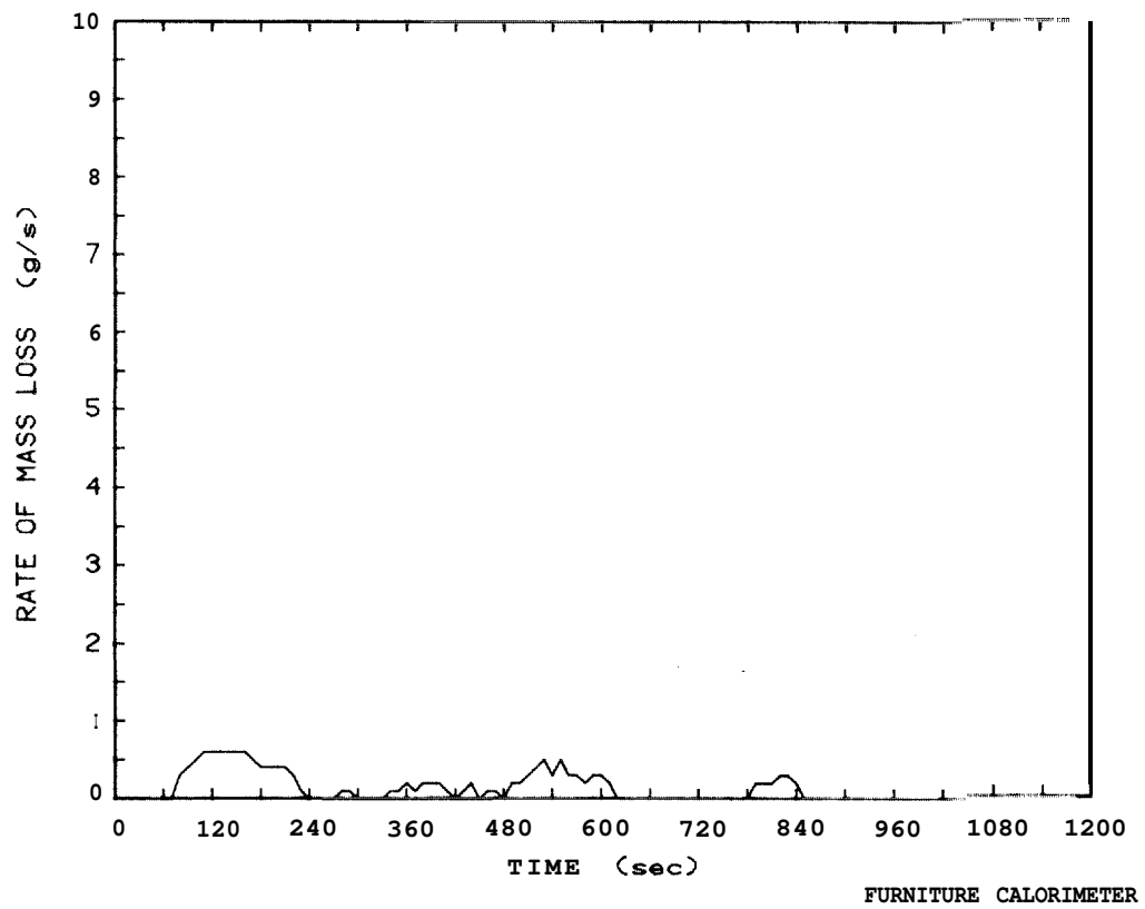
Figure 50: Rate of mass loss plot for chair from group setting, Test 55
