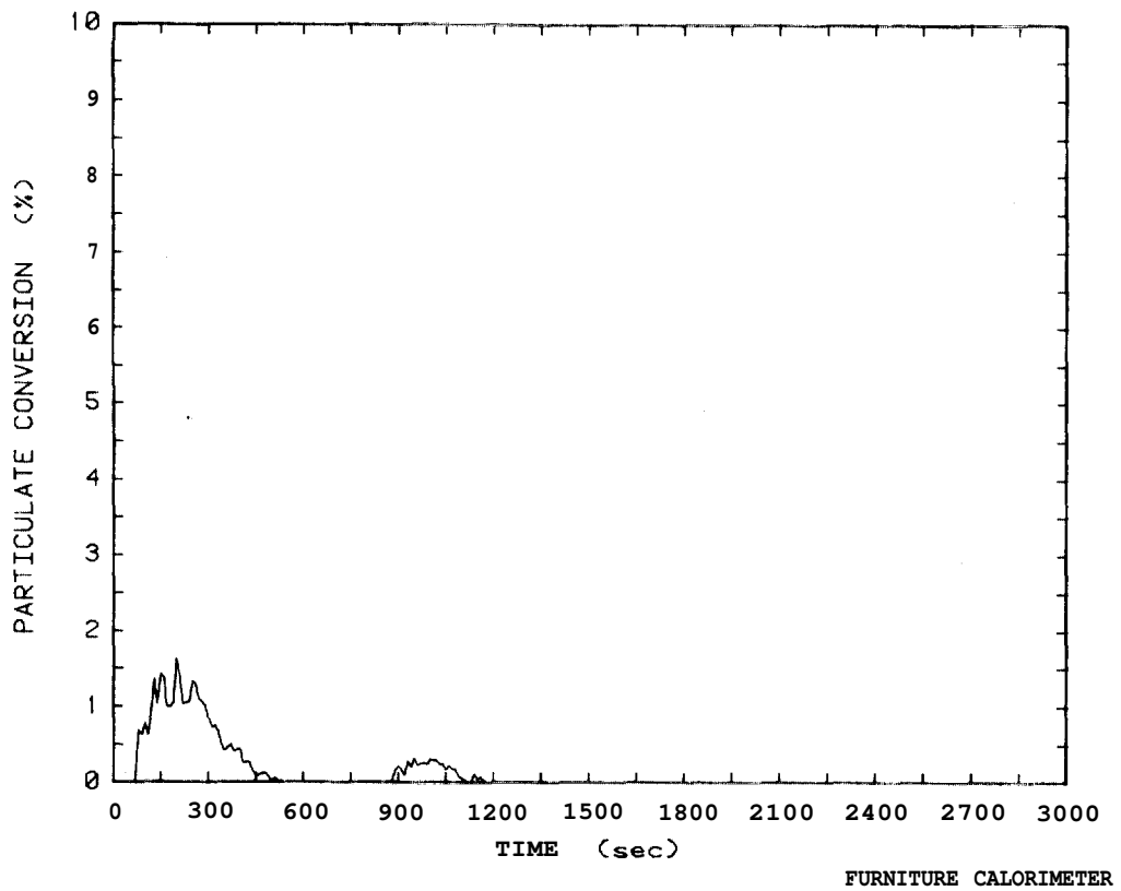
Figure 16. Smoke particulate conversion plot for easy chair Test 49
