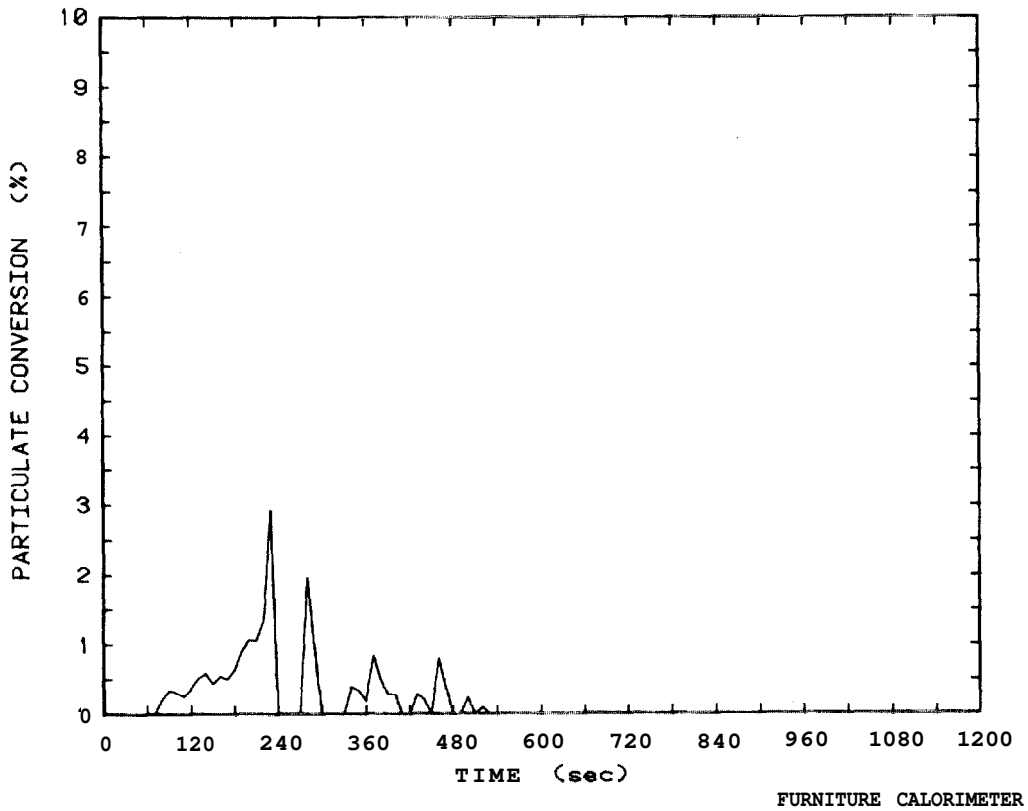
Figure 52: Smoke particulate conversion plot for chair from group setting, Test 55
