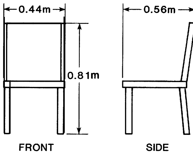
Figure 58. Photograph and dimensions of metal frame stackable chairs, test 75
