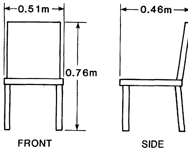
Figure 48. Photograph and dimensions of chair from group setting, test 55
