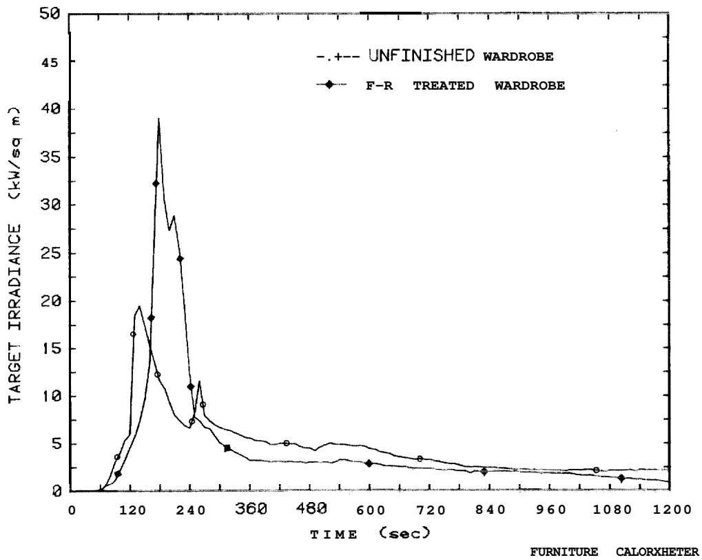
Figure 118. Comparison of target irradiances experienced in Test 41 and Test 44
