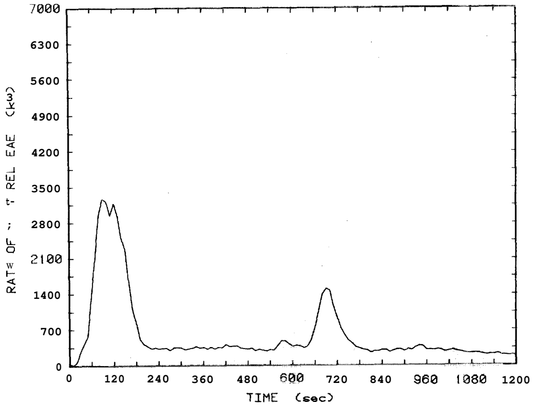
Figure 91. Rate of heat release plot for 12.7 mm plywood wardrobe, Test 39
