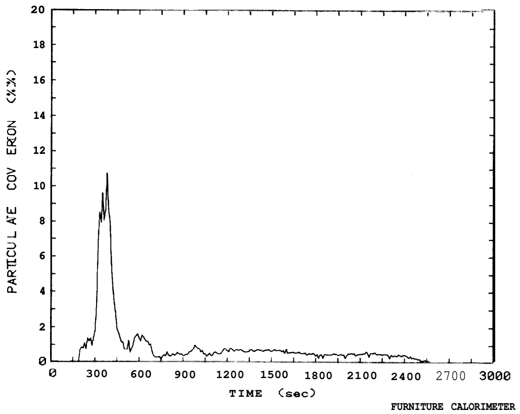
Figure 21. Smoke particulate conversion plot for easy chair Test 64
