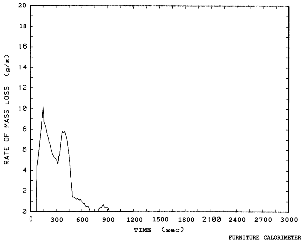
Figure 28: Rate of mass loss plot for patient chair Test 47
