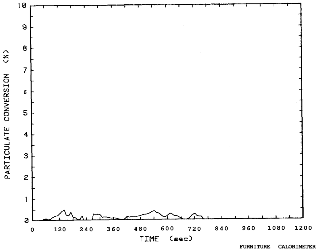
Figure 94. Smoke particulate conversion plot for 12.7 mm plywood wardrobe, Test 39
