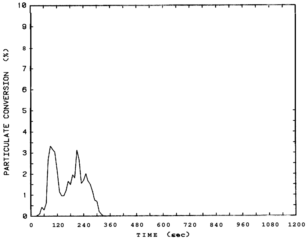
Figure 116. Smoke particulate conversion plot for 3.2 mm plywood wardrobe painted inside and out with two coats of fire-retardant latex paint, Test 44
