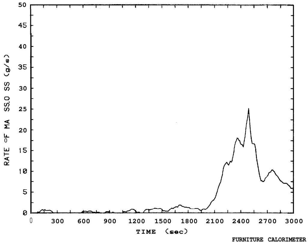
Figure 40: Rate of mass loss plot for molded plastic patient chair, Test 52
