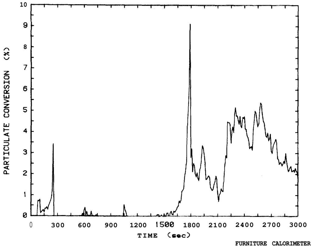
Figure 42: Smoke particulate conversion plot for molded plastic patient chair, Test 52
