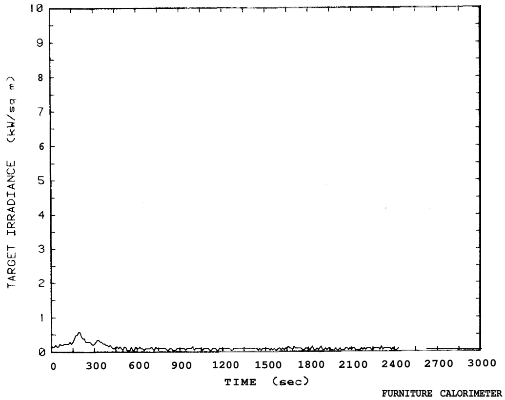
Figure 56: Target irradiance plot for chair with latex foam cushions, Test 56
