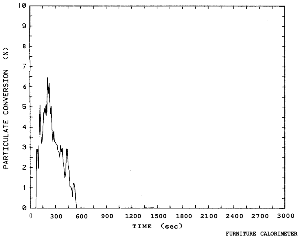
Figure 47: Smoke particulate conversion plot for metal frame chair, Test 53
