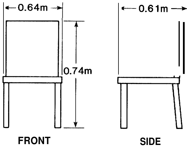
Figure 34. Photograph and dimensions of molded fiberglass chair, test 51
