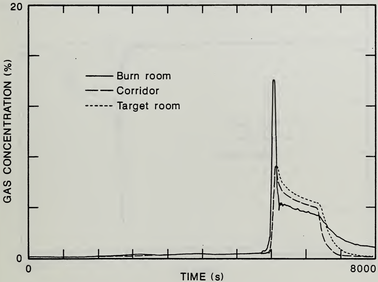
Figure 77. Comparison of Carbon Dioxide Concentrations in Each Compartment of the Large-Scale Test Facility for the Two-Cigarette Test of Foam 32X Mock-up Upholstery Chair Assembly With the Animal Exposure Chambers Connected to the Burn Room.
