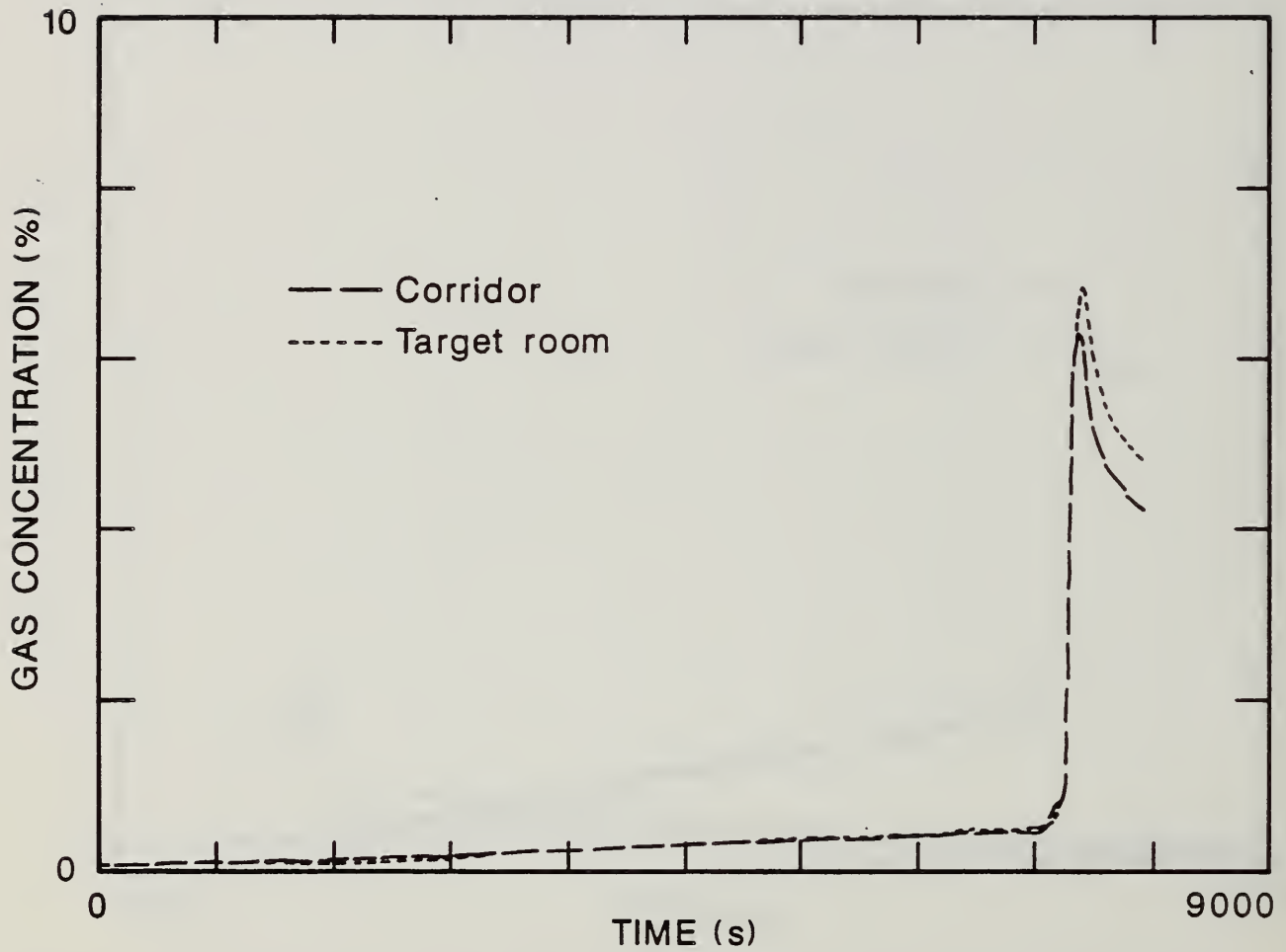
Figure 82. Comparison of Carbon Dioxide Concentrations in Each Compartment of the Large-Scale Test Facility for the Two-Cigarette Test of Foam 32X Mock-up Upholstery Chair Assembly With the Animal Exposure Chambers Connected to the Target Room.
