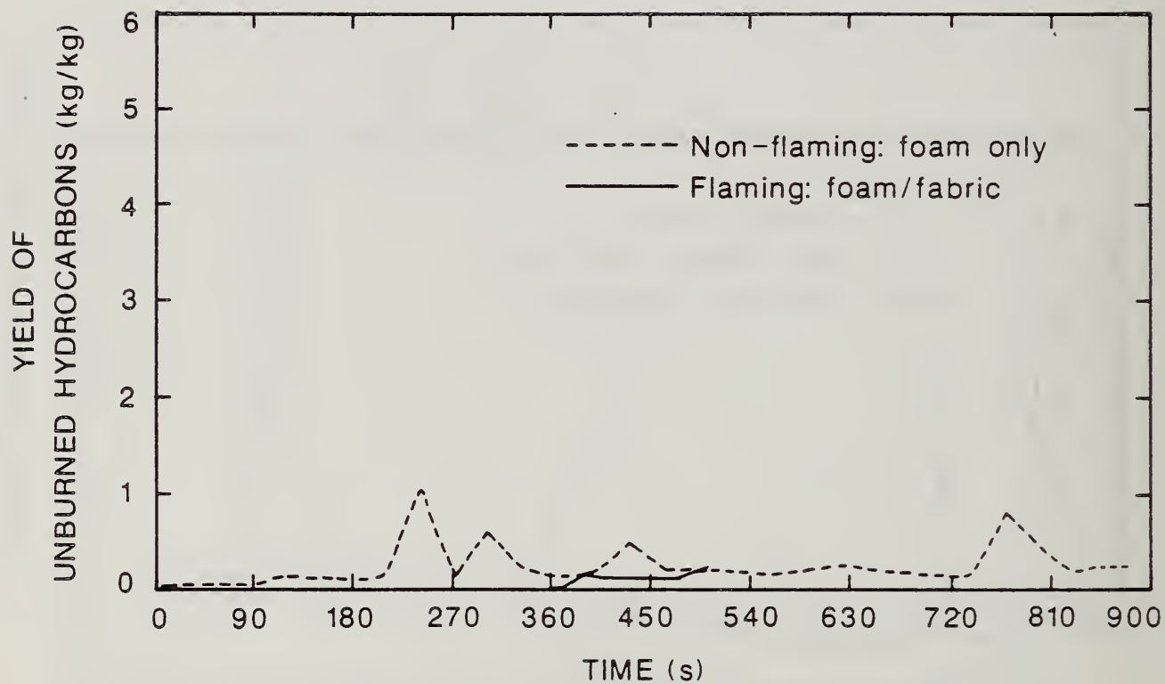
Figure 8. Comparison of Unburned Hydrocarbons for Foam 32 Flaming and Non-flaming Exposures Without a Cover Fabric and Flaming Exposure With a Cover Fabric.
