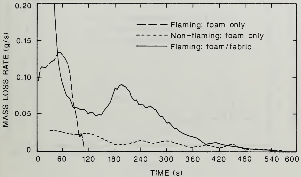
Figure 11. Comparison of Mass Loss Rate for Foam 32X Flaming and Non-flaming Exposures Without a Cover Fabric and Flaming Exposure With a Cover Fabric.
