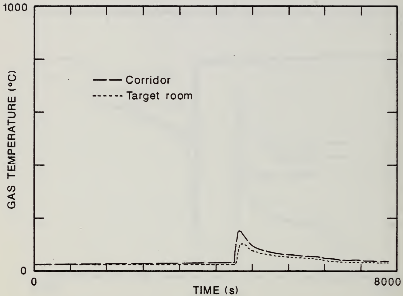
Figure 74. Comparison of the Upper Compartment Gas Temperatures in Each Compartment of the Large-Scale Test Facility for the Two-Cigarette Test of Foam 32 Mock-up Upholstery Chair Assembly With the Animal Exposure Chamber Connected to the Target Room.
