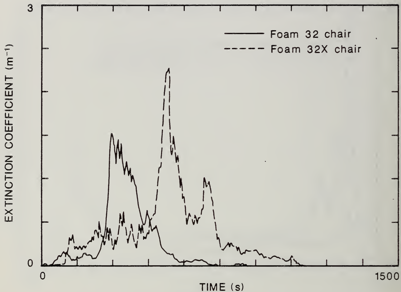
Figure 28. Comparison of the Smoke Extinction Coefficient for the Flaming Ignition of Mock-up Foams 32 and 32X Upholstery Chairs Tested in the Furniture Calorimeter.
