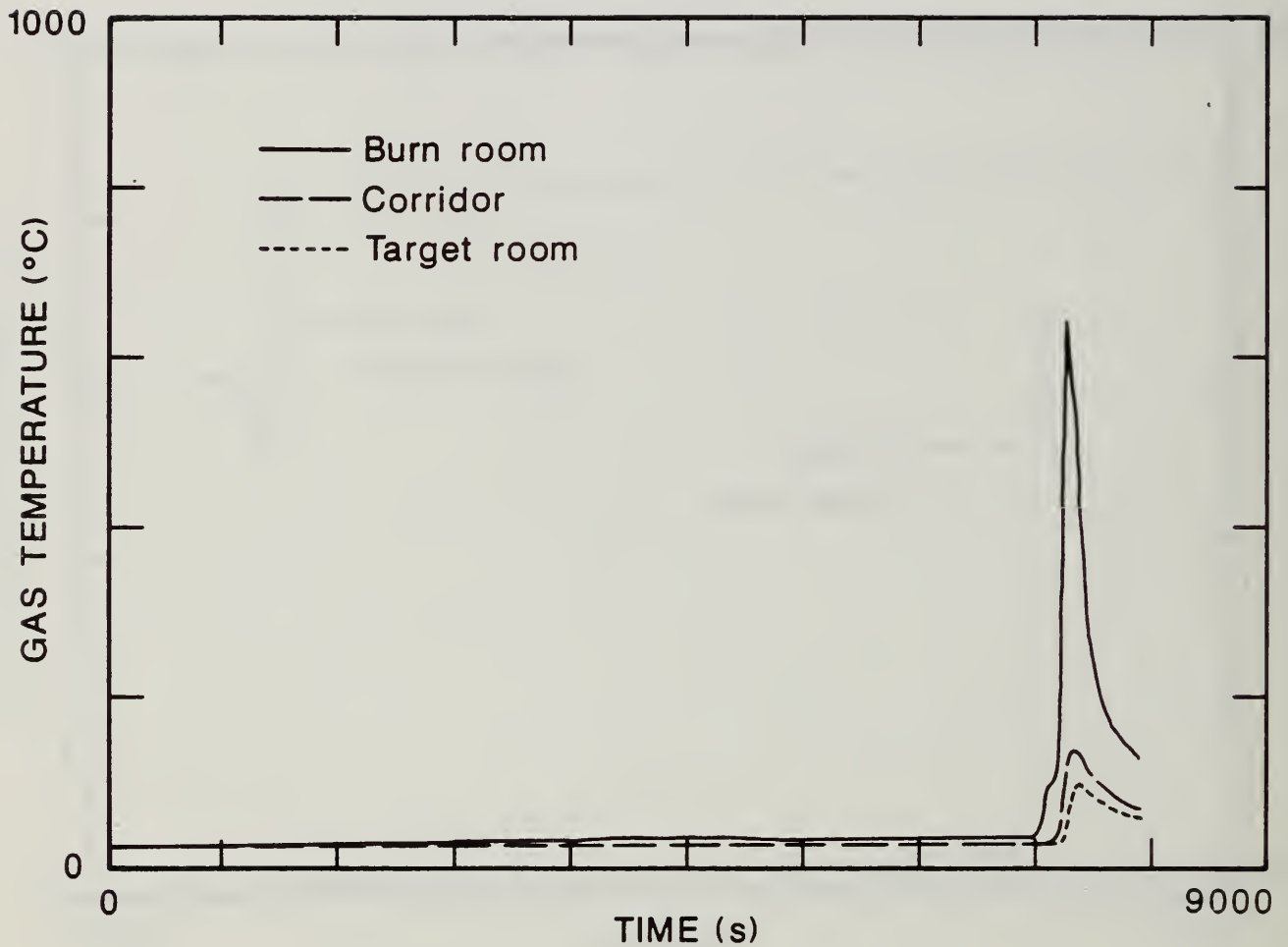
Figure 84. Comparison of Upper Compartment Gas Temperatures in Each Compartment of the Large-Scale Test Facility for the Two-Cigarette Test of Foam 32X Mock-up Upholstery Chair Assembly With the Animal Exposure Chambers Connected to the Target Room.
