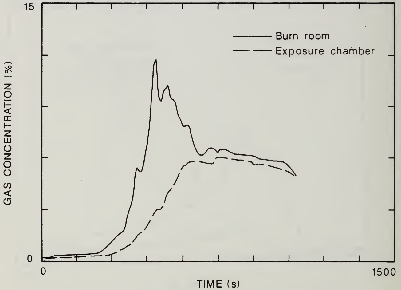
Figure 48. Comparison of Carbon Dioxide Concentration in the Burn Room and the Animal Exposure Chamber for Flaming Ignition of Foam Mock-up Upholstery Chair Assembly.
