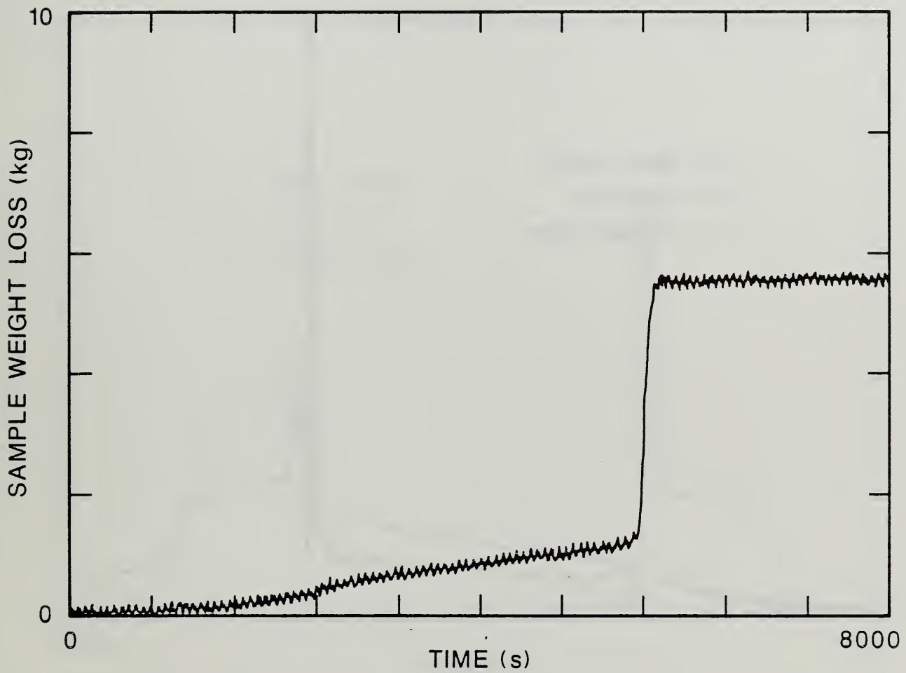
Figure 75. Mass Loss of Upholstery Chair Assembly Made from Foam 32X and Exposed to Two-Cigarettes in the Large-Scale Test Facility With the Animal Exposure Chambers Connected to the Burn Room.
