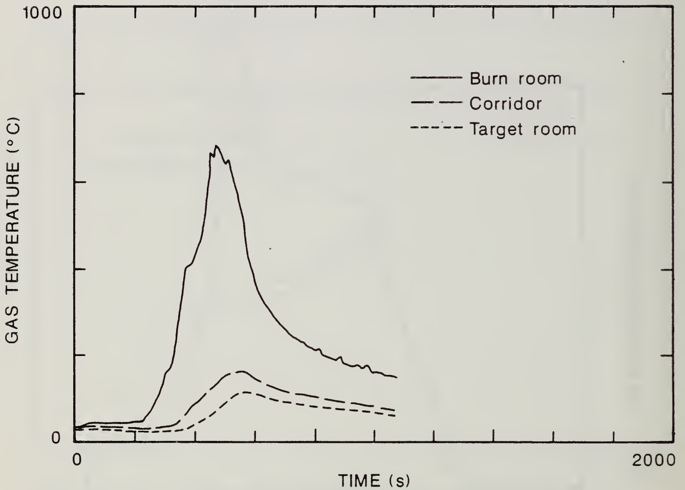
Figure 46. Upper Layer Gas Temperatures in Each Compartment of the Large-Scale Facility During Flaming Ignition test of Foam 32 Mock-up Upholstery Chair Assembly.
