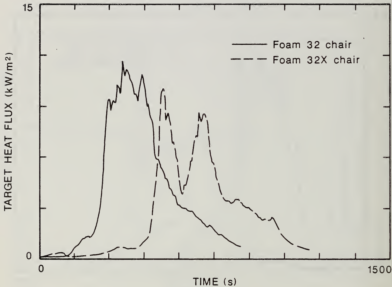
Figure 22. Furniture Calorimeter Data Comparing the Heat Flux Received by a Target Material from the Flaming Ignition of Mock-up Upholstery Chairs made from Foam 32 and Foam 32X.
