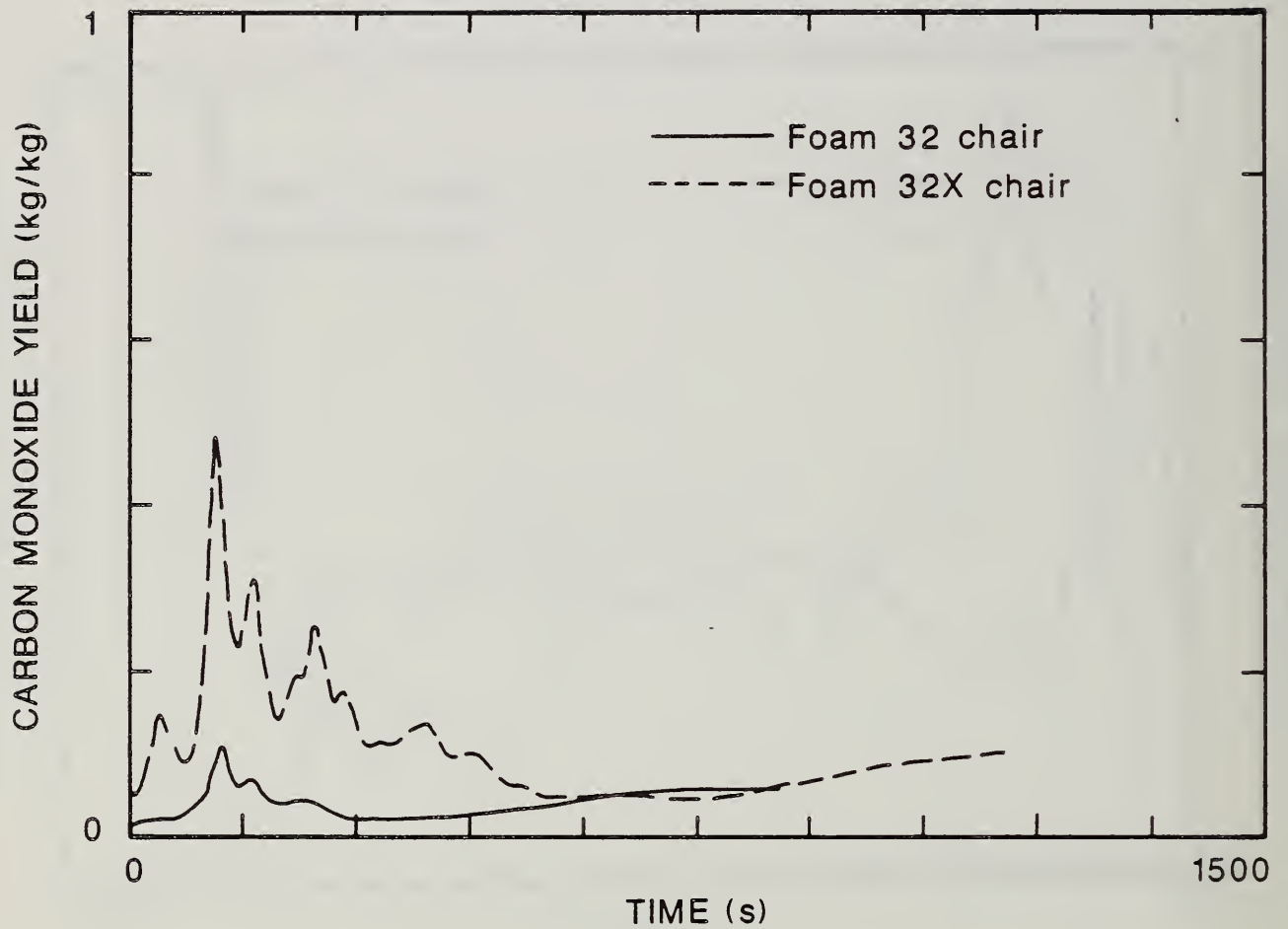
Figure 26. Comparison of Carbon Monoxide Yield for the Flaming Ignition of Foams 32 and 32X Mock-up Chairs Tested in the Furniture Calorimeter.
