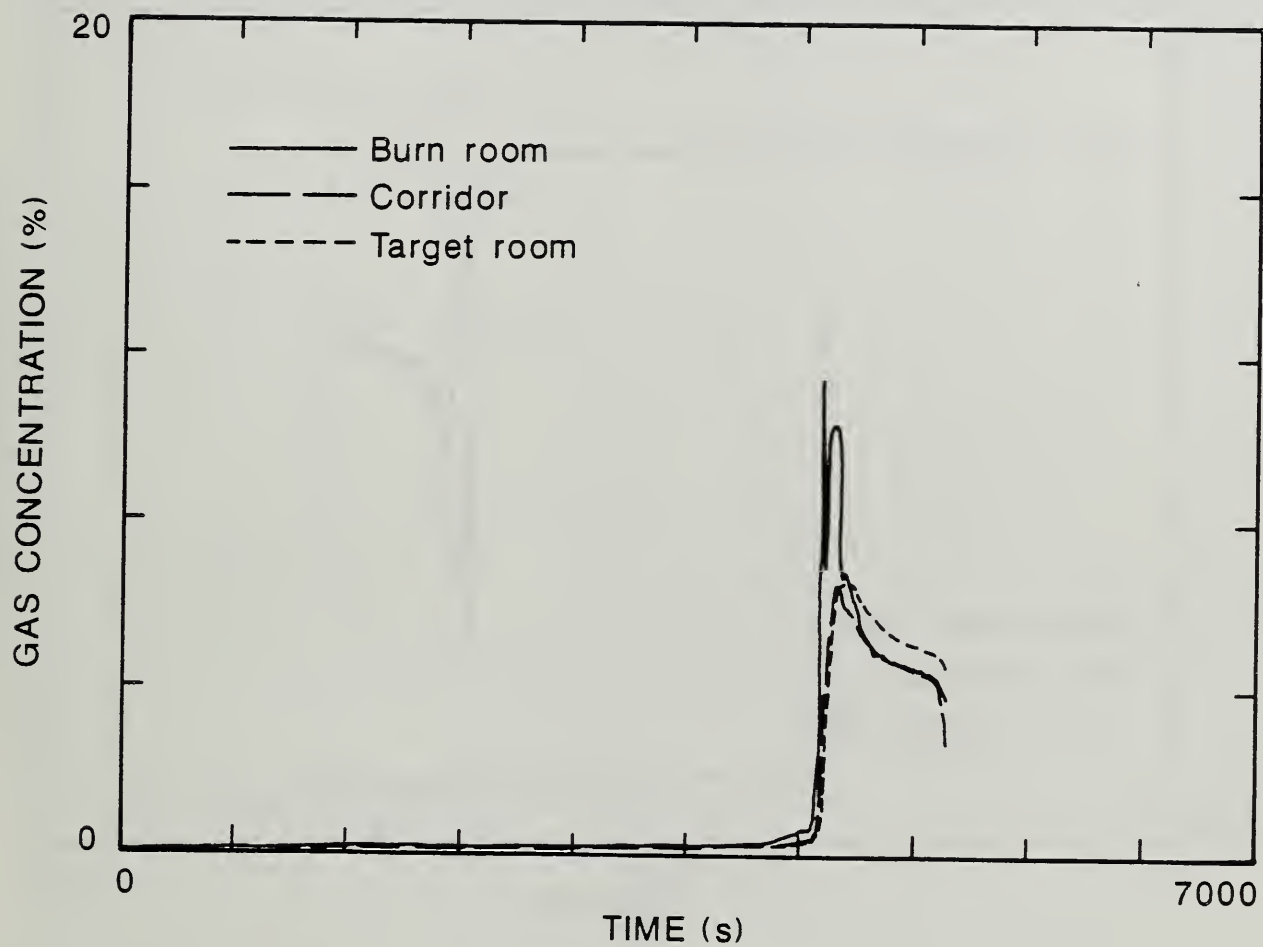
Figure 61. Comparison of Carbon Dioxide Concentrations in Each Compartment of the Large-Scale Test Facility for the Two-Cigarette Test of Foam 32X Mock-up Upholstery Chair Assembly.
