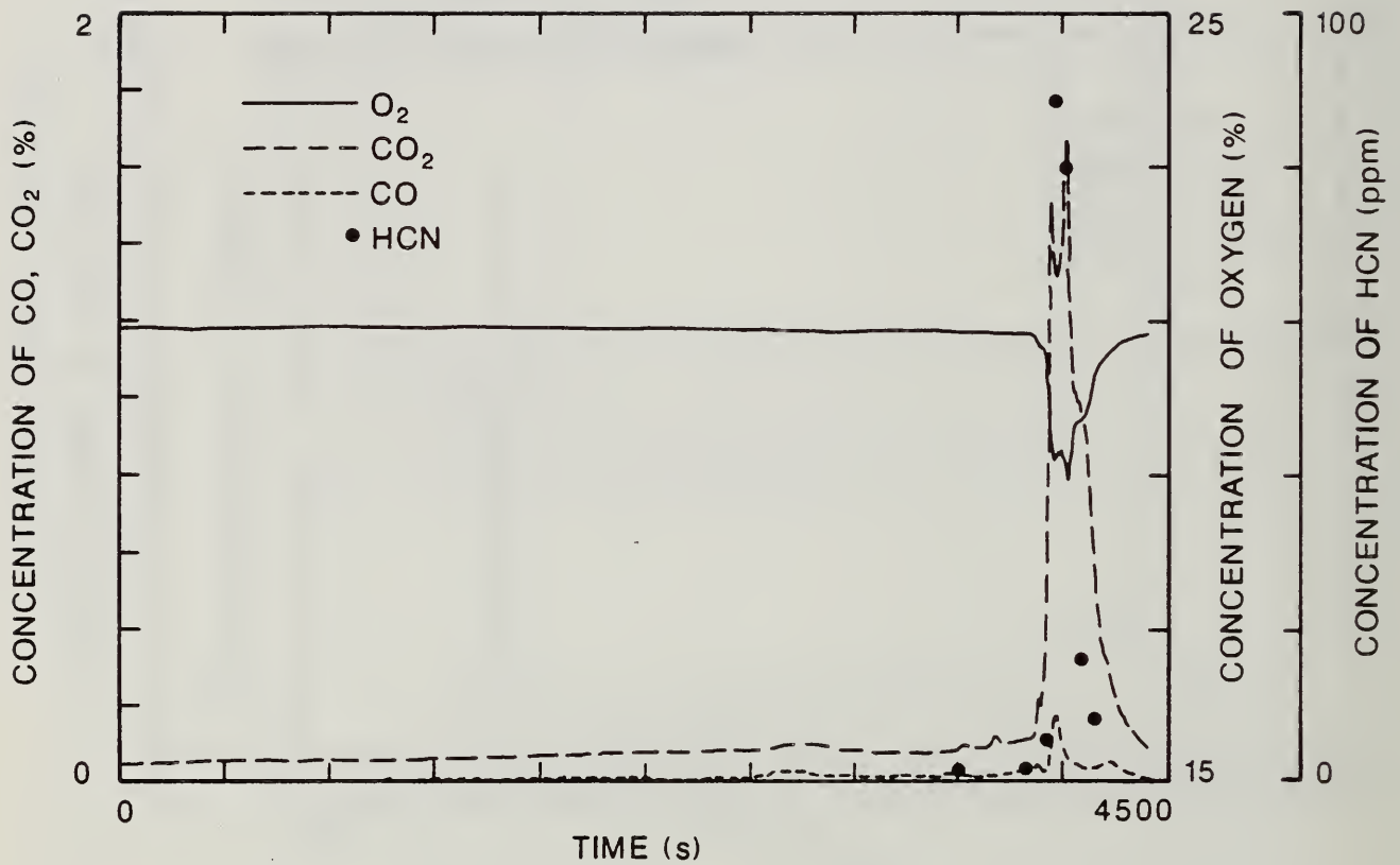
Figure 32. Concentration of CO 2 , CO, HCN, and Oxygen During the Smoldering-to-Flaming Ignition of Foam 32X Mock-up Upholstery Chairs Tested in the Furniture Calorimeter.
