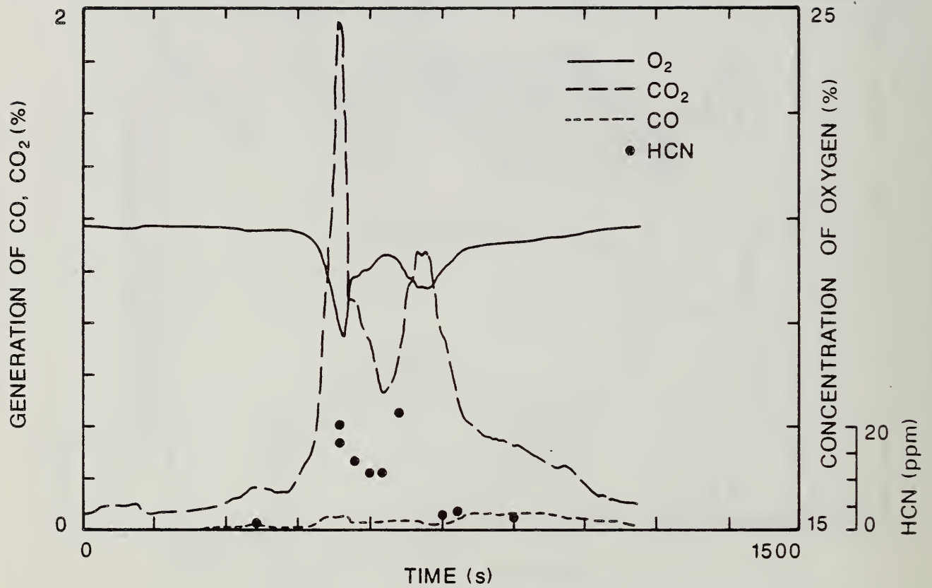
Figure 20. Furniture Calorimeter Data for the Concentration of Carbon Dioxide, Carbon Monoxide, HCN, and Oxygen for Flaming Ignition of Mock-up Chairs made with Foam 32X.
