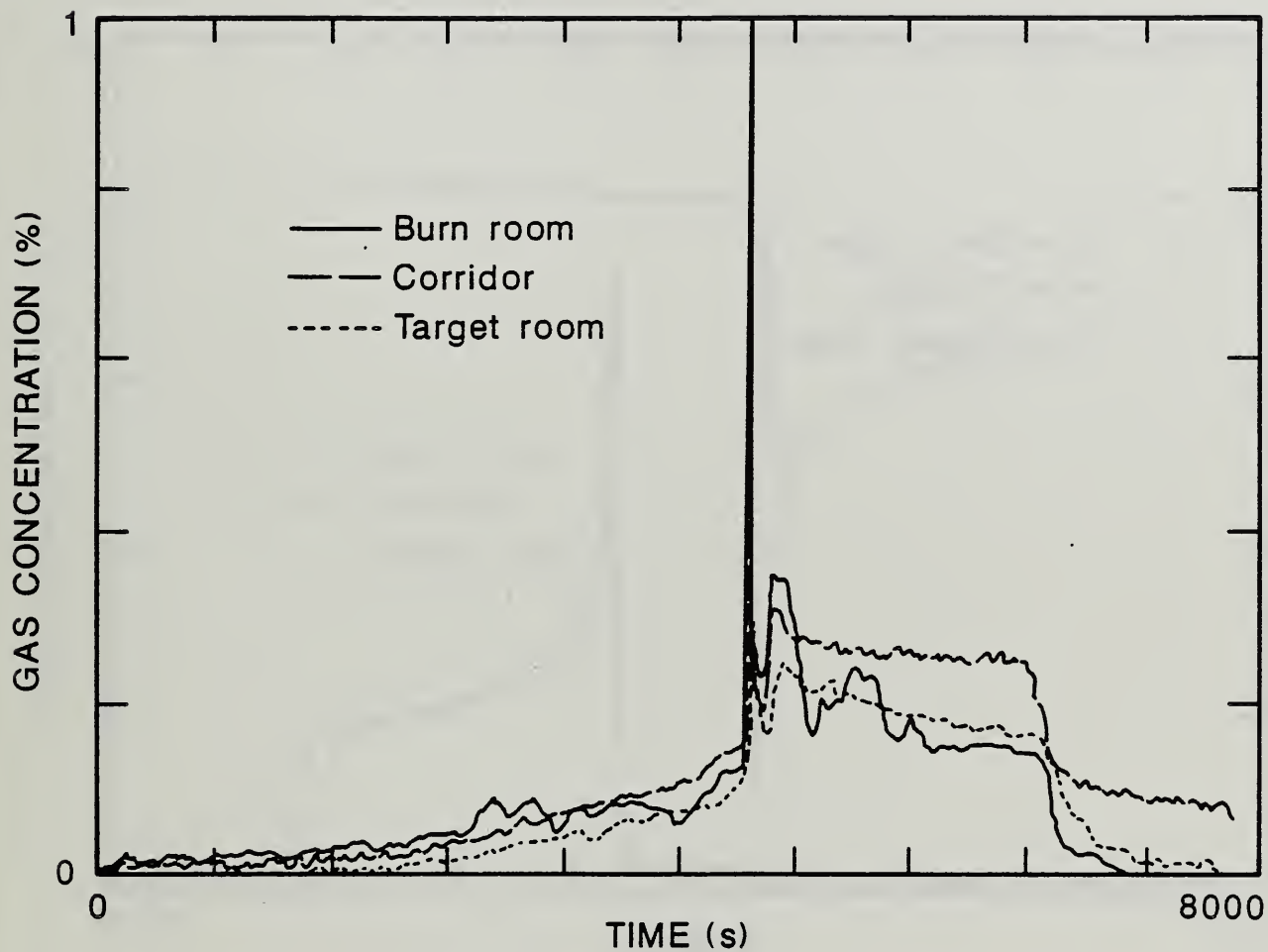
Figure 71. Comparison of Carbon Monoxide Concentrations in Each Compartment of the Large-Scale Test Facility for the Two-Cigarette Test of Foam 32 Mock-up Upholstery Chair Assembly With the Animal Exposure Chamber Connected to the Target Room.
