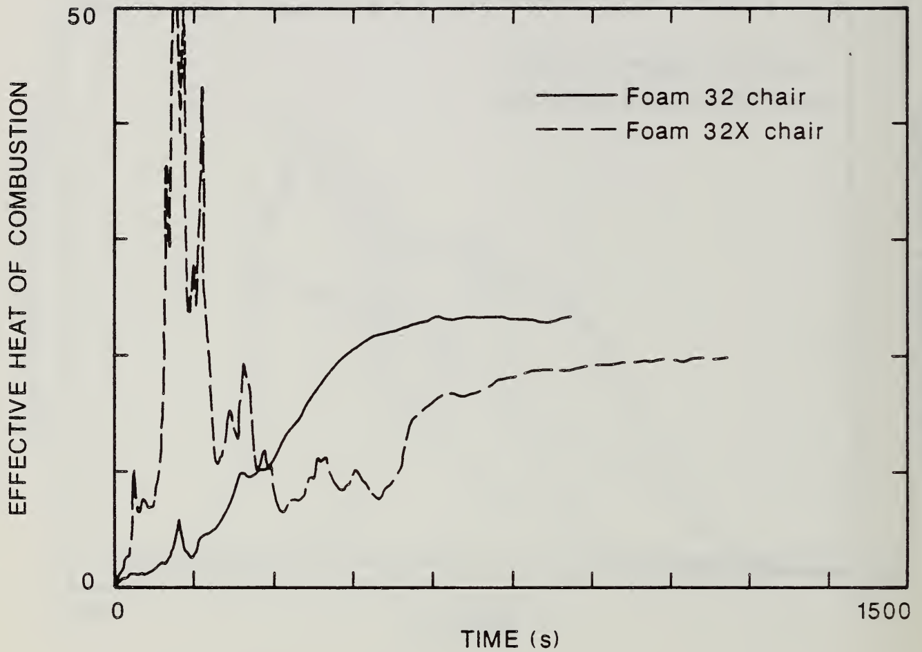
Figure 24. Comparison of the Effective Heat of Combustion from the Flaming Ignition of Foams 32 and 32X Mock-up Upholstery Chairs Tested in the Furniture Calorimeter.
