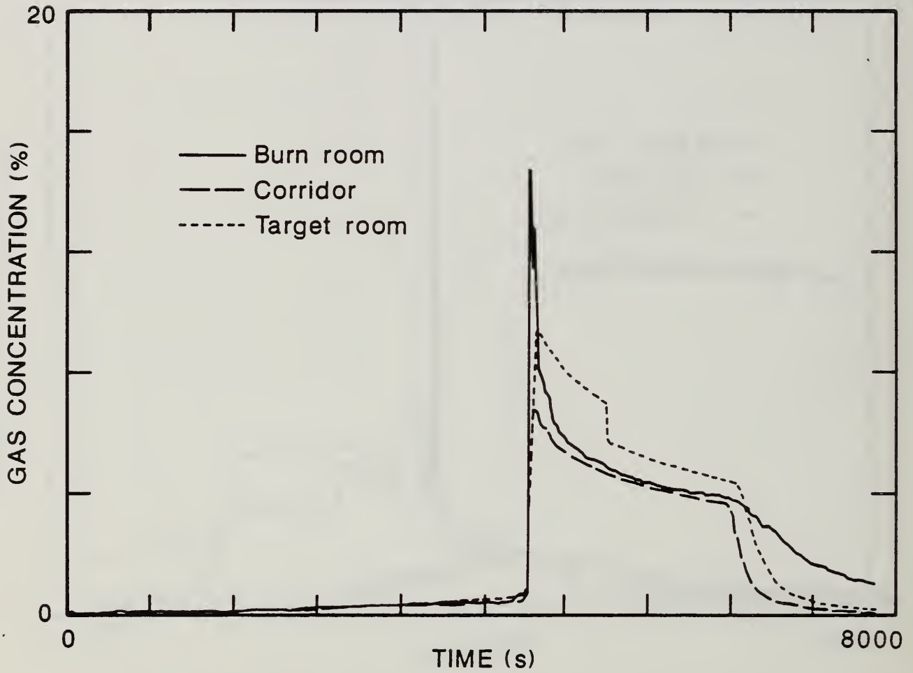
Figure 72. Comparison of Carbon Dioxide Concentration in Each Compartment of the Large-Scale Test Facility for the Two-Cigarette Test of Foam 32 Mock-up Upholstery Chair Assembly With the Animal Exposure Chamber Connected to the Target Room.
