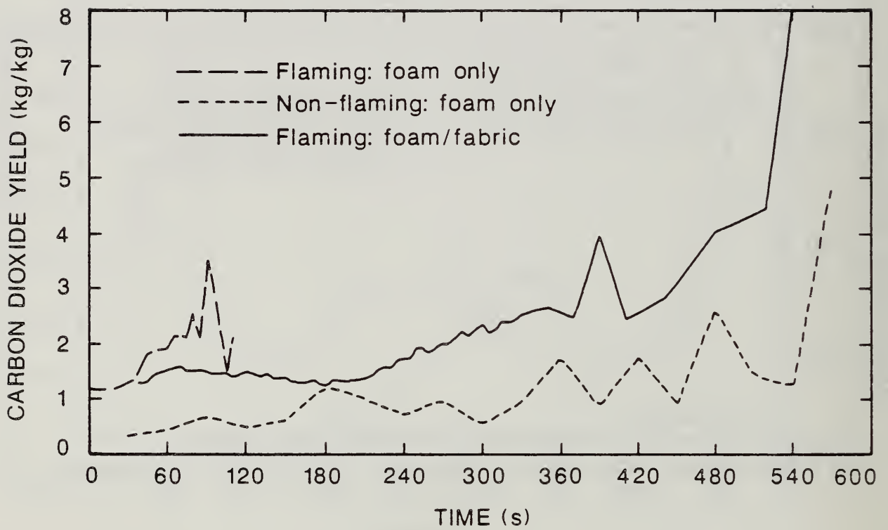
Figure 12. Comparison of Carbon Dioxide Yield for Foam 32X Flaming and Non-flaming Exposures Without a Cover Fabric and Flaming Exposures With a Cover Fabric.
