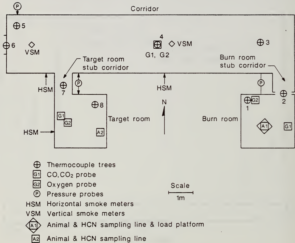
Figure 40. Schematic Floor Plan of The Large-Scale Three Compartment Test Facility.
