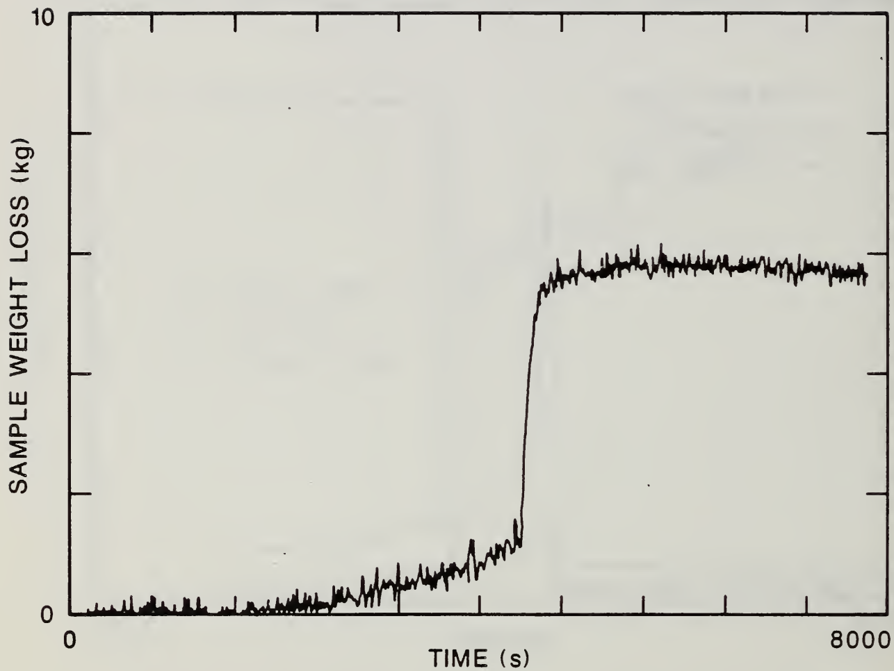
Figure 70. Mass Loss of Upholstery Chair Assembly Made from Foam 32 and Exposed to Two-Cigarettes in the Large-Scale Test Facility With the Animal Exposure Chambers Connected to the Target Room.
