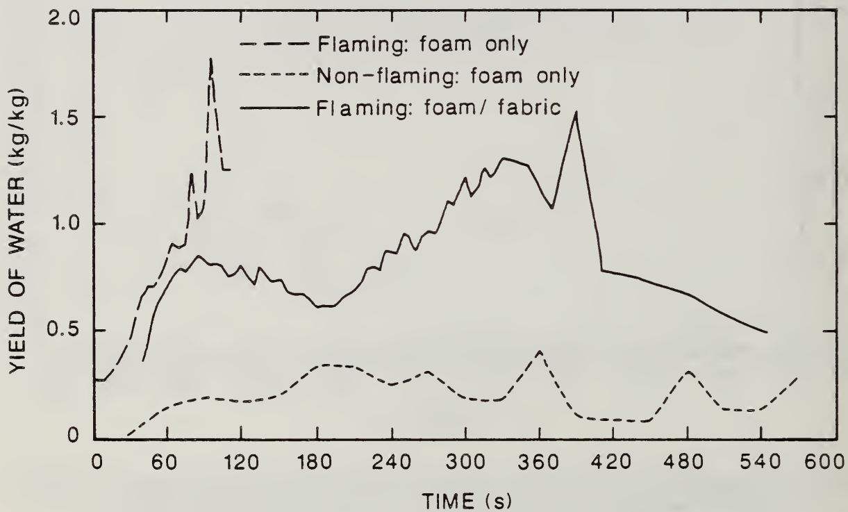
Figure 14. Comparison of Water Yield for Foam 32X Flaming and Non-flaming Exposures Without a Cover Fabric and Flaming Exposure With a Cover Fabric.
