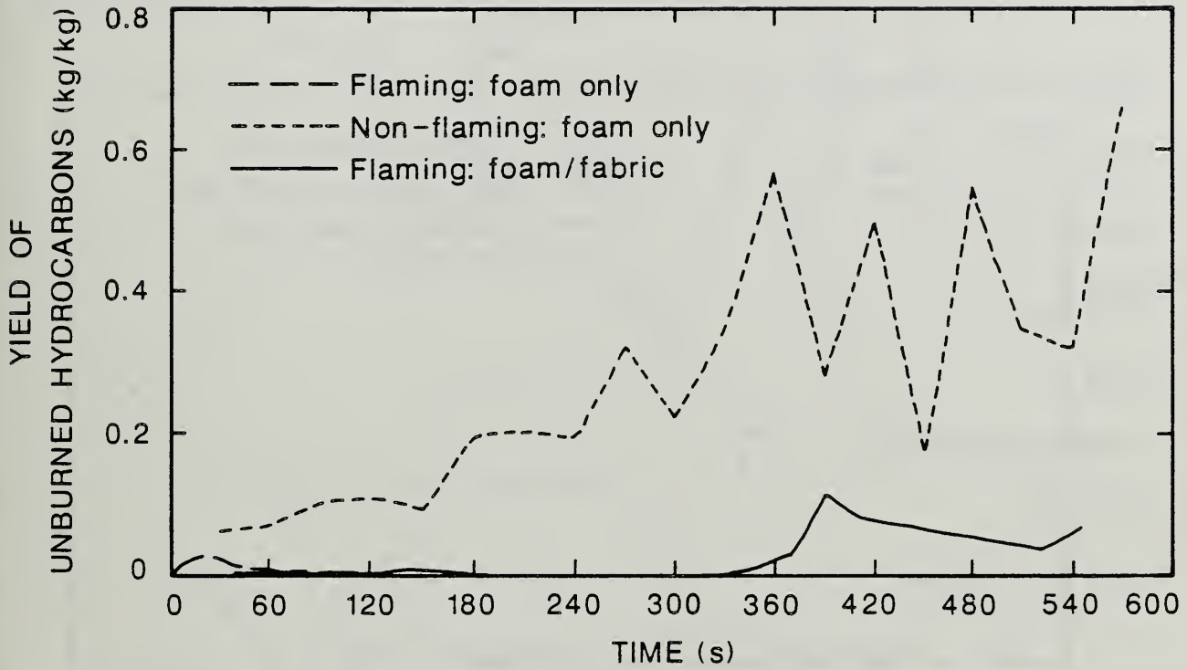
Figure 15. Comparison of Unburned Hydrocarbon Yield for Foam 32X Flaming and Non-flaming Exposures Without a Cover Fabric and Flaming Exposure With a Cover Fabric.
