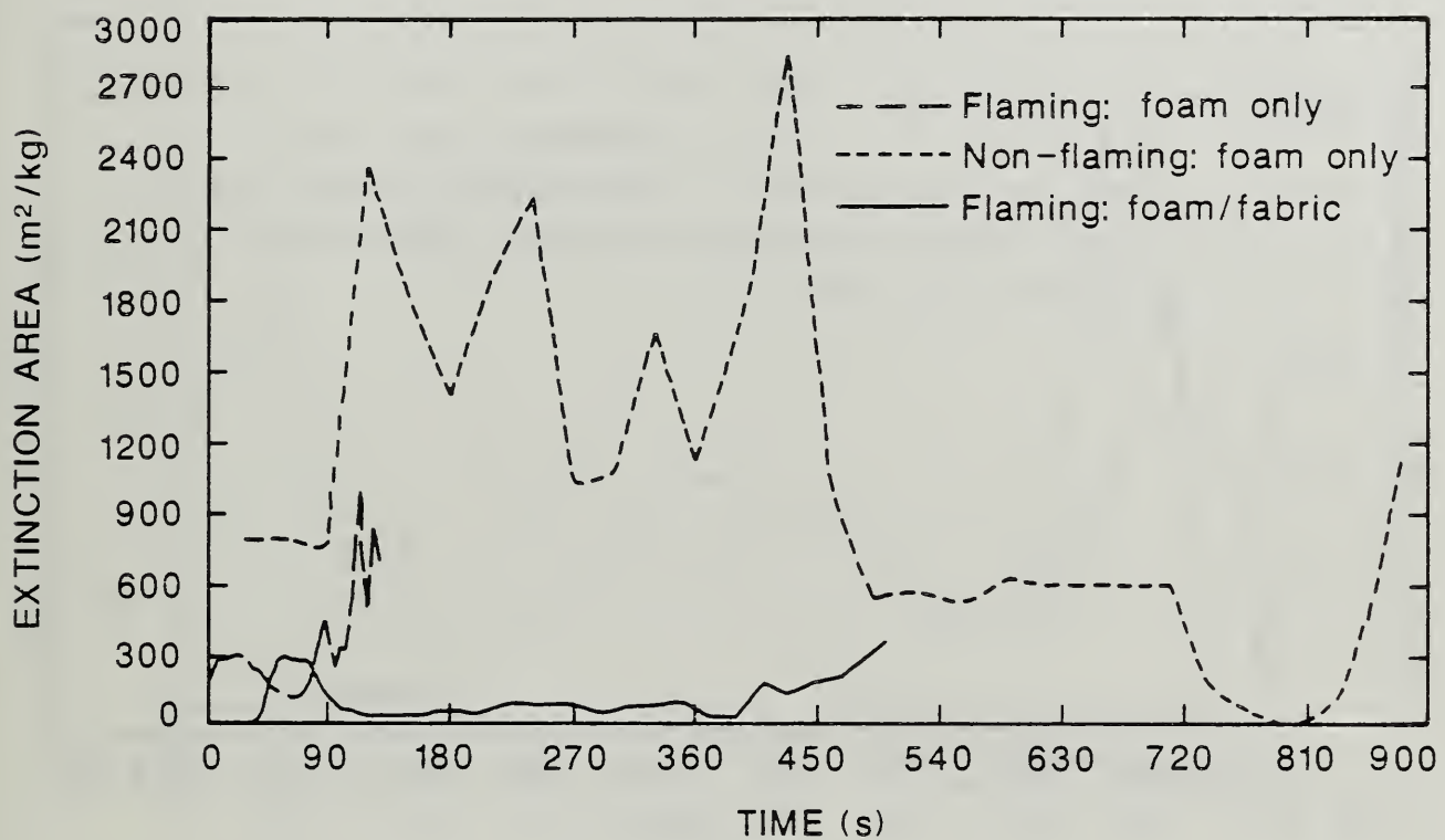
Figure 9. Comparison of Smoke Extinction Area for Foam 32 Flaming and Non-flaming Exposures Without a Cover Fabric and Flaming Exposure With a Cover Fabric..
