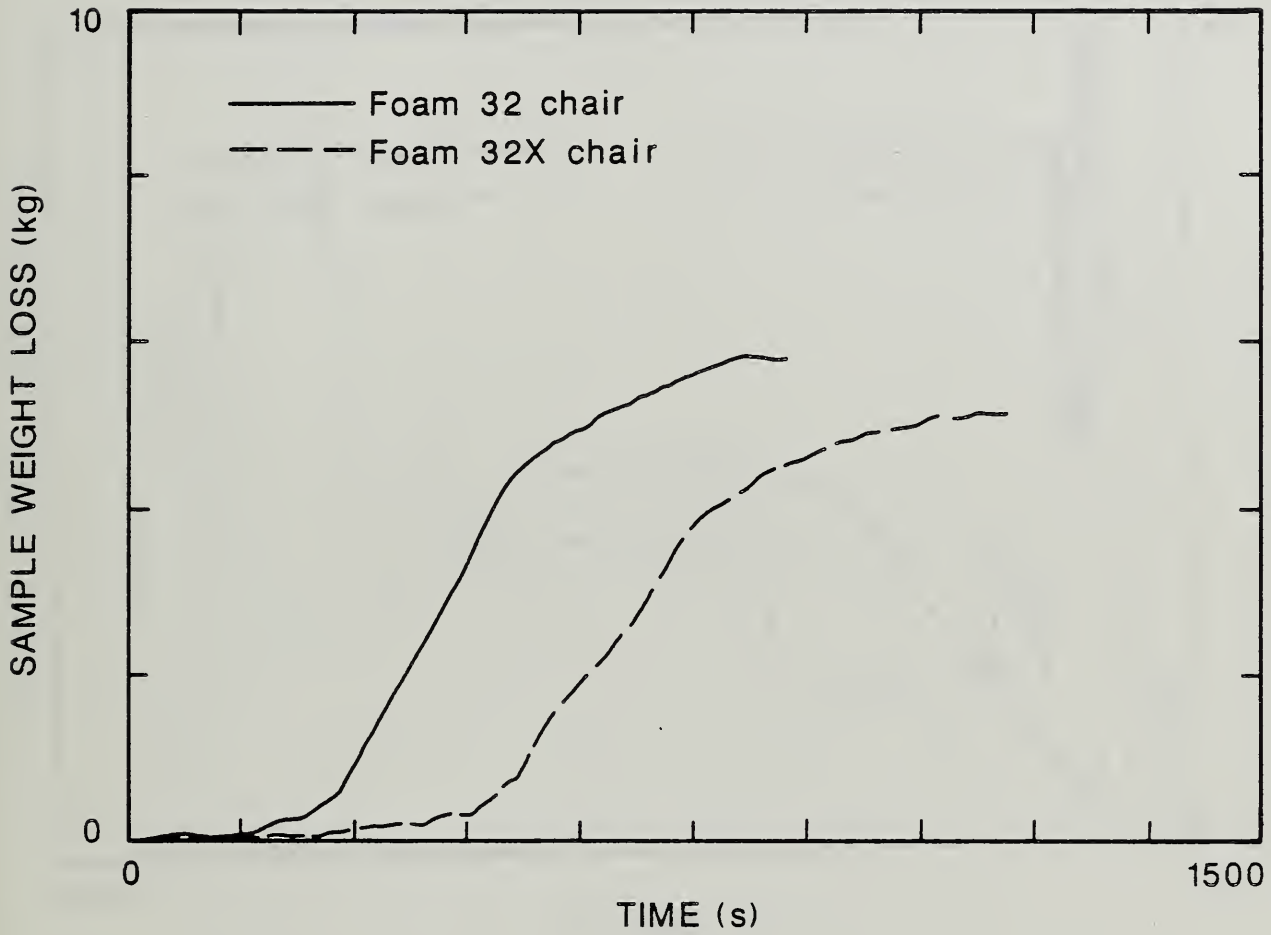
Figure 23. Comparison of Sample Weight Loss During Flaming Ignition of Foams 32 and 32X in the Furniture Calorimeter.
