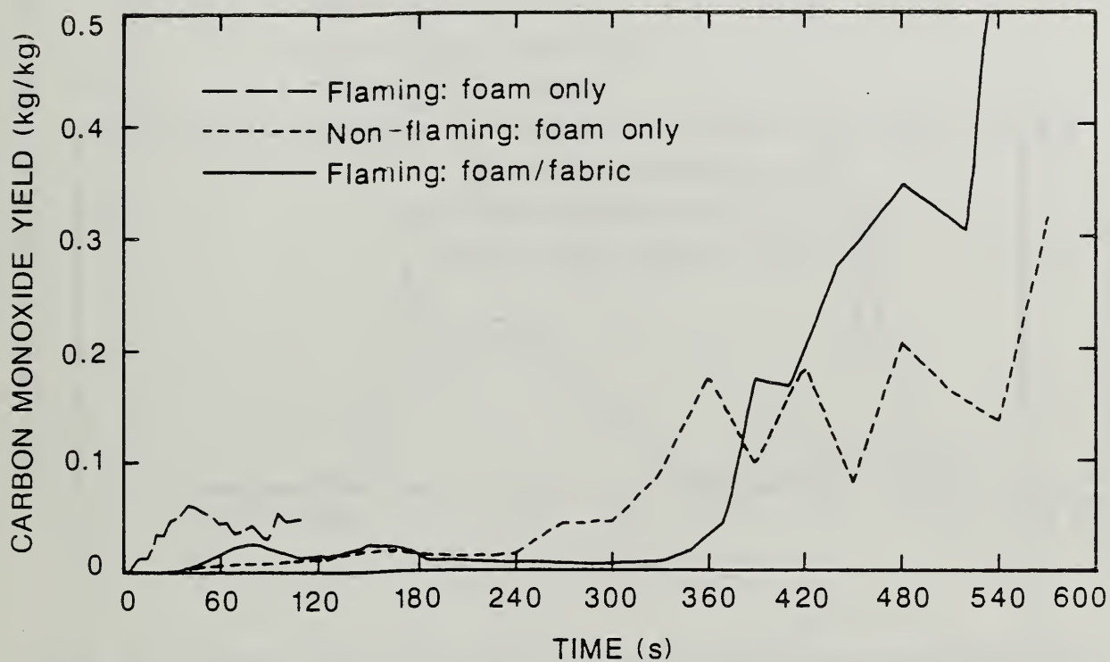
Figure 13. Comparison of Carbon Monoxide Yield for Foam 32X Flaming and Non-flaming Exposures Without a Cover Fabric and Flaming Exposure With a Cover Fabric.
