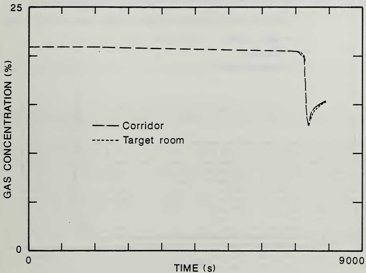
Figure 83. Comparison of Oxygen Concentrations in Each Compartment of the Large-Scale Test Facility for the Two-Cigarette Test of Foam 32X Mock-up Upholstery Chair Assembly With the Animal Exposure Chambers Connected to the Target Room.
