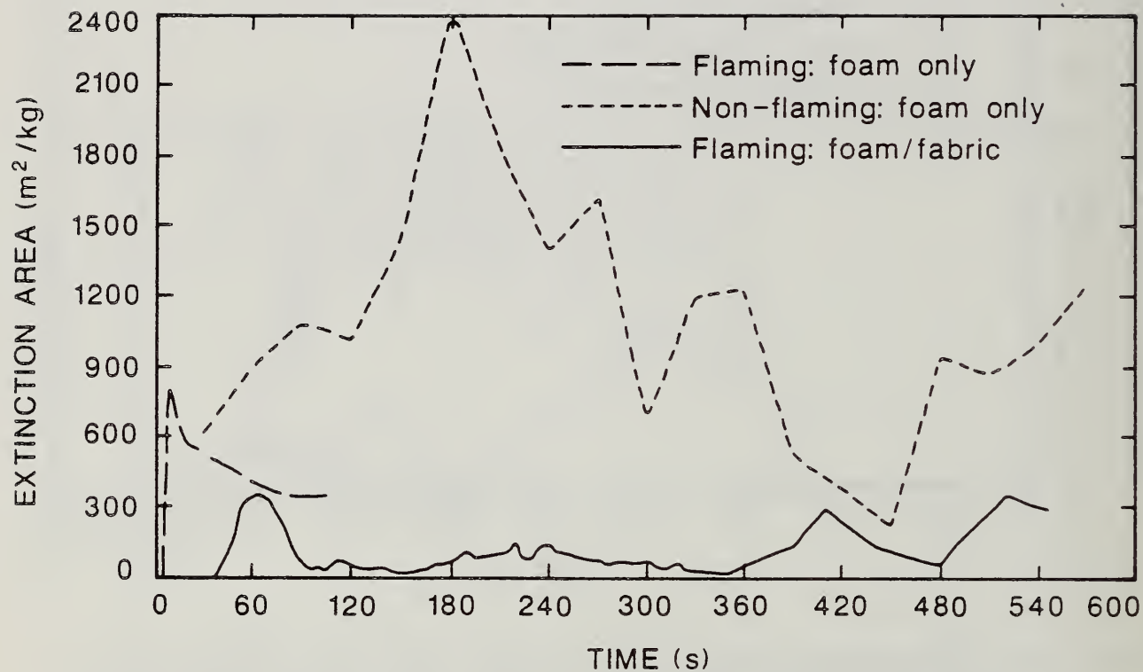
Figure 16. Comparison of Smoke Extinction Area for Foam 32X Flaming and Non-flaming Exposures Without a Cover Fabric and Flaming Exposure with a Cover Fabric.
