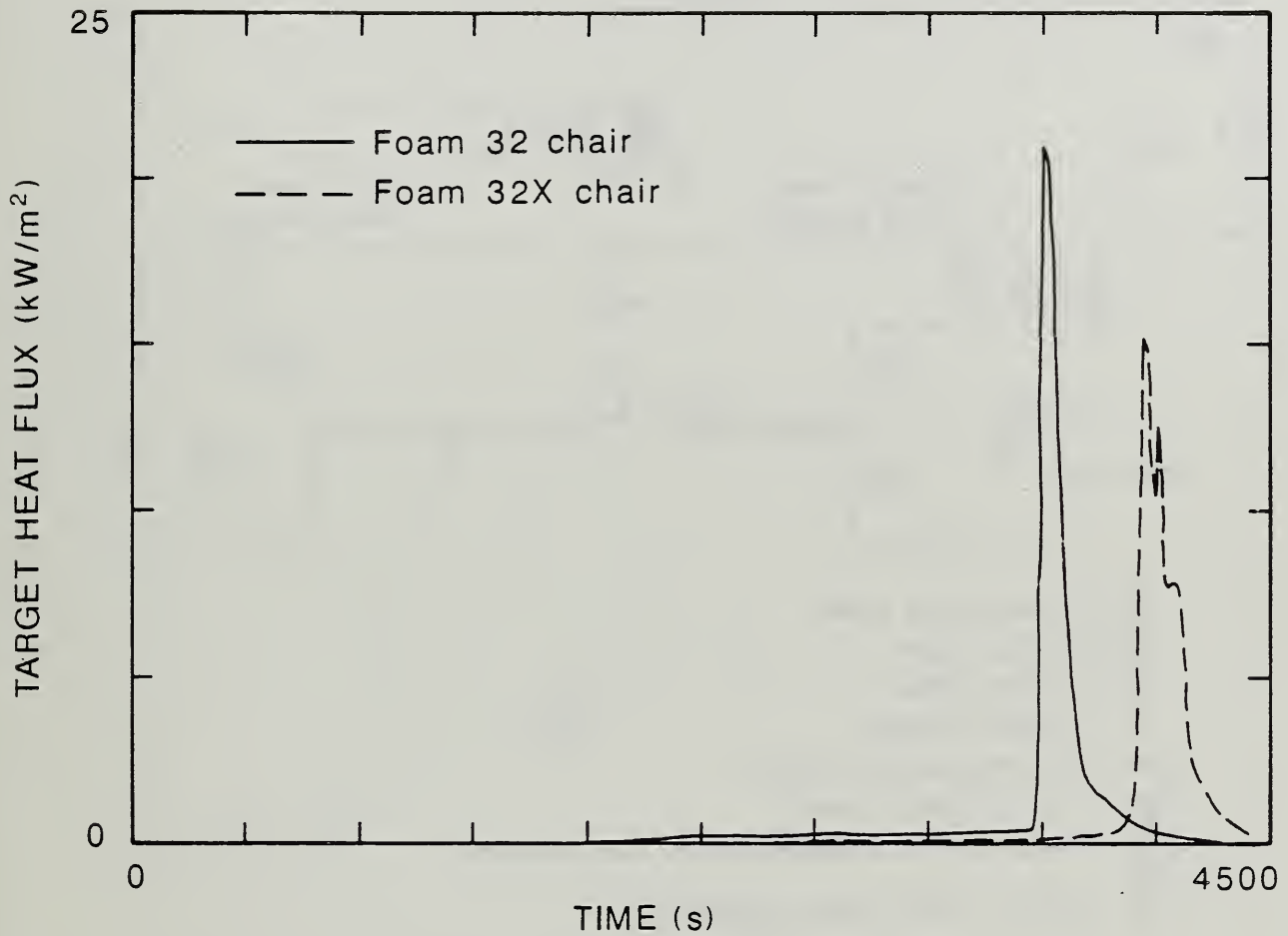
Figure 39. Comparison of the Heat Flux Received by a Target Material from the Smoldering-to-Flaming Ignitions of Foams 32 and 32X Upholstery Chair Mock-ups Tested in the Furniture Calorimeter..
