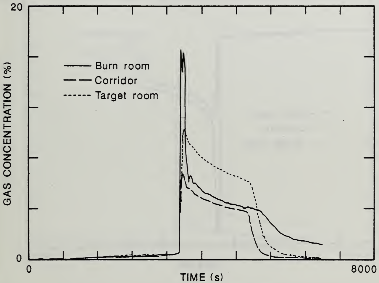
Figure 67. Comparison of Carbon Dioxide Concentrations in Each Compartment of the Large-Scale Test Facility for the Two-Cigarette Test of Foam 32 Mock-up Upholstery Chair Assembly With the Animal Exposure Chambers Connected to the Burn Room.
