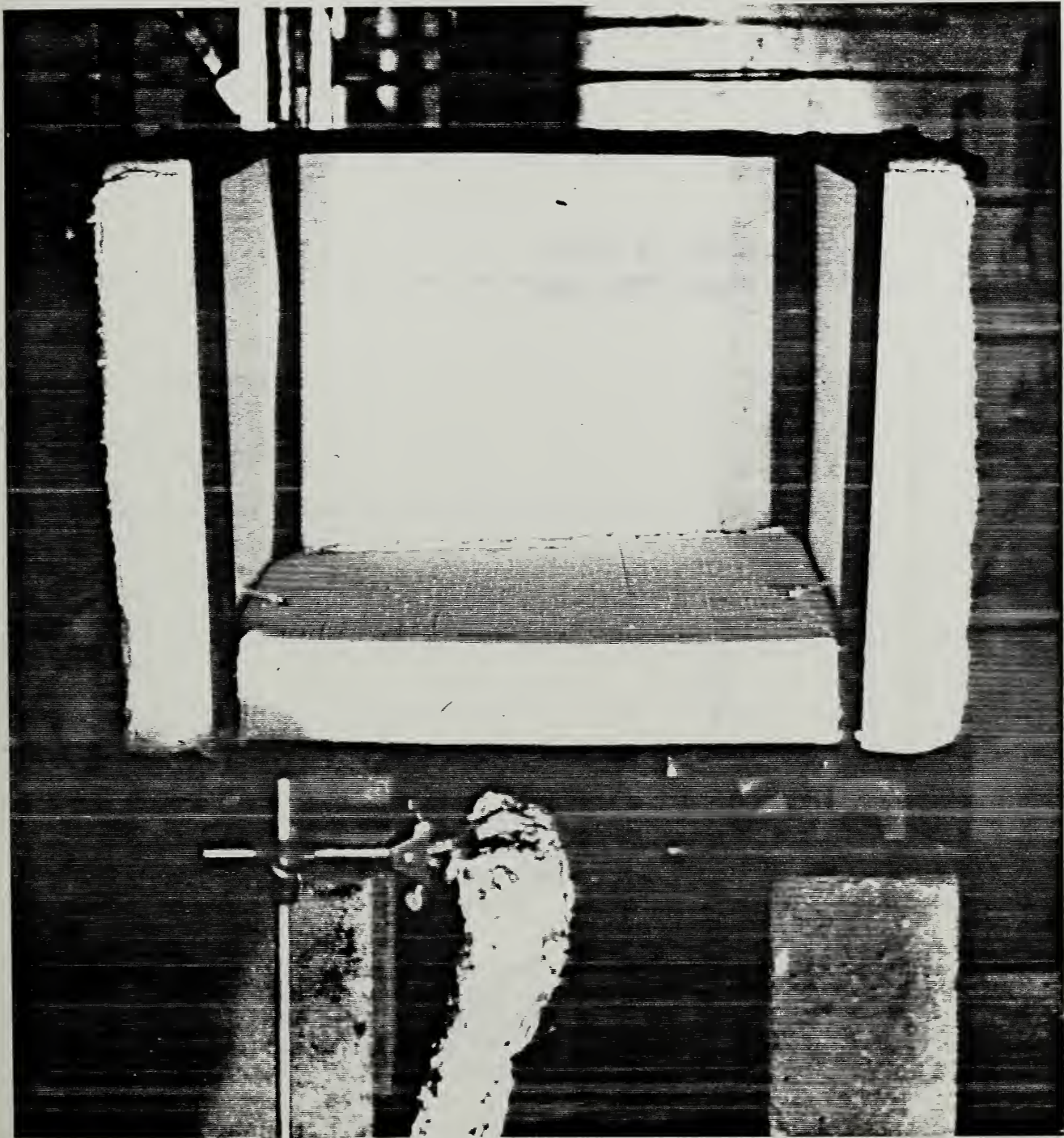
Figure 29. Upholstery Chair Mock-up with Two Smoldering Cigarettes as Tested in the Furniture Calorimeter.
