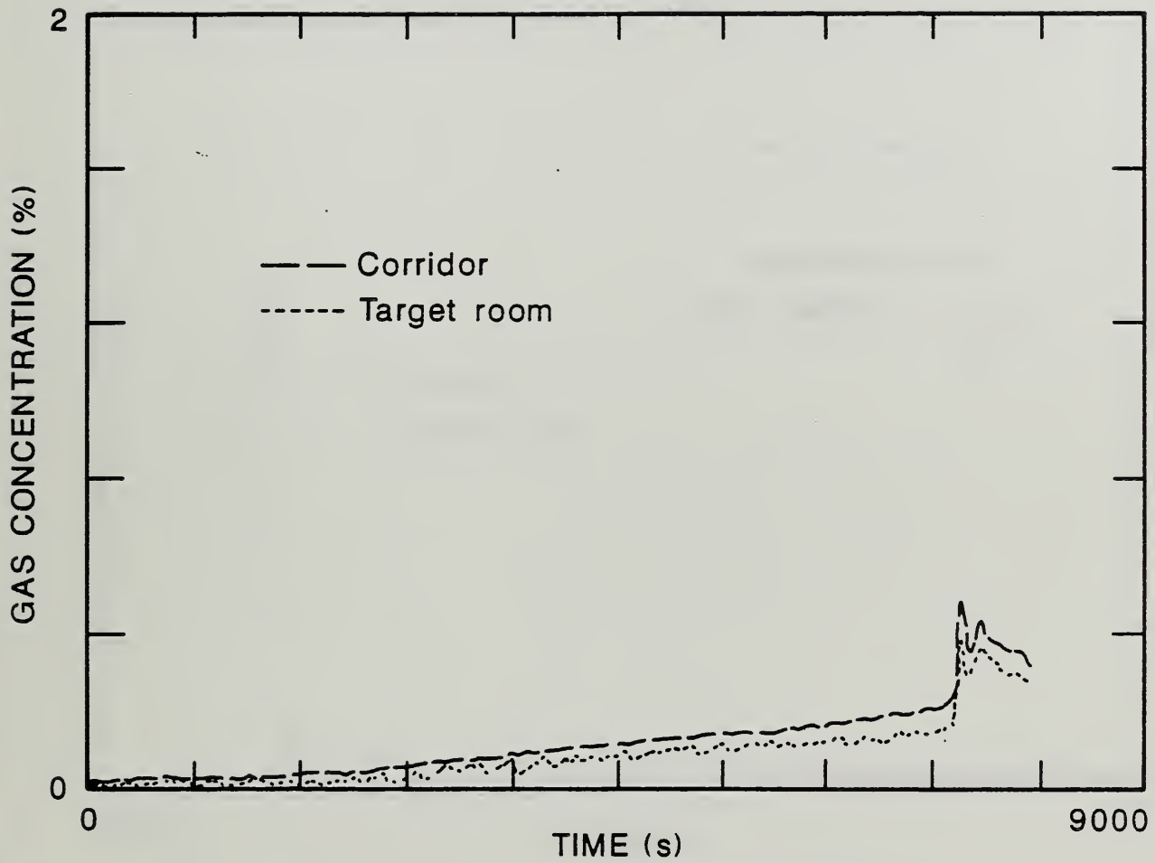
Figure 81. Comparison of Carbon Monoxide Concentrations in Each Compartment of the Large-Scale Test Facility for the Two-Cigarette Test of Foam 32X Mock-up Upholstery Chair Assembly With the Animal Exposure Chambers Connected to the Target Room.
