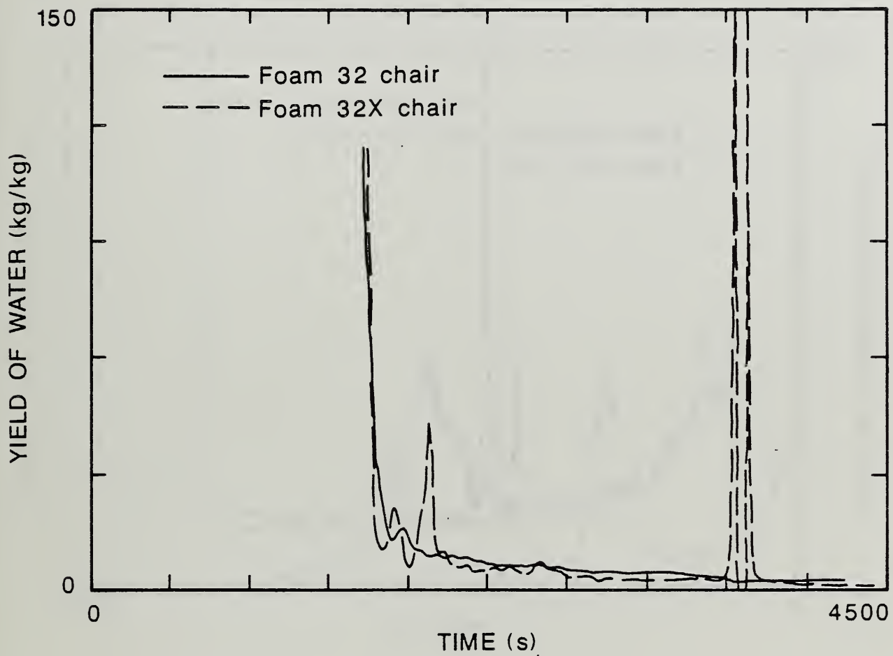
Figure 35. Comparison of the Yield of Water from Smoldering-to-Flaming Ignitions of Foams 32 and 32X Upholstery Chair Mock-ups Tested in the Furniture Calorimeter (excluding early smoldering because of erratic response).
