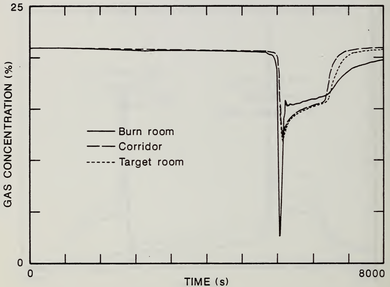
Figure 78. Comparison of Oxygen Concentrations in Each Compartment of the Large-Scale Test Facility for the Two-Cigarette Test of Foam 32X Mock-up Upholstery Chair Assembly With the Animal Exposure Chambers Connected to the Burn Room.
