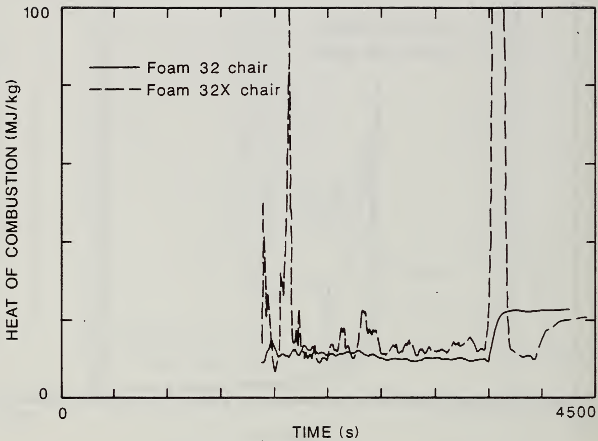
Figure 36. Comparison of The Heat of Combustion from the Smoldering-to-Flaming Ignitions of Foams 32 and 32X Upholstery Chair Mock-ups Tested in the Furniture Calorimeter (excluding early smoldering because of erratic response).
