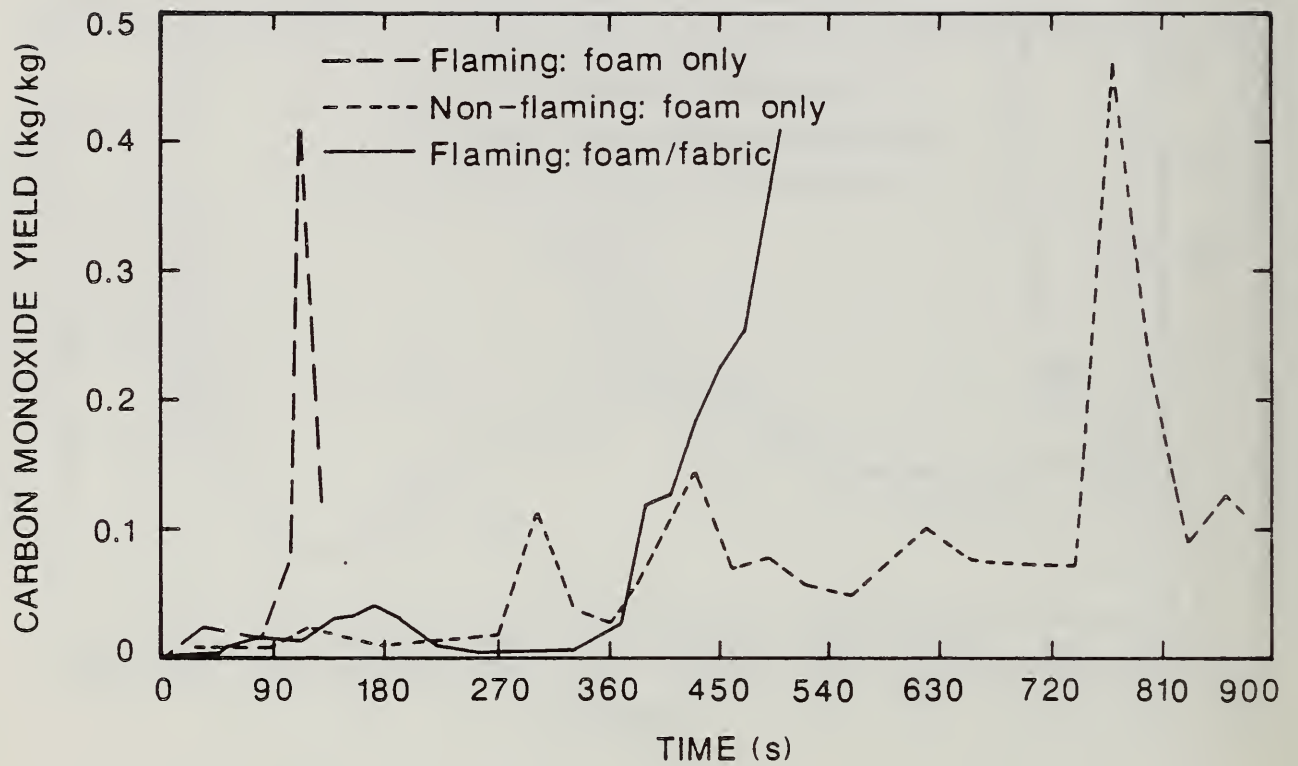
Figure 6. Comparison of Carbon Monoxide Yield for Foam 32 Flaming and Non-flaming Exposures Without a Cover Fabric and Flaming Exposure With a Cover Fabric.
