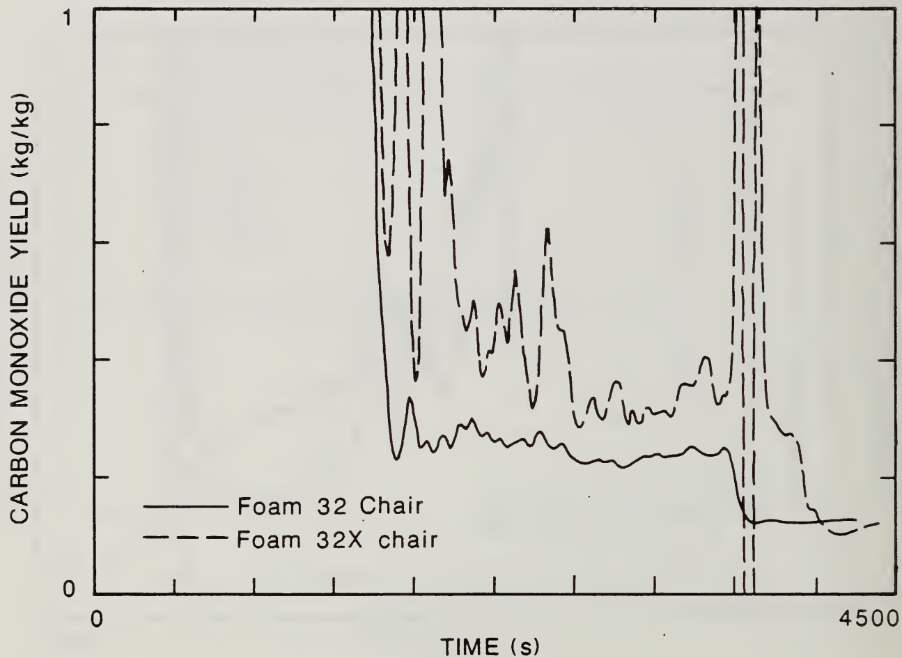
Figure 34. Comparison of Carbon Monoxide Yields for Smoldering-to-Flaming Ignitions of Foams 32 and 32X Upholstery Chair Mock-ups Tested in the Furniture Calorimeter (excluding early smoldering because of erratic response).
