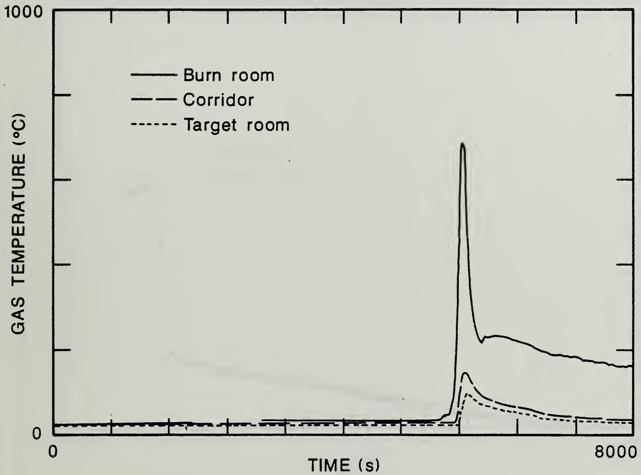
Figure 79. Comparison of Upper Compartment Gas Temperatures in Each Compartment of the Large-Scale Test Facility for the Two Cigarette Test of Foam 32X Mock-up Upholstery Chair Assembly With the Animal Exposure Chambers Connected to the Burn Room.
