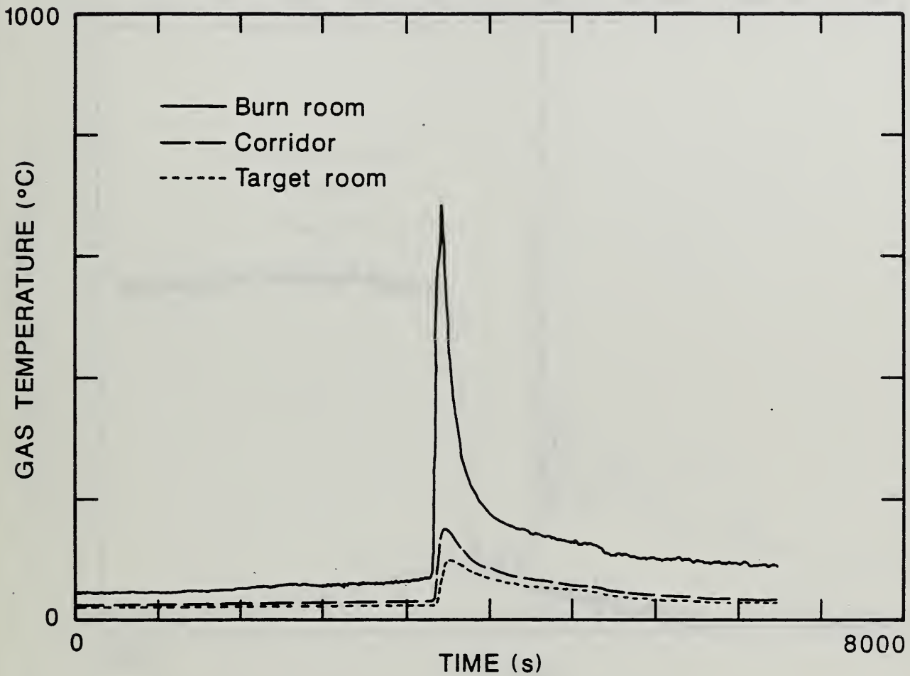
Figure 69. Comparison of the Upper Compartment Gas Temperature in Each Compartment of the Large-Scale Test Facility for the Two Cigarette Test of Foam 32 Mock-up Upholstery Chair Assembly With the Animal Exposure Chambers Connected to the Burn Room.
