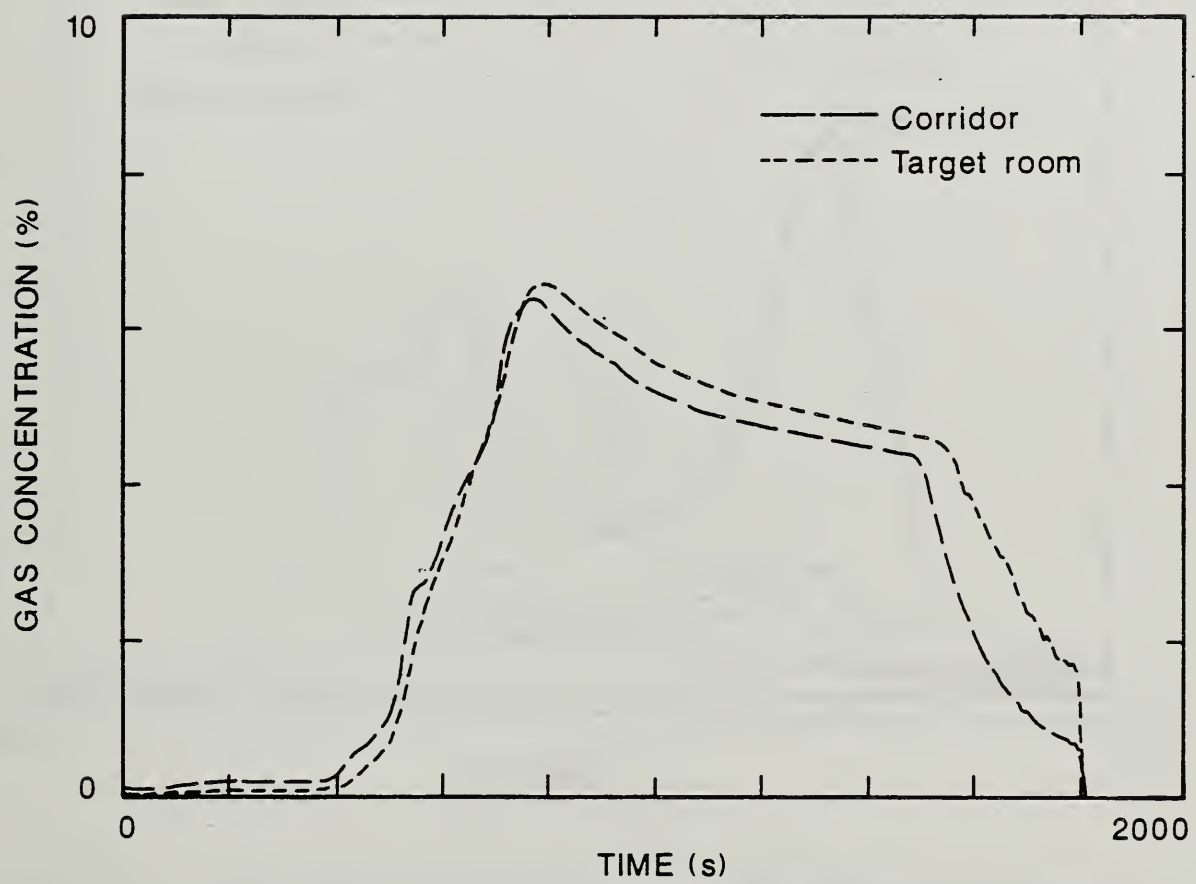
Figure 45. Carbon Dioxide Concentration in Each Compartment of the Large-Scale Facility During Flaming Ignition Test of Foam 32X Mock-up Upholstery Chair Assembly.
