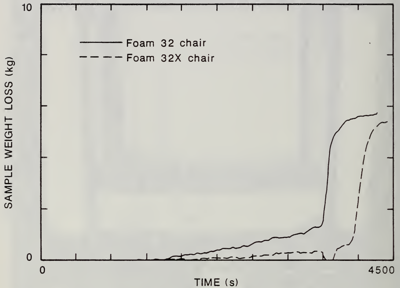
Figure 30. Comparison of Sample Weight Loss During Smoldering-to-Flaming Ignition of Mock-up Upholstery Chairs Made from Foams 32 and 32X Tested in the Furniture Calorimeter.
