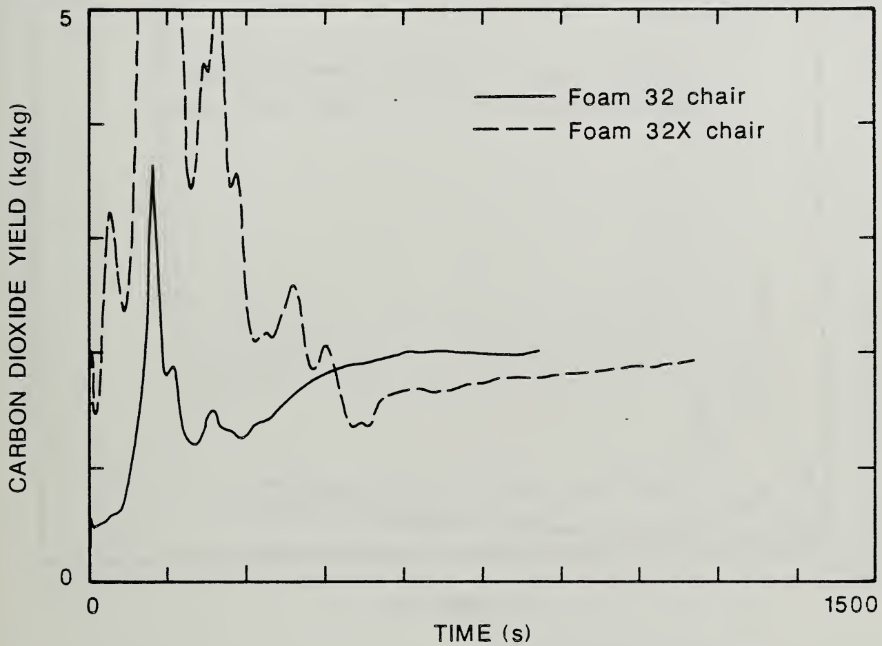
Figure 25. Comparison of Carbon Dioxide Yield for the Flaming Ignition of Foams 32 and 32X Mock-up Upholstery Chairs Tested in the Furniture Calorimeter.
