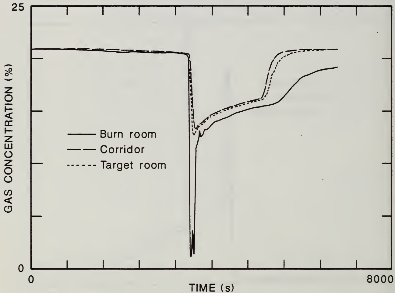
Figure 68. Comparison of Oxygen Concentrations in Each Compartment of the Large-Scale Test Facility for the Two-Cigarette Test of Foam 32 Mock-up Upholstery Chair Assembly With the Animal Exposure Chambers Connected to the Burn Room.
