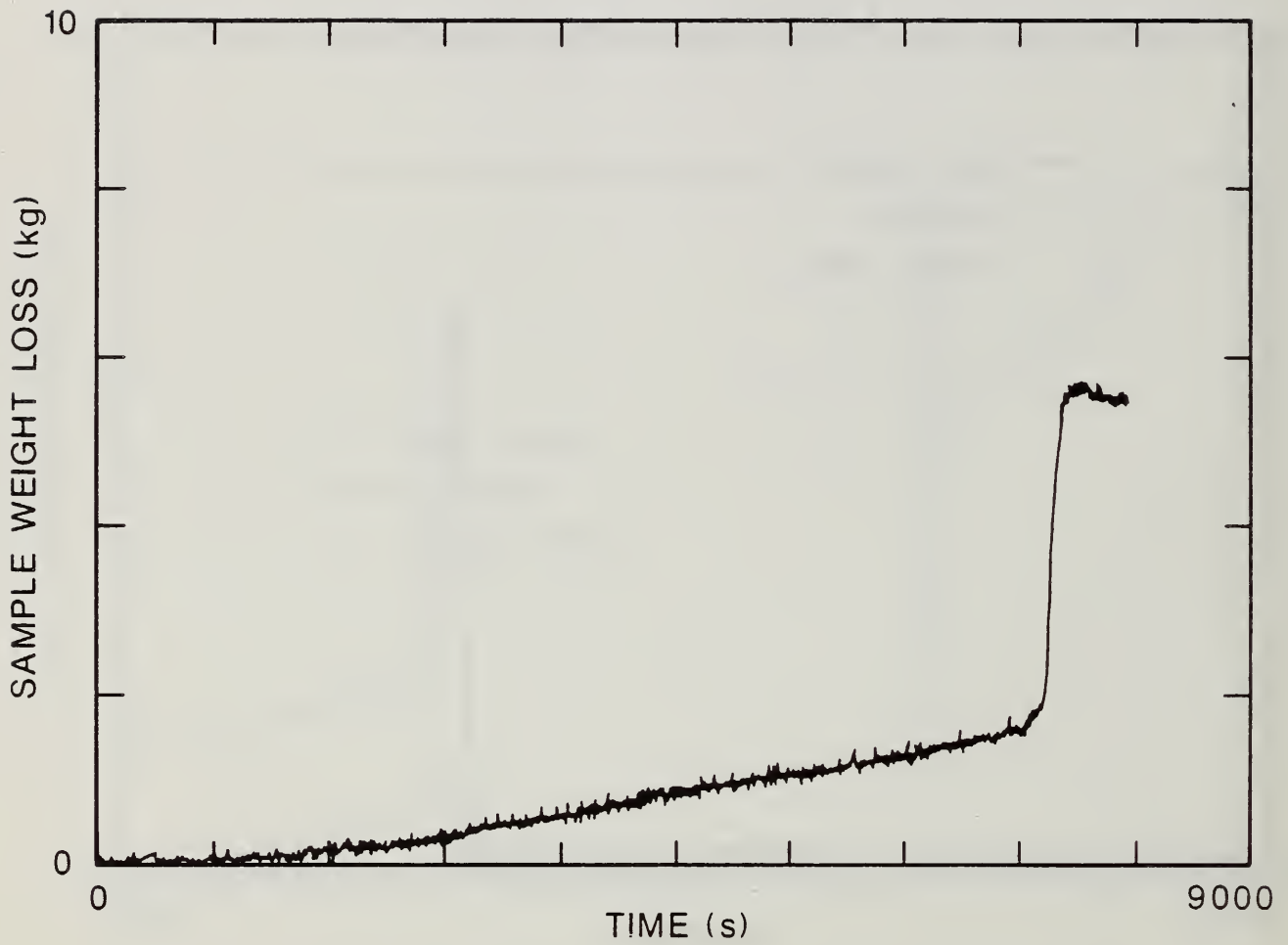
Figure 80. Mass Loss of Upholstery Chair Assembly Made from Foam 32X and Exposed to Two-Cigarettes in the Large-Scale Test Facility With the Animal Exposure Chambers Connected to the Target Room.
