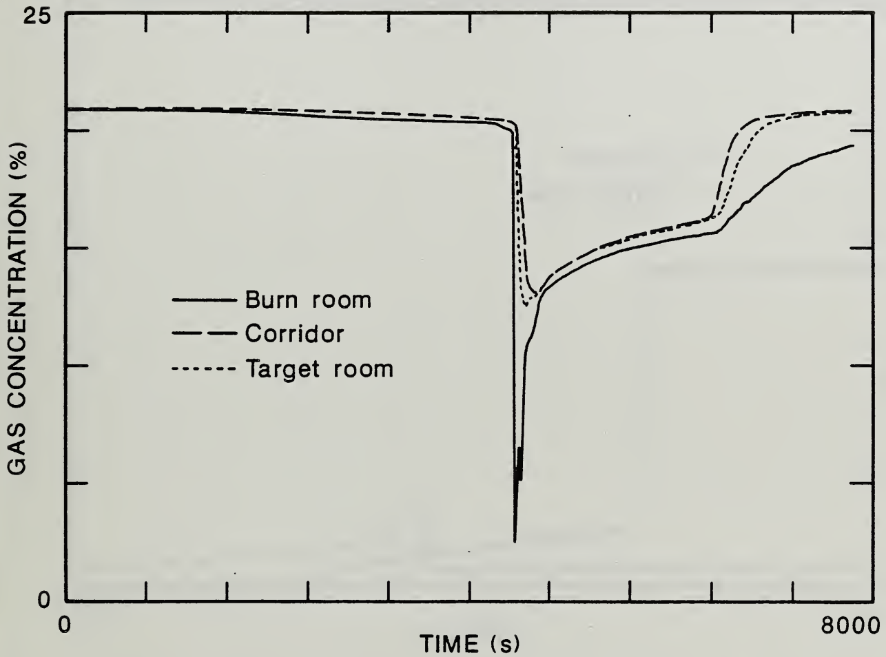
Figure 73. Comparison of Oxygen Concentration in Each Compartment of the Large-Scale Test Facility for the Two-Cigarette Test of Foam 32 Mock-up Upholstery Chair Assembly With the Animal Exposure Chamber Connected to the Target Room.
