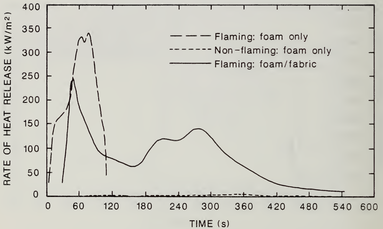
Figure 10. Comparison of Heat Release Rate for Foam 32X Flaming and Non-flaming Exposures Without a Cover Fabric and Flaming Exposure With a Cover Fabric.
