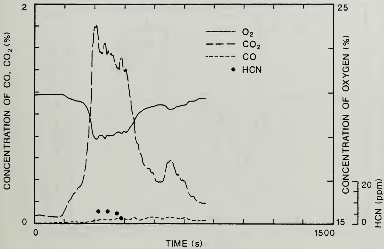
Figure 19. Furniture Calorimeter Data for the Concentration of Carbon Dioxide, Carbon Monoxide, HCN, and Oxygen for the Flaming Ignition of Mock-up Chairs made with Foam 32.
