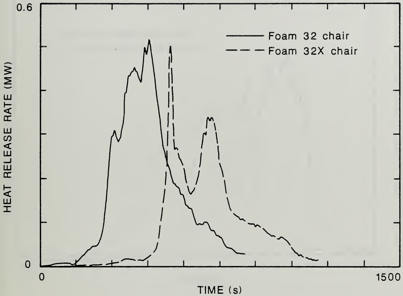
Figure 21. Furniture Calorimeter Data Comparing the Rate of Heat Release from the Flaming Ignition of Mock-up Chairs Made from Either Foam 32 and Foam 32X.
