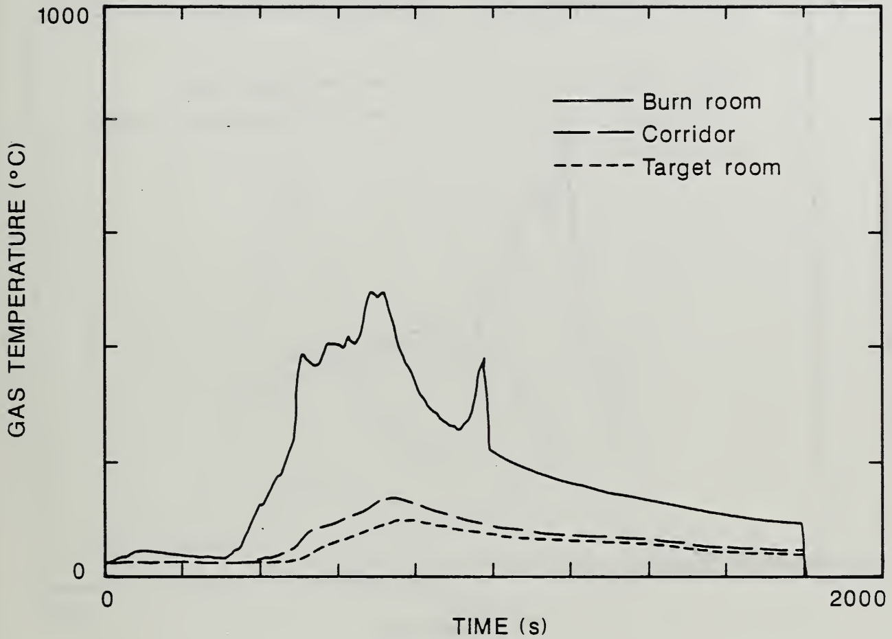
Figure 47. Upper Layer Gas Temperatures in Each Compartment of the Large-Scale Facility During Flaming Ignition test of Foam 32 Mock-up Upholstery Chair Assembly.
