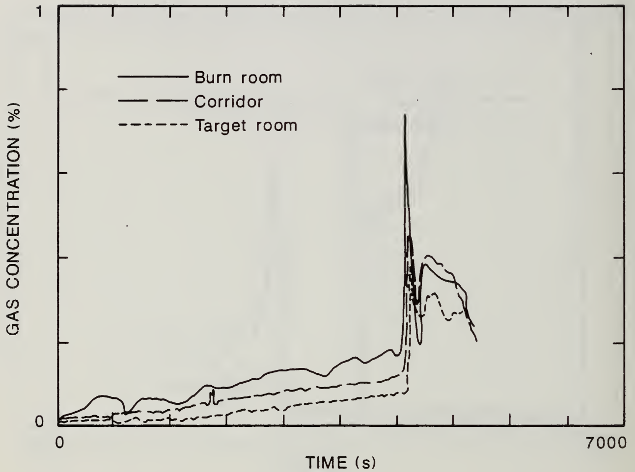
Figure 60. Comparison of Carbon Monoxide Concentrations in Each Compartment of the Large-Scale Test Facility for the Two-Cigarette Test of Foam 32X Mock-up Upholstery Chair Assembly.
