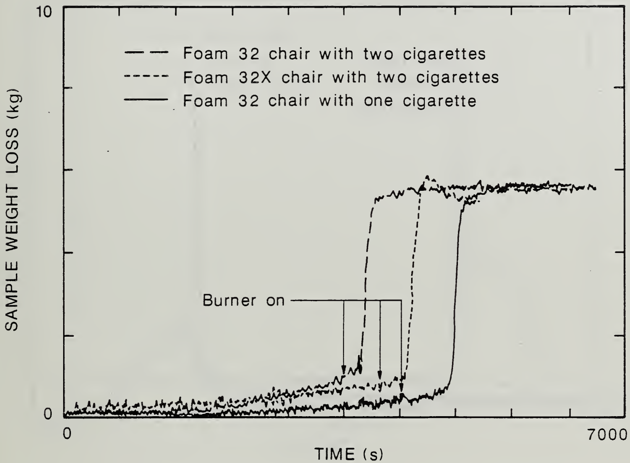
Figure 51. Comparison of Weight Loss for Preliminary Smoldering-to-Flaming Experiments of Foams 32 and 32X Mock-up Upholstery Chair Assemblies.
