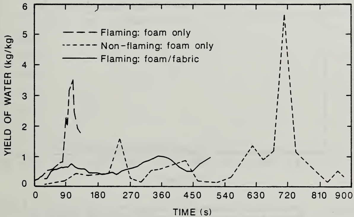
Figure 7. Comparison of Water Yield for Foam 32 Flaming and Non-flaming Exposures Without a Cover Fabric and Flaming Exposure With a Cover Fabric.
