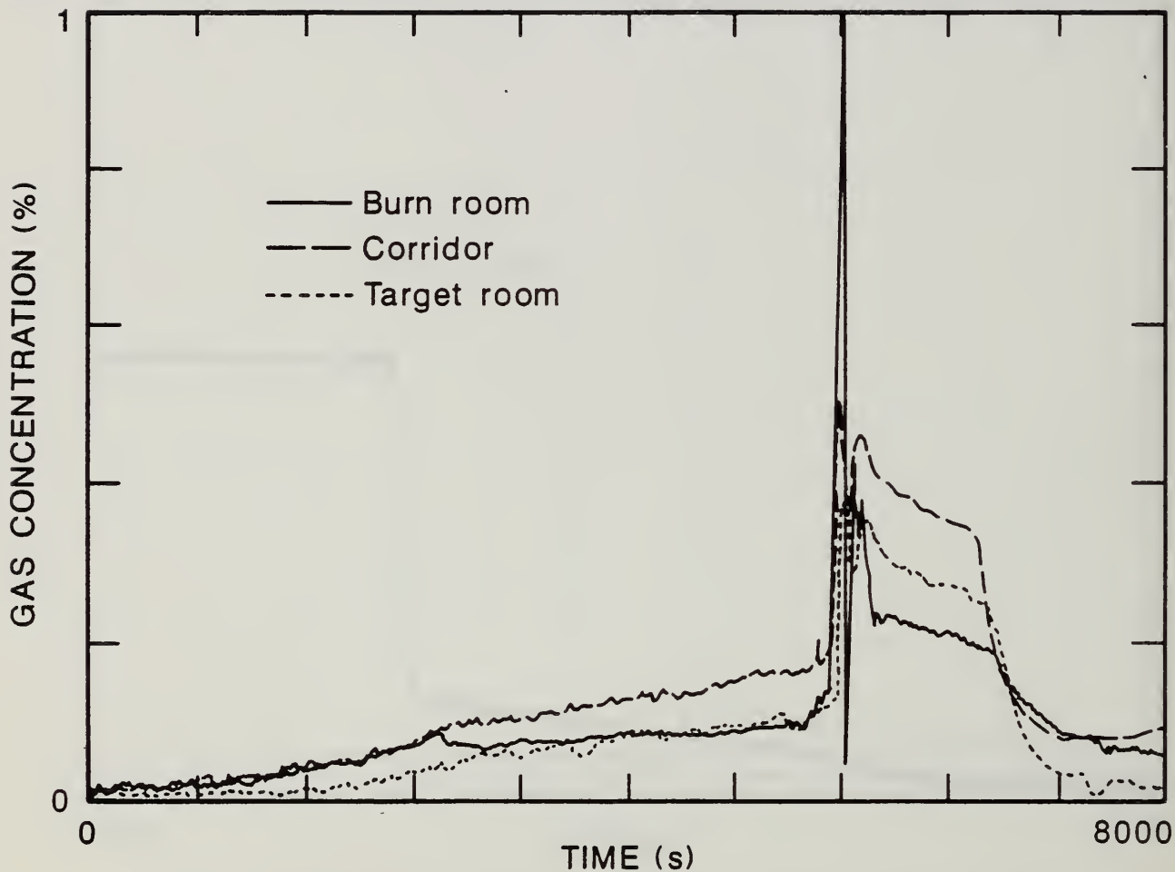
Figure 76. Comparison of Carbon Monoxide Concentrations in Each Compartment of the Large-Scale Test Facility for the Two-Cigarette Test of Foam 32X Mock-up Upholstery Chair Assembly With the Animal Exposure Chambers Connected to the Burn Room.
