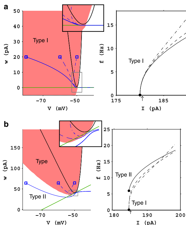
Fig. 2 The Type of f-I curve depends on the point of reset. a When a = 0 only type I f-I curves are possible. The phase plane at a current just above rheobase ( I = I_{SN} + 0.5 pA) shows that the trajectories are forced to pass through the ghost of the saddle-node bifurcation independently of the starting point (three steady-state trajectories are shown for three different values of V_r voltage reset). The frequency–current plot on the right shows the f-I curve corresponding to the three different reset conditions (consistent line types; full , dash or dot/dash ). b When a > 0 it is possible to have type I and type II depending on the reset. The region in pink shows the basin of attraction of the stable fixed point just before ( I = I_{SN} - 0.1 pA) the system loses stability via a saddle-node bifurcation. The resets at -50 and -60 mV result in trajectories that pass very near the two nullclines, and are therefore very slow. The reset at -80 mV is outside the ghost of the attraction basin so that its trajectory passes further away from the saddle-node bifurcation. The insets show the enlarged areas enclosed by the gray rectangles . The arrow on the I -axis of the f-I plot indicates the current that was used to draw nullclines and trajectories in the phase plane. The conventions for line colors is the same as in Fig. 1
