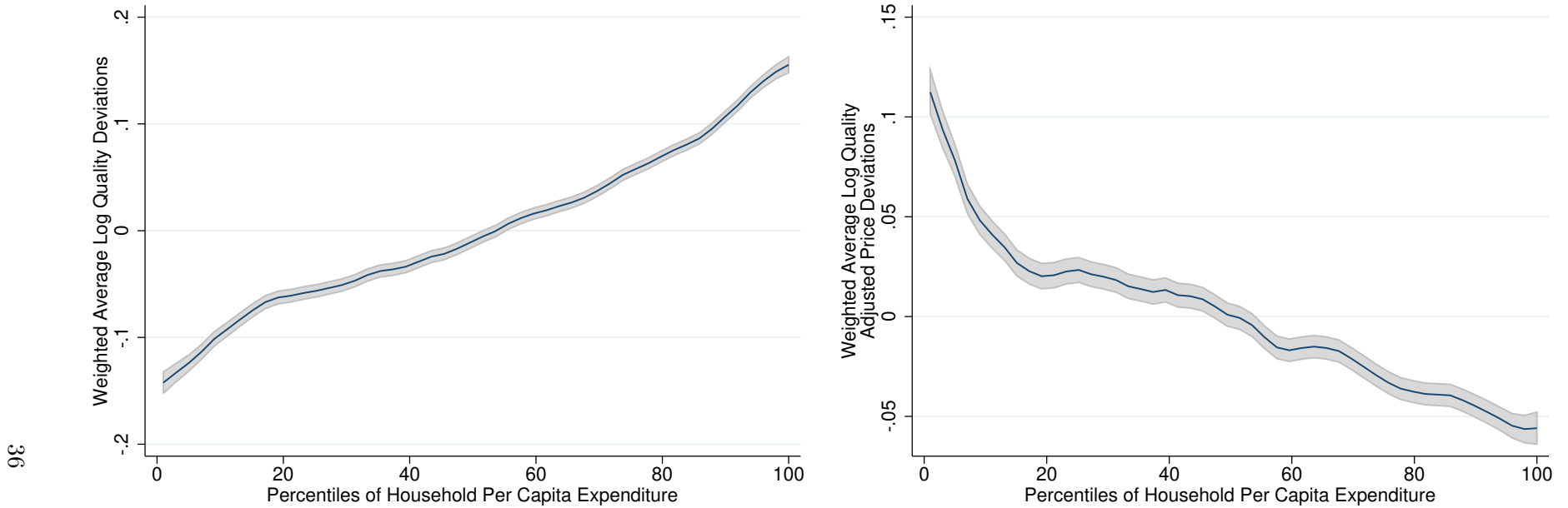
Figure 2: Distribution of Weighted Average Product Quality and Quality-Adjusted Prices across Consumption Baskets
