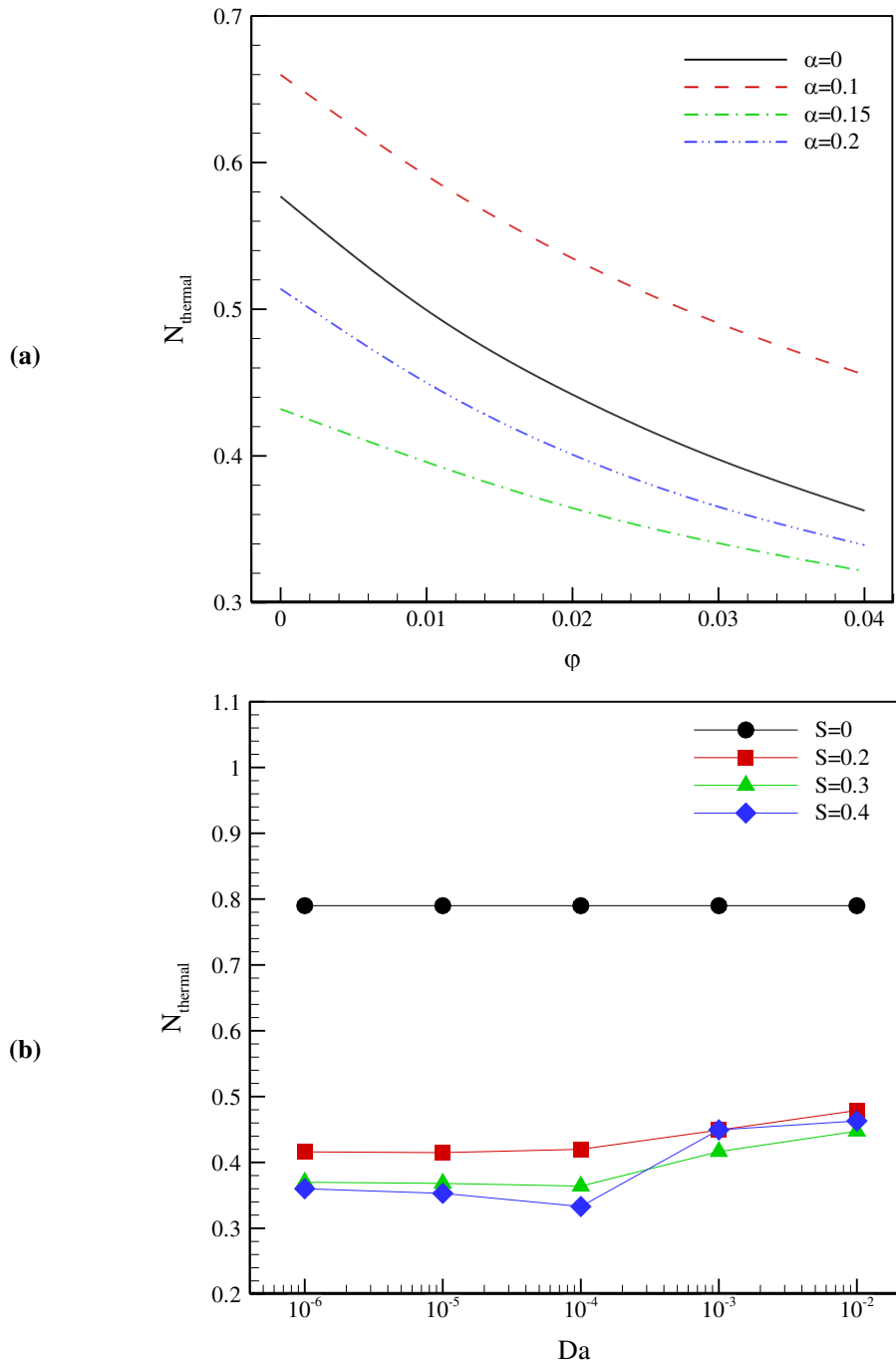
Fig. 16. Variations of the thermal entropy generation with a) volume fraction of nanoparticles for different values of wave amplitude at S = 0.3 and Da = 10^{-4} ; b) Darcy number for different values of non-dimensional thickness of the porous layer at \alpha = 0.15 and \phi = 0.02 .
