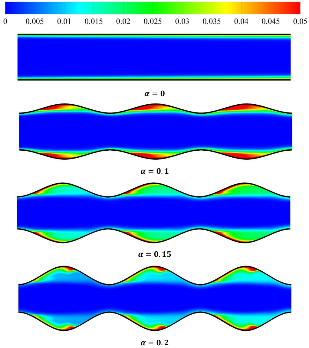
Fig. 7. Temperature distribution for different values of wave amplitude at S = 0.3 , Da = 10^{-4} and \varphi = 0.02 .
