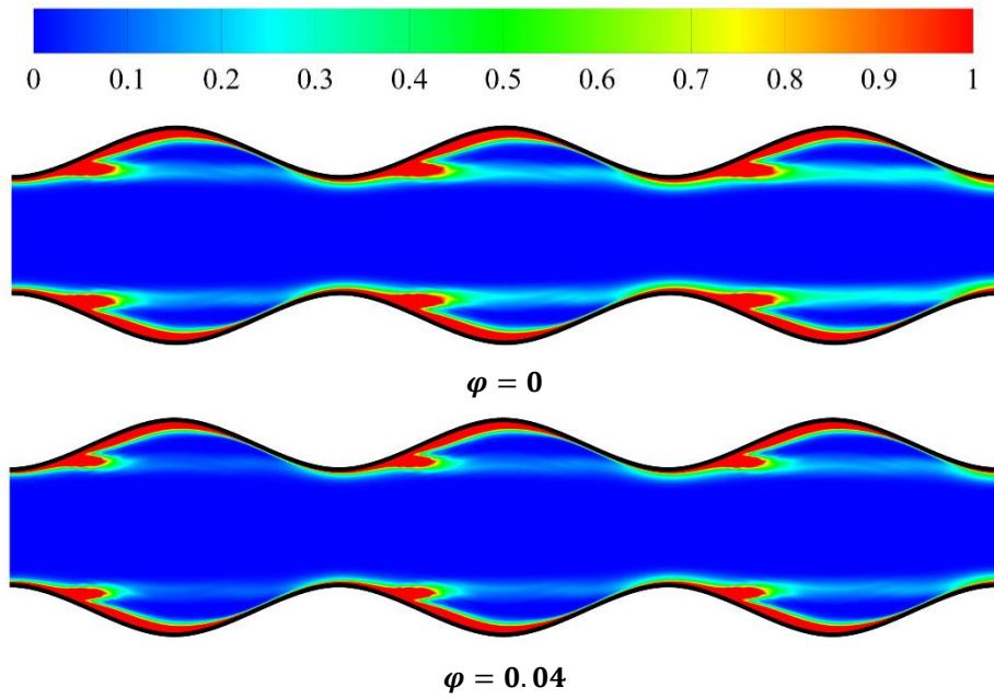
Fig. 11. Distribution of non-dimensional thermal entropy generation for two values of solid volume fractions of nanoparticles at S = 0.3 \cdot Da = 10^{-4} and \alpha = 0.15 .
