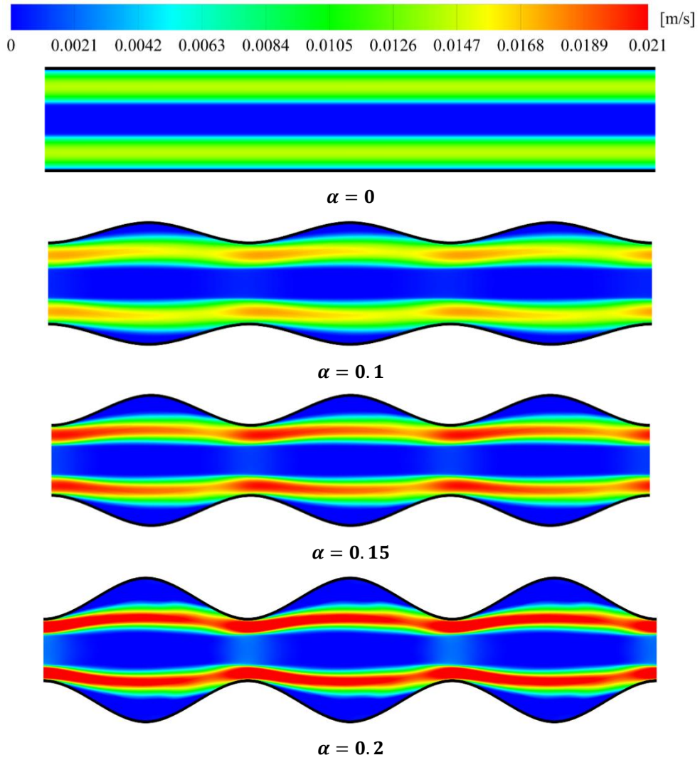
Fig. 6. Axial velocity distribution for different values of wave amplitude at S = 0.3 , Da = 10^{-4} and \varphi = 0.02 .
