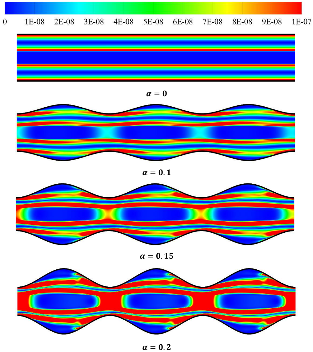
Fig. 14. Distribution of non-dimensional viscous entropy generation for different values of wave amplitude at S = 0.3 , Da = 10^{-4} and \varphi = 0.02 .
