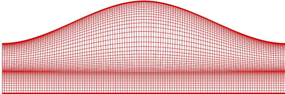
Fig. 2. Typical grid used in the computational domain.
