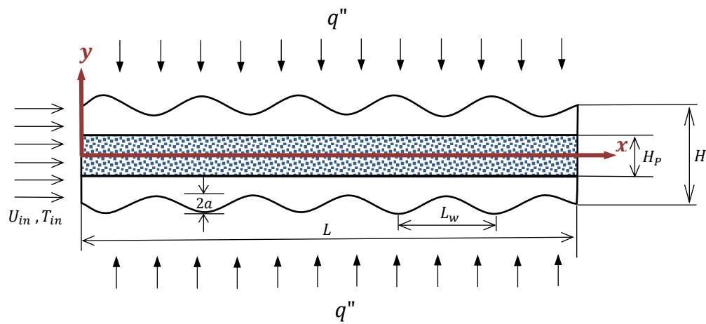
Fig. 1. Schematic view of the problem configuration
