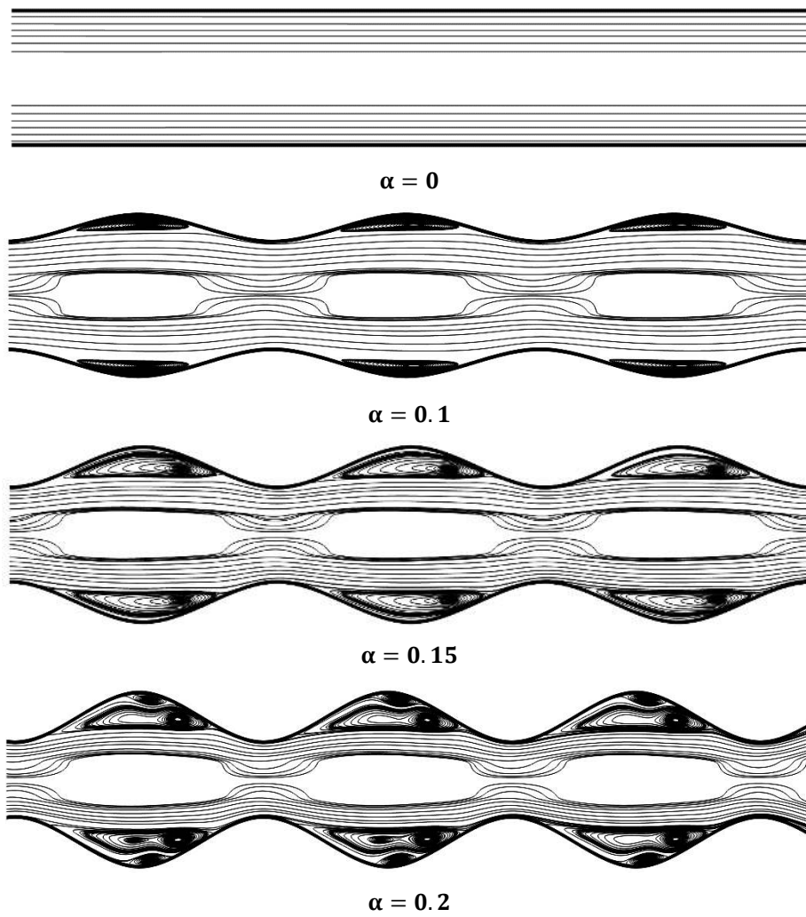
Fig. 5. Streamlines for different values of wave amplitude at S = 0.3 \cdot Da = 10^{-4} and \varphi = 0.02 .
