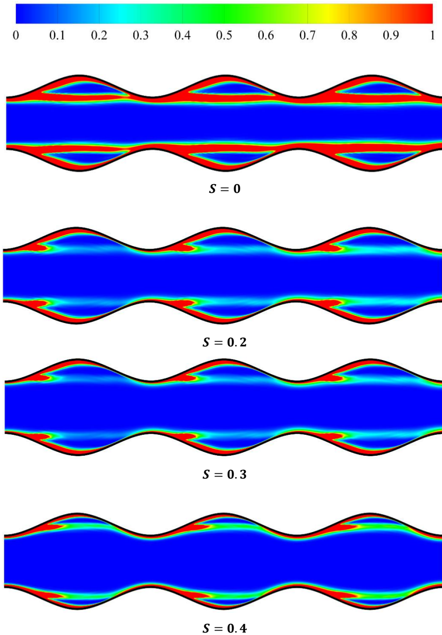
Fig. 12. Distribution of non-dimensional thermal entropy generation for different values of non-dimensional porous layer thickness at \phi = 0.02 \cdot Da = 10^{-4} and \alpha = 0.15 .
