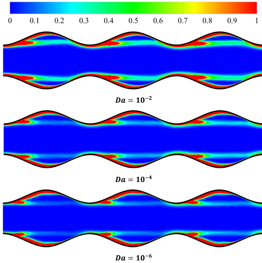
Fig. 13. Distribution of non-dimensional thermal entropy generation for different values of Darcy number at \varphi = 0.02 , S = 0.3 and \alpha = 0.15 .
