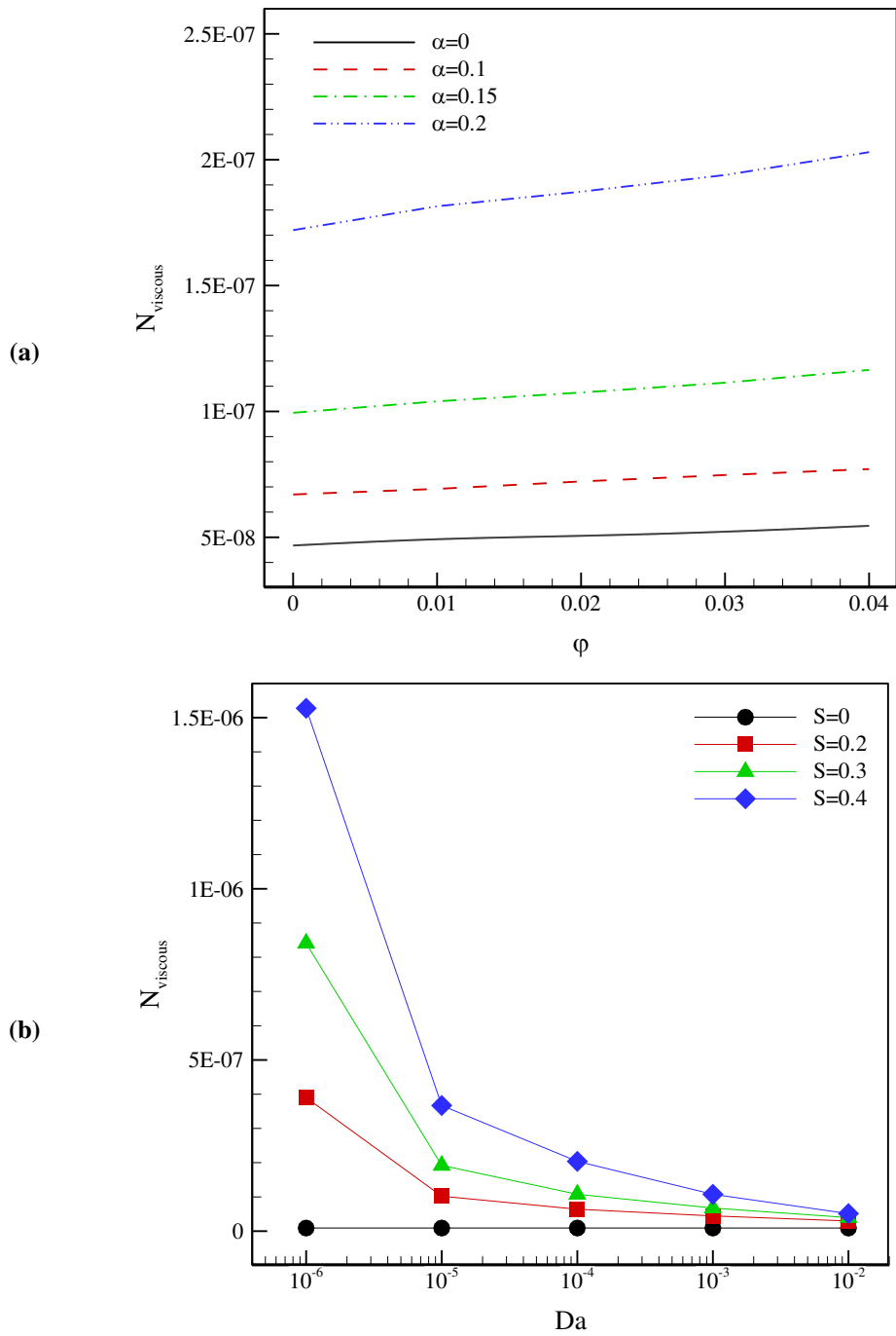
Fig. 17. Variations of the viscous entropy generation with a) volume fraction of nanoparticles for different values of wave amplitude at S = 0.3 and Da = 10^{-4} ; b) Darcy number for different values of non-dimensional thickness of the porous layer at \alpha = 0.15 and \phi = 0.02 .
