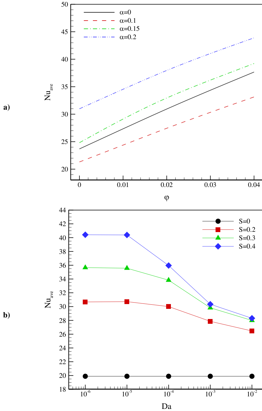
Fig. 8. Variations of the average Nusselt number with a) volume fraction of nanoparticles for different values of wave amplitude at S = 0.3 and Da = 10^{-4} ; b) Darcy number for different values of non-
