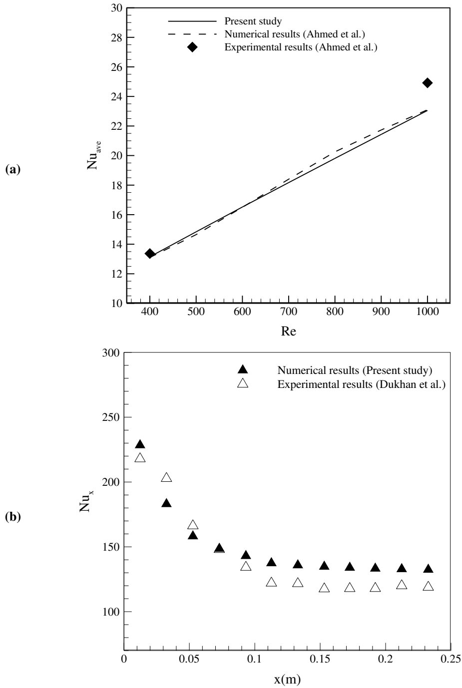
Fig. 3. Comparison between the present numerical results and the experimental and numerical results of Ahmed et al. [59] for averaged Nusselt number and experimental data of Dukhan et al. [60] for local Nusselt number.
