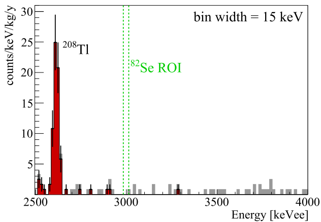
Fig. 6 High-energy spectrum of the \text{Zn}^{82}\text{Se} array collected in 530h before (gray) and after (red) the rejection of the \alpha background. The green lines indicate a FWHM region centered on the ^{82}\text{Se} Q-value
