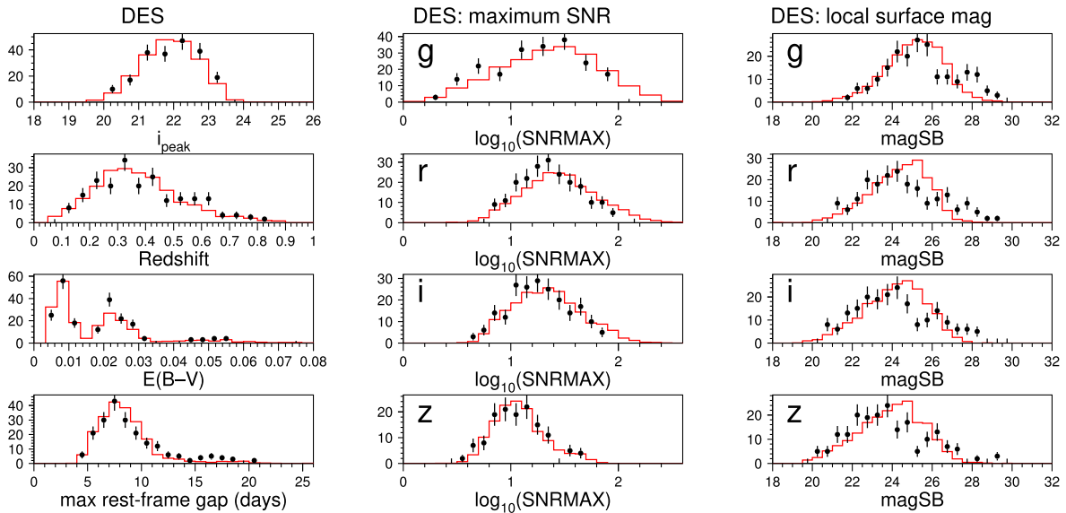
Figure 6. Comparison of data (black dots) and simulation with G10 scatterer model (red histogram) for distributions in the DES-SN sample, where the simulation is scaled to have the same number of events as the data. Left column shows i_{\text{peak}} , CMB redshift, Galactic extinction, and maximum gap between observations (rest frame). Middle column shows log of maximum SNR in each band. Right column shows local surface mag in each band.
