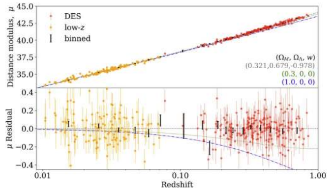
Figure 1. Hubble diagram for the DES-SN3YR sample. Top: distance modulus ( \mu ) from BBC fit (black bars, which are used for cosmology fits) and for each SN (red, orange circles). The dashed gray line shows our best-fit model, while the green and blue dotted lines show models with no dark energy and matter densities \Omega_m = 0.3 and 1.0 respectively. Bottom: residuals to the best-fit model; 1\sigma error bars show 68% confidence.
