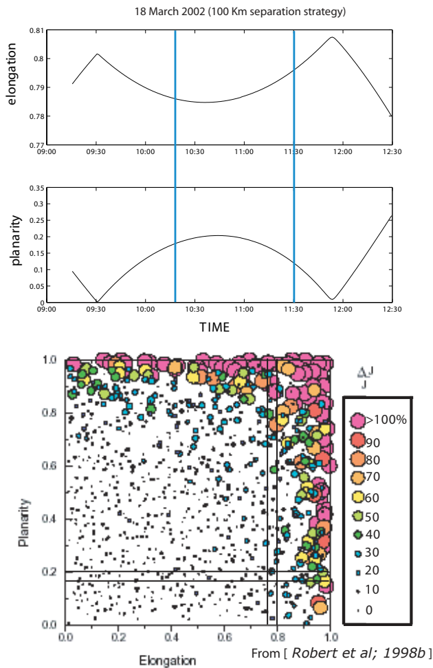
Fig. 1. Cluster spacecraft tetrahedron parameters for the 18 March 2002 perigee pass (upper panels), during which the spacecraft separation strategy was 100 km. The two blue vertical lines delimit the ring current traversal by the spacecraft. Bottom panel shows results of the study made by Robert et al. (1998b), which evaluated the influence of the tetrahedron shape (characterised by the tetrahedron parameters) on the estimate of |J| . Black lines demarcate the extreme values taken by the two parameters for spacecraft separation distances during the 18 March 2002 ring current interval. This separation can go up to 250 km at perigee, due to the keplerian evolution of the orbit (acceleration of the leading spacecraft). We can notice that the maximum uncertainty on |J| is never more than 20%.
