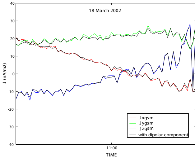
Fig. 3. Current density (in the the GSM coordinate system) as computed using two different magnetic field data inputs: FGM data (black curves) and FGM data from which we subtracted the dipolar field contribution (colored curves).
