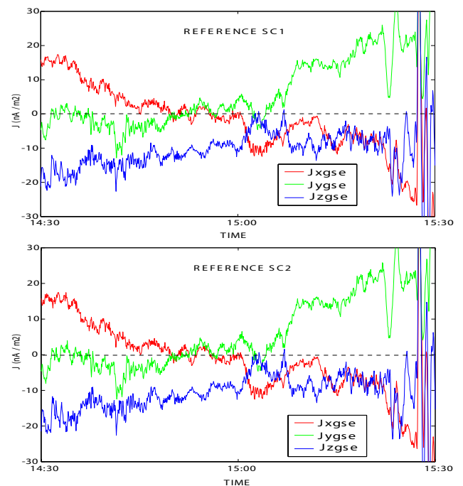
Fig. 2. Current density (in the GSE coordinate system) for the 13 April 2002 perigee pass, as computed using two different spacecraft of reference: SC1 (upper panel) and SC2 (lower panel).
