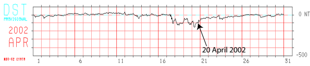
Fig. 12. D_{st} index values for April 2002. On the 20 April 2002 storm conditions are observed, while Cluster is passing through perigee. At 18:00 UT, the D_{st} index was about -101 nT.
