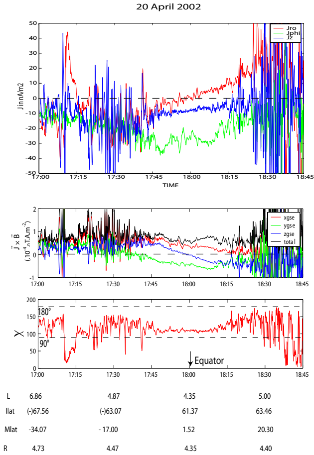
Fig. 14. Curlometer results for the 20 April 2002 event. From top to bottom: current density in the local cylindrical coordinate system and in \text{nA}\cdot\text{m}^{-2} , pressure gradient (computed from \mathbf{J}\times\mathbf{B} ), and \chi angle between local current flow and magnetic field. L-shell, invariant latitudes, magnetic latitudes and geocentric distances are indicated at the bottom of the plot.
