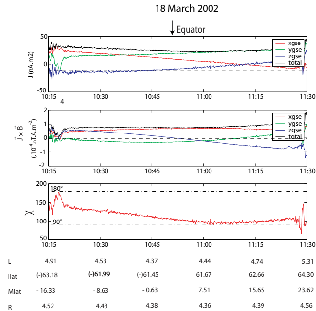
Fig. 11. Curlometer results for the 18 March 2002 event. From top to bottom: current density in the GSE coordinate system, pressure gradient (computed from \mathbf{J} \times \mathbf{B} ), and \chi angle between local current flow and magnetic field. L-shell, invariant latitudes, magnetic latitudes and geocentric distances are indicated at the bottom of the plot.
