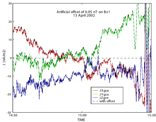
Fig. 4. Current density (in the GSE coordinate system) as computed using two different magnetic field data inputs: FGM data (colored curves) and FGM data to which we added an artificial offset of 0.05 nT on the B_z component (on SC1, black dashed curves).
