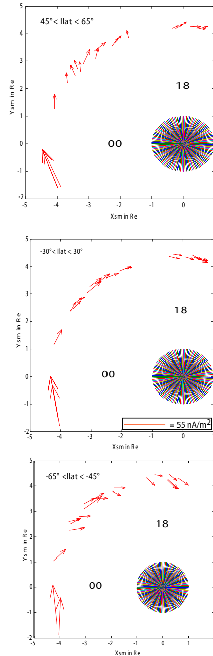
Fig. 15. Current density vectors for the February–June 2002 Cluster perigee passes, averaged over three invariant latitude intervals, and projected down to the equatorial plane: (a) from 45^\circ to 65^\circ (b) from -30^\circ to 30^\circ (c) from -45^\circ to -65^\circ
