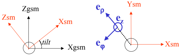
Fig. 6. Coordinate transformations from Geocentric Solar Magnetospheric into Solar Magnetic, and from Solar Magnetic into the local cylindrical coordinate system [ e_\rho, e_\phi, e_z ], used in our analysis. The black circle represents the Earth, and the blue circle the Cluster spacecraft tetrahedron.
