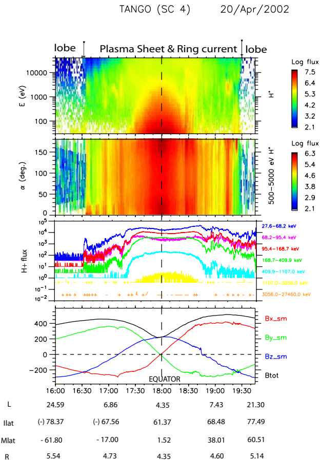
Fig. 13. Cluster SC4 data for the 20 April 2002 event: H^+ energy-time spectrogram in particle flux units (ions/cm 2 sr s keV), the pitch-angle distribution (in particle flux units) for the 0.5 to 5 keV energy range, the H^+ energy-time spectrogram from the RAPID instrument (27.6–3056.0 keV), and the magnetic field components in the SM coordinate system. L-shell, invariant latitudes, magnetic latitudes and geocentric distances are indicated below. Dashed line represents the equatorial crossing.
