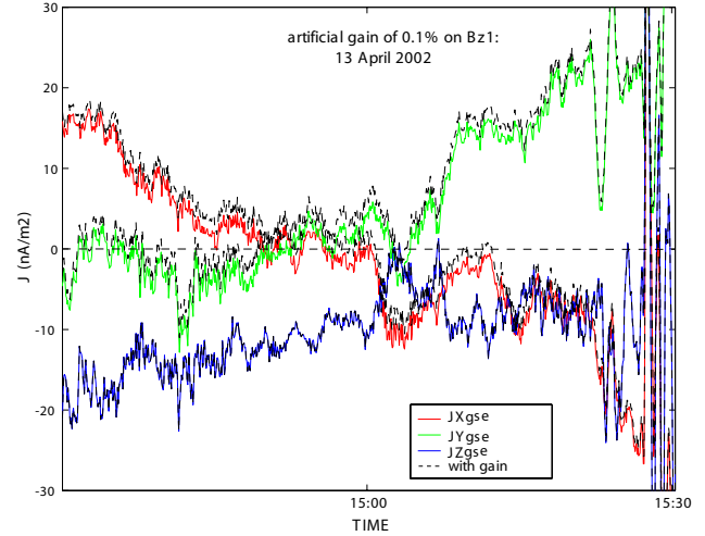
Fig. 5. Current density (in the GSE coordinate system) as computed using two different magnetic field data inputs: FGM data (colored curves) and FGM data to which we added an artificial gain of 0.1% on the B_z component (on SC1, black dashed curves).
