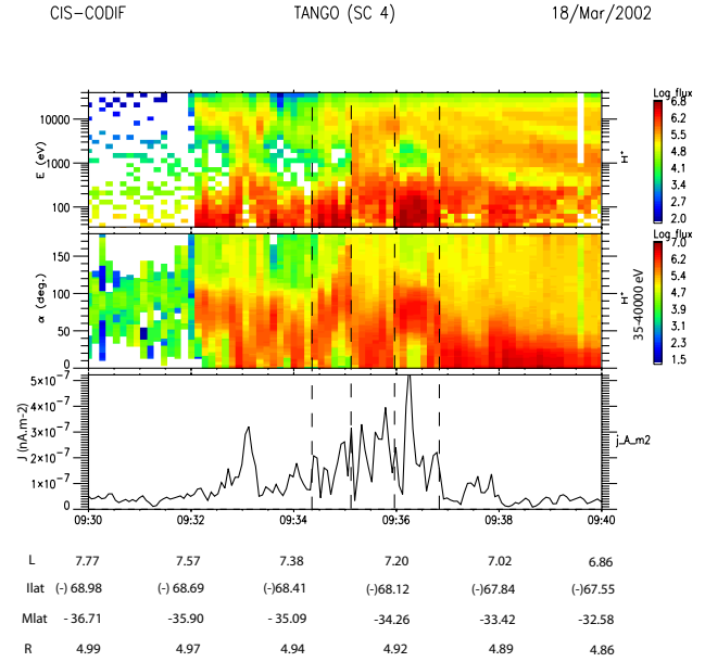
Fig. 10. Inner plasma sheet zoom for the 18 March 2002 event: H^+ energy-time spectrogram in particle flux units (ions/cm 2 sr s keV), pitch angle distribution for the 35–40000 eV energy range in particle flux units (ions / cm 2 sr s keV) and total current density in nA.m -2 . L-shell, invariant latitudes, magnetic latitudes and geocentric distances are indicated below.
