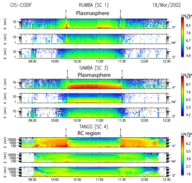
Fig. 8. CIS-CODIF data for the 18 March 2002 event: H^+ , He^+ , O^+ energy-time spectrograms in particle flux units ( \text{ions}/\text{cm}^2 \text{ sr s keV} ) from SC1, SC3 and SC4. CODIF on SC1 and SC3 were using the RPA mode, allowing measurements of plasma particles from \sim 1 \text{ eV} to \sim 25 \text{ eV} , characteristic of the plasmasphere. CODIF on SC4 was operating in a normal magnetospheric mode ( 25 \text{ eV} – 40 \text{ keV} ) which allows the detection of the ring current particles. We thus are using the SC1 and 3 to monitor the position of the plasmasphere/plasmapause, and SC4 to monitor the ring current. As it appears on these 3 spectrograms, and taking into account that the spacecraft separation was only a few hundred kilometers, the plasmasphere and the ring current boundaries were almost collocated for this event, at the MLT sector of the Cluster trajectory (see text for details).
