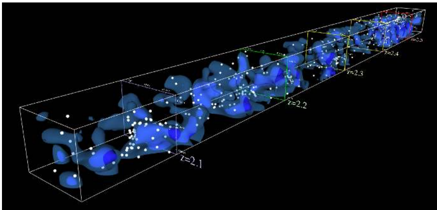
Figure 12. Three-dimensional rendering of the CLAMATO tomographic map, showing two isodensity contours at \delta_F^{\text{rec}} = -0.08 and \delta_F^{\text{rec}} = -0.18 , along with coeval galaxy positions shown as dots. This figure is available online as an interactive figure ( http://www2.mpa-hd.mpg.de/homes/tmueller/projects/clamato/map2017.html ) — it requires a load-time of several minutes. By left-clicking and moving the mouse, the viewpoint can be rotated, while the right-mouse button or scroll wheel can be used to zoom in or out; double left-clicking at any point in the map focuses the viewpoint there. The buttons labeled ‘Isosurface: -0.08’ and ‘-0.18’ toggles the respective isodensity surfaces on and off. The ‘Reset View’ button restores the figure to its default state and perspective.
