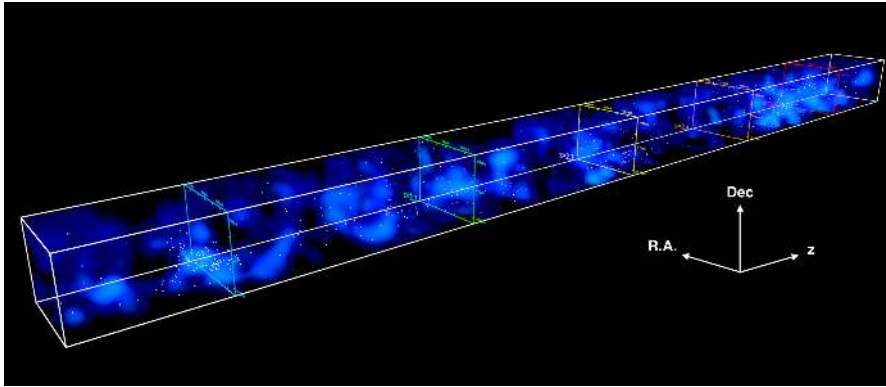
Figure 11. Still image from our 3D video visualization of the CLAMATO reconstructed absorption map (smoothed with a R = 2 h^{-1} Mpc Gaussian kernel), where the absorption is indicated by the blue transparency. Foreground galaxy redshift positions are denoted by the yellow dots, while the triad (not present in the video) indicates the directions of increasing R.A., declination, and redshift. The full video, which offers a virtual reality option when viewed with a smartphone and Google Cardboard-compatible headset, can be viewed on https://youtu.be/QGtXi7P4u4g .
