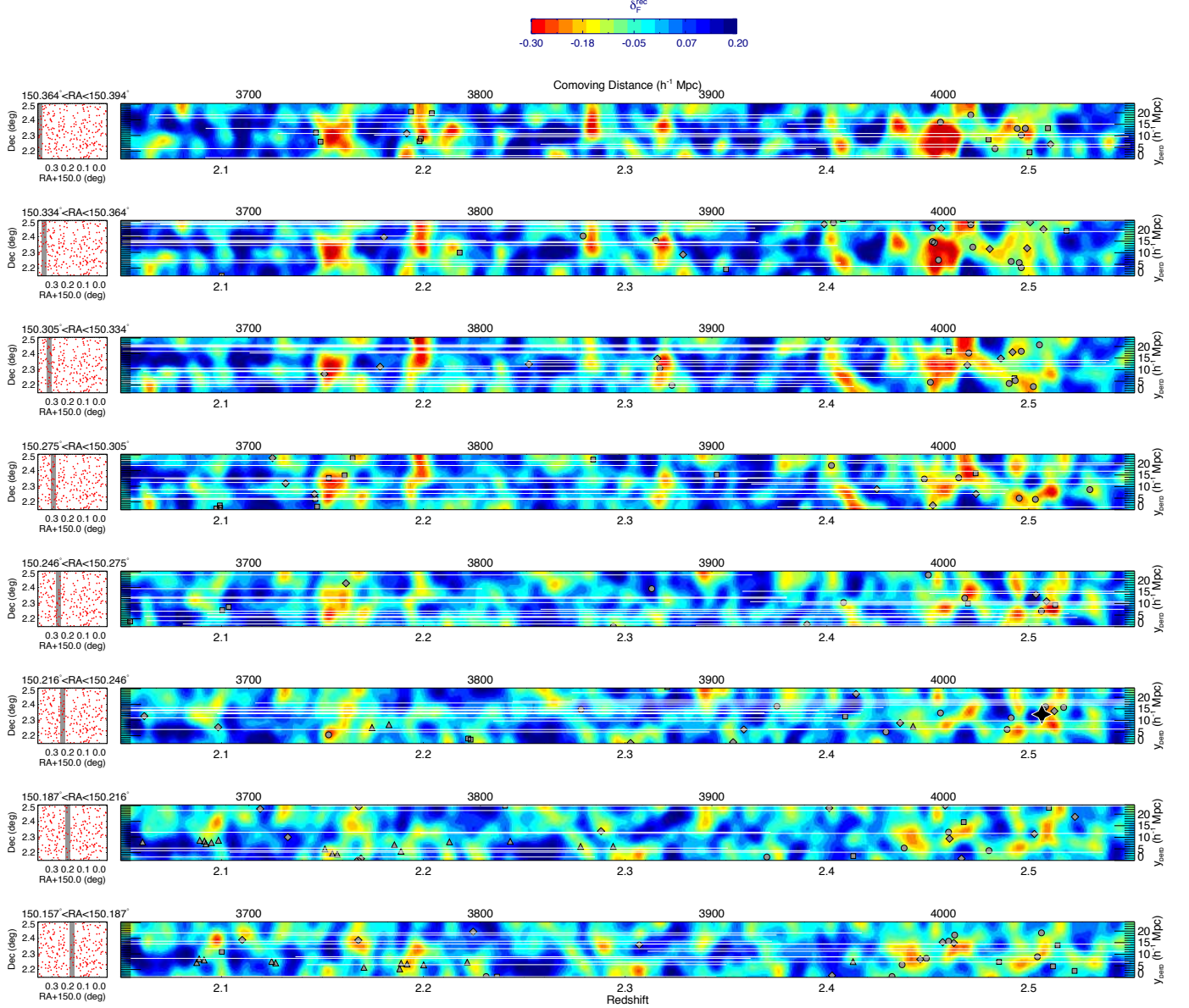
Figure 9. Wiener-filtered tomographic reconstructions of the Ly \alpha forest absorption field, \delta_F^{\text{ec}} , at 2.05 < z_\alpha < 2.55 from the current CLAMATO data (color map), shown after smoothing with an isotropic R = 2 h^{-1} Mpc Gaussian kernel. Each color panel shows the absorption projected over a 2 h^{-1} Mpc R.A. slice, the position of which is denoted by the shaded region in the subpanels to the left that also show the sightline positions on the sky as red dots. The color convention for the absorption is such that red denotes overdensities while blue denotes underdensities. White horizontal lines denote the sightline coverage, while symbols mark the location of known foreground galaxy redshifts: downwards triangles from MOSDEF, upwards triangles from ZFIRE, squares from VUDS, diamonds from zCOSMOS-Deep, and circles from CLAMATO. The large black stars indicate the reported central positions of the galaxy overdensities at z = [2.10, 2.44, 2.47, 2.51] . This sequence is continued in Figure 10.
