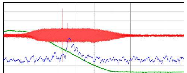
Figure 4: Oscilloscope screenshot (500 ns/div) showing the Q out signal from the first BPM (red, horizontal), the raw ICT (blue curve), and the Faraday cup signal (green line). The short spike on the BPM signal corresponds to the laser-induced electron bunch, also visible as peak on the ICT signal.
