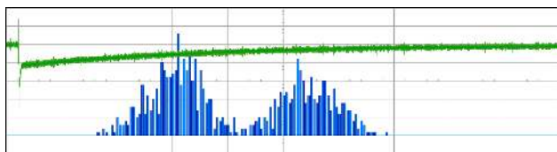
Figure 6: Oscilloscope screenshot (200 μs/div) showing the signal from the Faraday cup (green). The histogram is displayed in blue. The left peak corresponds to charge from laser-induced electrons, the right peak from dark current. In contrast to the other plots, this measurement was recorded with a klystron forward power of only 6.6 MW leading to an electron energy of 4.3 MeV.
