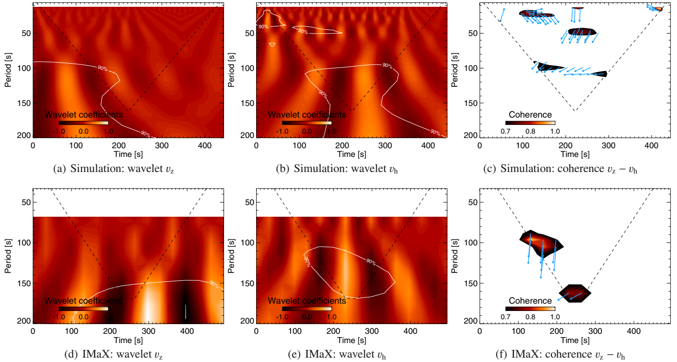
Fig. 4. a) Wavelet amplitude spectrum of v_z from the simulation. b) Wavelet amplitude spectrum of v_h from the simulation. c) Wavelet phase coherence spectrum between v_z and v_h from the simulation. The arrows represent the phase lag in polar coordinates (zero phase corresponds to arrows pointing to the right). d) Wavelet amplitude spectrum of v_z from IMAx. e) Wavelet amplitude spectrum of v_h from IMAx. f) Wavelet phase coherence spectrum between v_z and v_h from IMAx. The arrows represent the phase lag in polar coordinates (zero phase corresponds to arrows pointing to the right). The dashed line represents the cone of influence where results cannot be trusted (area between the dashed lines and the edges of the diagram). The white contours represent the 95% confidence level.
