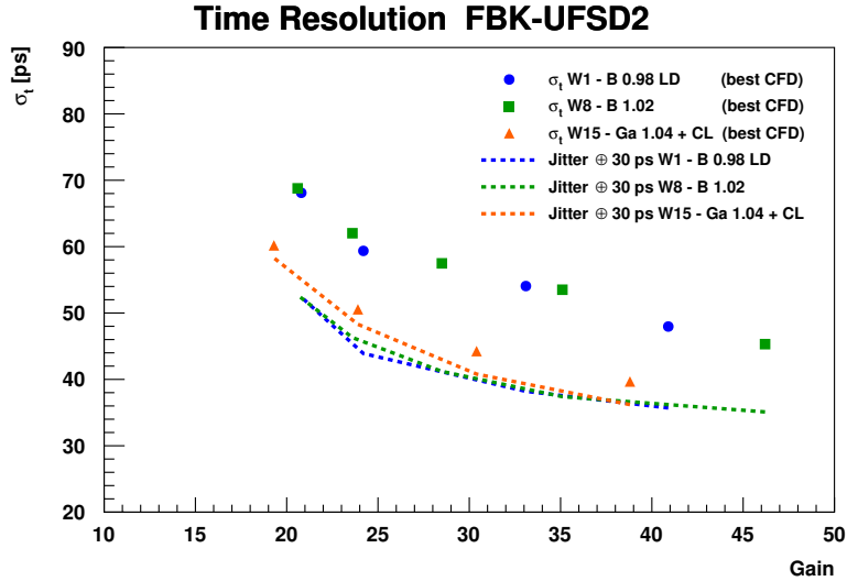
Figure 9: Time resolution as a function of the gain measured on sensors with three different gain layer configuration: Boron Low Diffusion (blue dots), Boron (green squares), and Gallium + Low Carbon (orange triangles). Jitter contributions plus the predicted Landau noise of \sim 30 ps are also shown as dotted lines.
