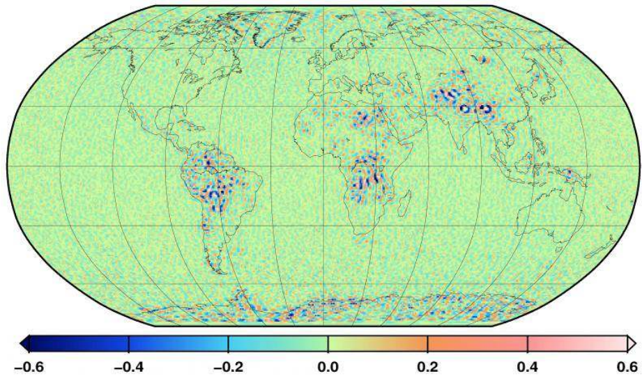
Fig. 20 Geoid height differences [m] between GOCE (DIR) and EGM2008 up to degree/order 240
