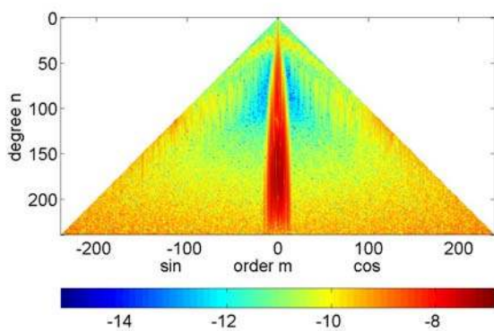
Fig. 7 Differences in the estimated spherical harmonic coefficients C_{nm} and S_{nm} due to regularization, displayed in \log_{10} scale
