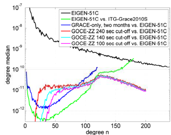
Fig. 5 Degree median spectra of GOCE SGG-ZZ only solutions (direct approach) obtained with different filters compared to EIGEN-51C: 1 – EIGEN-51C; 2 – EIGEN-51C versus ITG-Grace10s; 3 – a GRACE-only two-months solution versus EIGEN-51C; 4,5,6 – GOCE SGG-ZZ-only solutions versus EIGEN-51C for 240, 140 and 100 seconds high-pass cut-off periods
