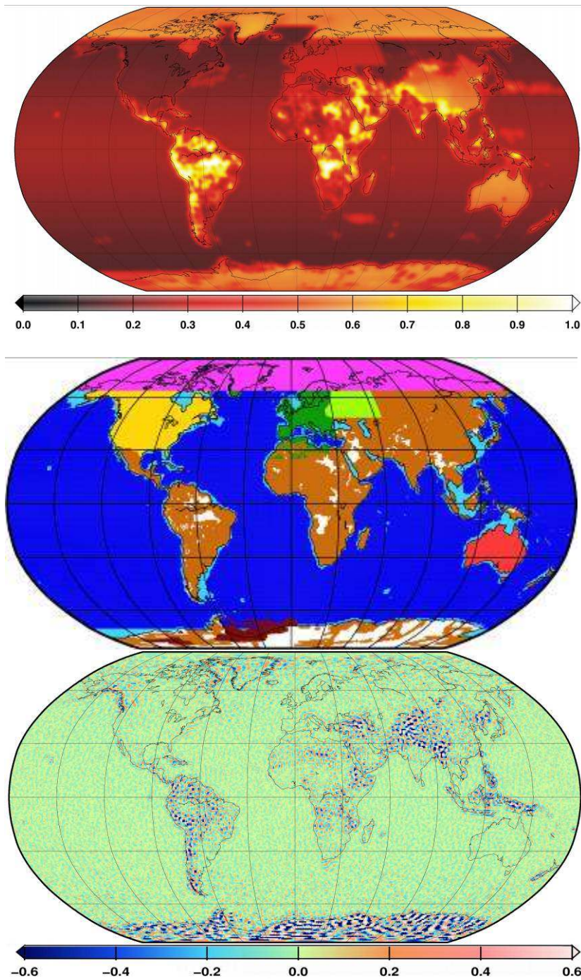
Fig. 19 Comparison of EIGEN-5C with the GOCE (DIR) model: a) geoid height error [m] of EIGEN-5C obtained by rigorous error propagation from the full variance/covariance matrix up to degree/order 260; b) patchwork of the terrestrial and altimetry data as used for EIGEN-5C; c) geoid height differences [m] between GOCE and EIGEN-5C, up to degree/order 240
