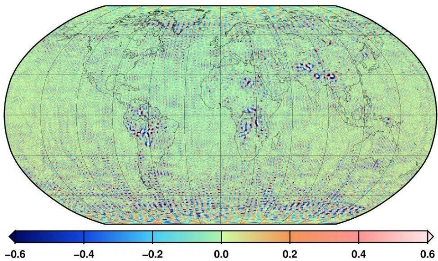
Fig. 21 Geoid height differences [m] between ITG-Grace2010s and EGM2008 up to degree/order 180
