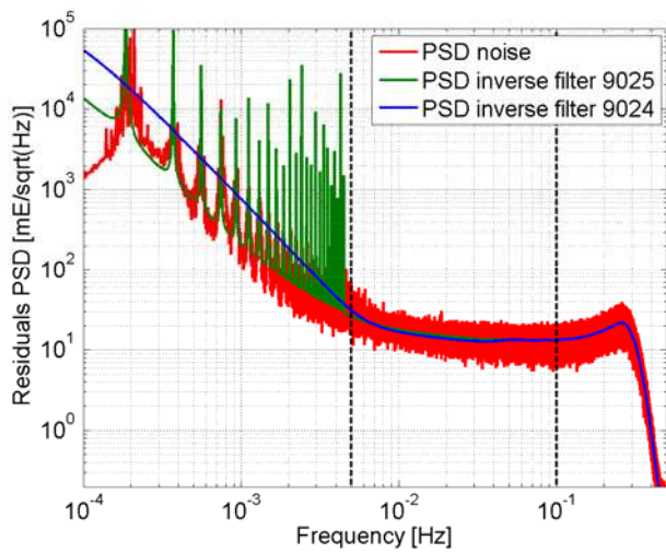
Fig. 9 Gradiometer noise and different SGG filter models of the gravity gradient component V_{ZZ}
