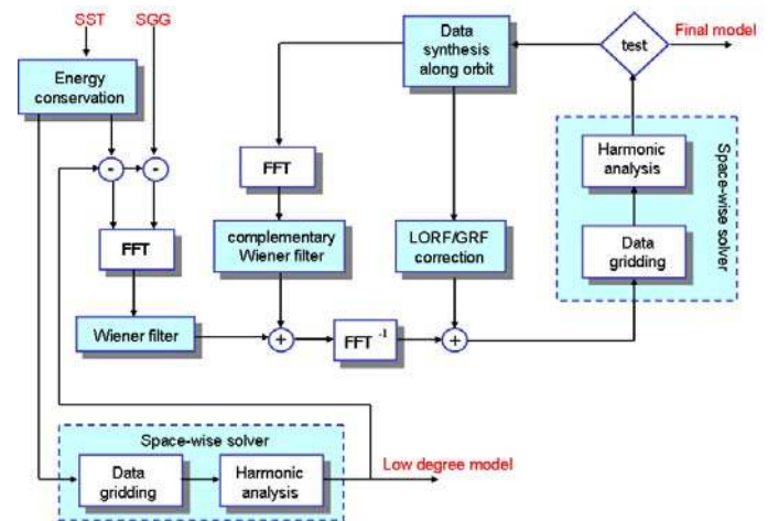
Fig. 12 The space-wise iterative scheme
