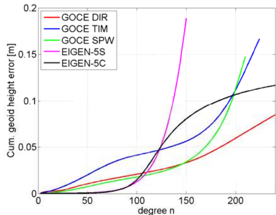
Fig. 16 Cumulative geoid height errors [m] of the three GOCE models DIR, TIM and SPW, and the EIGEN satellite-only and combined models EIGEN-5S and EIGEN-5C as a reference
