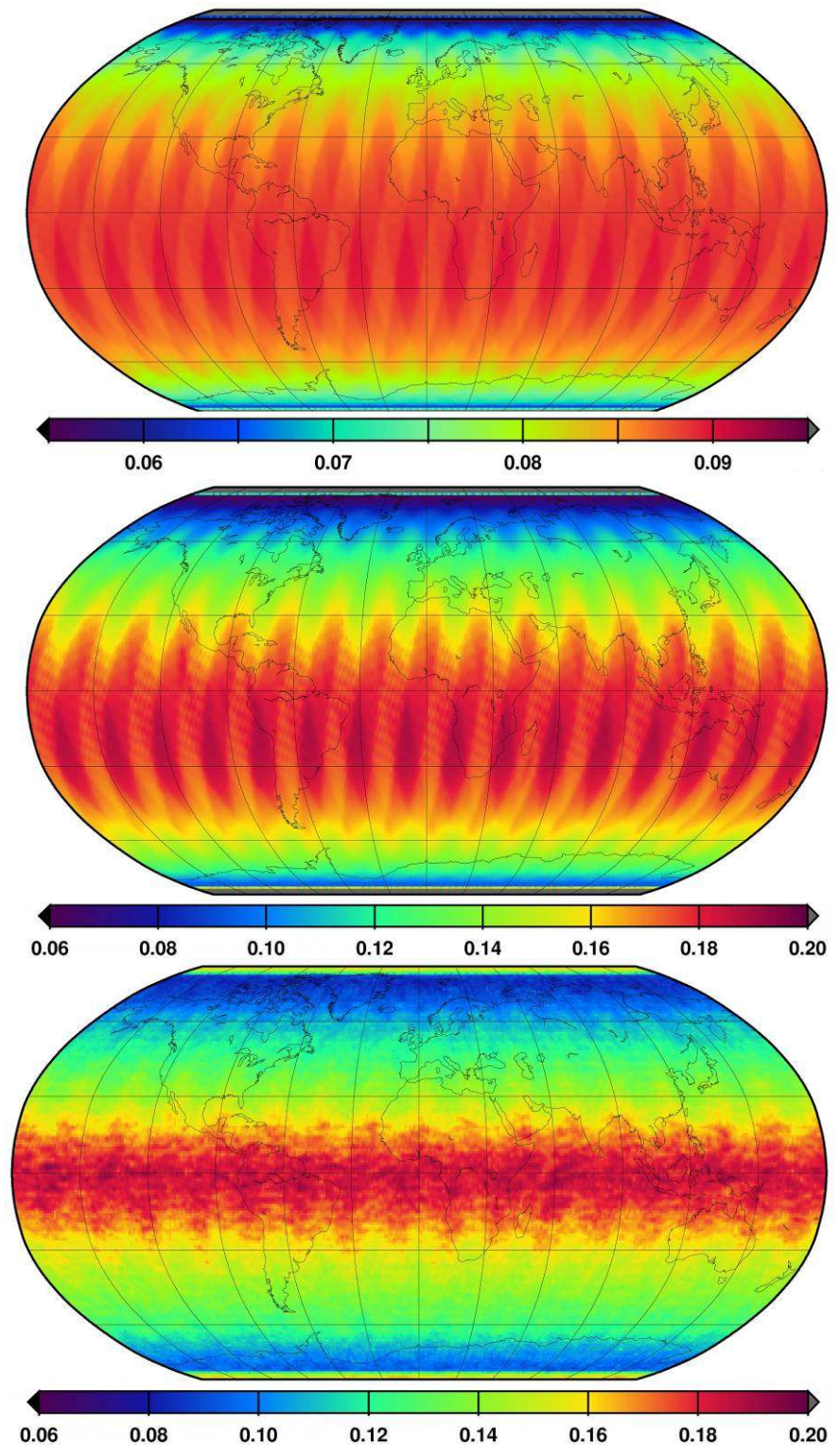
Fig. 17 Propagated geoid height errors [m]: (a) DIR; (b) TIM; (c) SPW; please note the different scale of DIR compared to TIM and SPW
