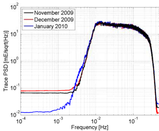
Fig. 4 Amplitude spectra of the trace for two days in November 2009 (black), December 2009 (red), and January 2010 (blue), respectively
