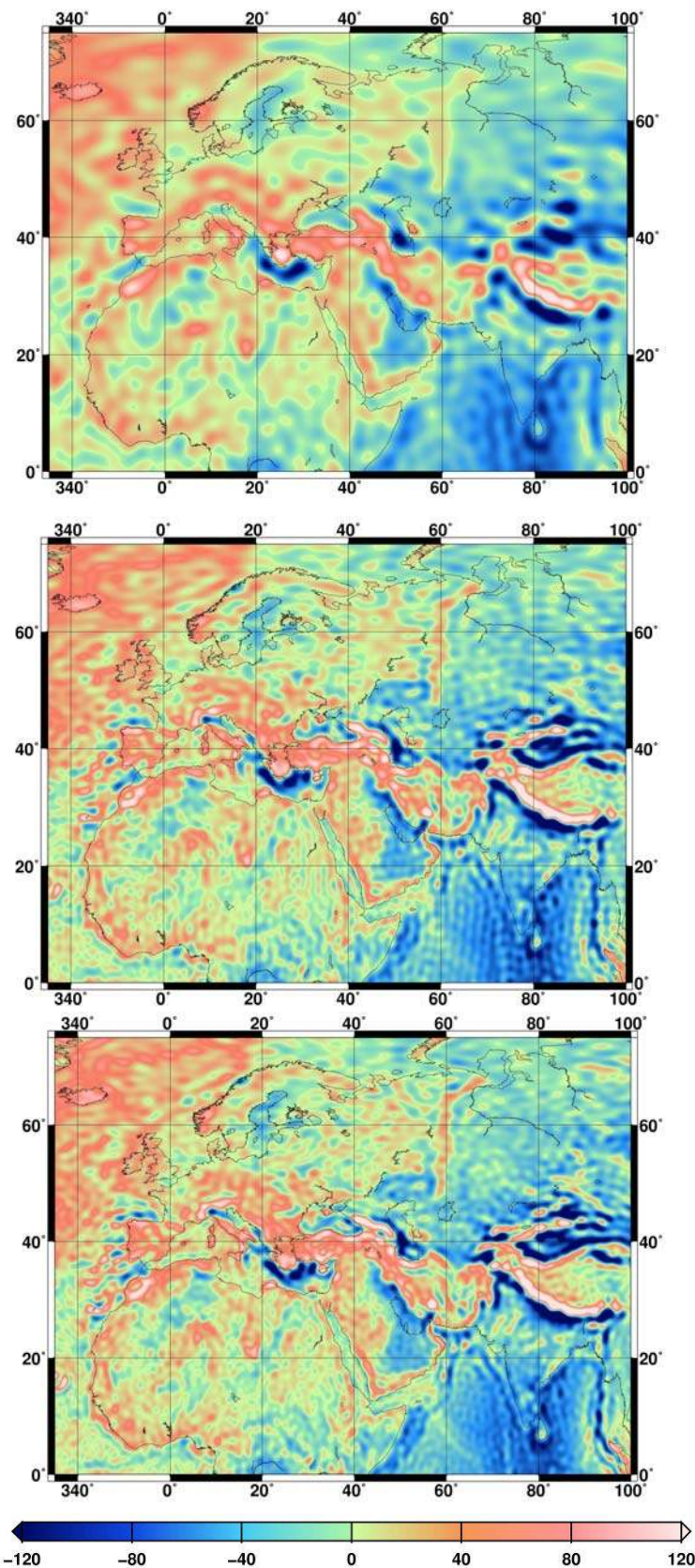
Fig. 18 Gravity anomalies over Europe, Western Asia and Northern Africa (mGal) from a) CHAMP (AIUB-CHAMP03S); b) GRACE (ITG-Grace2010s); c) GOCE (TIM)
