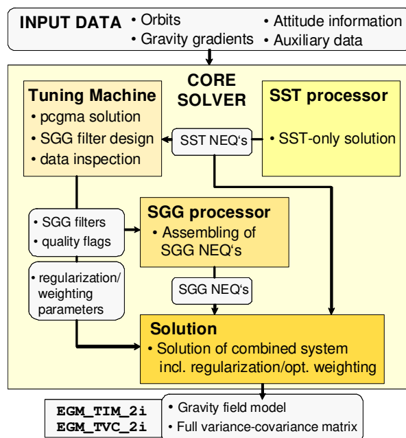
Fig. 8 Software architecture and product flow of the time-wise gravity field processing
