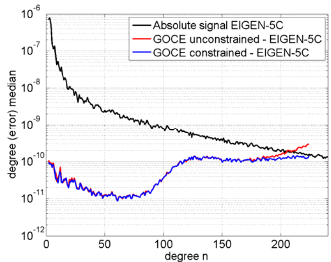
Fig. 10 Degree medians of constrained vs. unconstrained TIM solution
