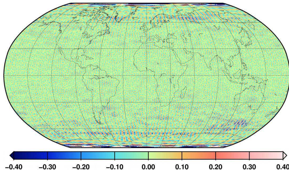
Fig. 23 Geoid height differences [m] between ITG-Grace2010s and GOCE (TIM) for the spherical harmonic degree range 80 to 160
