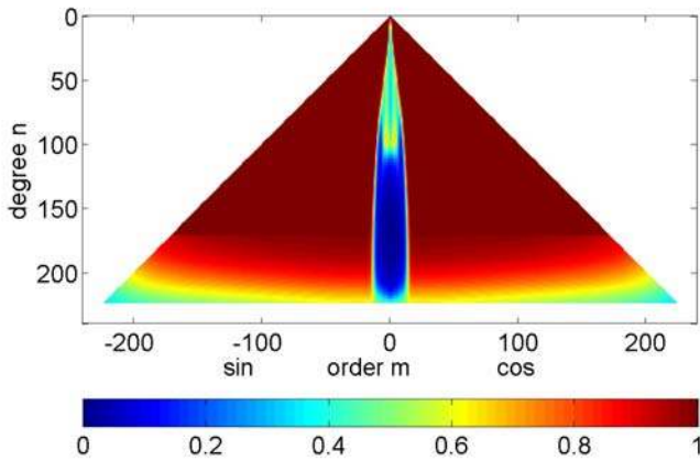
Fig. 11 Redundancy factors of constrained TIM solution. A value of '1' means that a certain coefficient is determined solely from GOCE information
