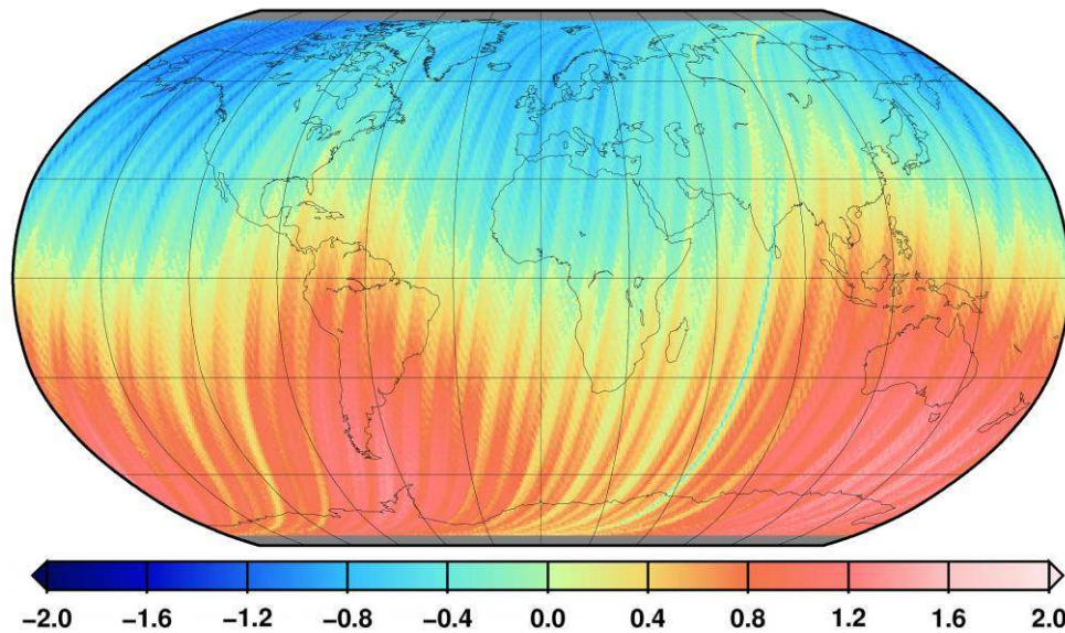
Fig. 2 Spatial distribution of the gradiometer noise (Eötvös) for the descending tracks of the V_{zz} gravity gradients (defined in the GRF)
