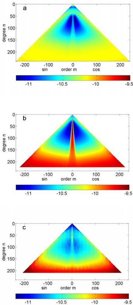
Fig. 15 Estimated coefficient standard deviations: a) DIR; b) TIM; c) SPW. Scaling is \log_{10}(\dots)
