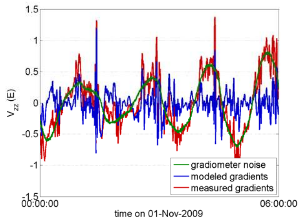
Fig. 1 Time series of the gradiometer noise of the V_{zz} component in comparison to the signal derived from EIGEN-5C. All curves have been reduced by GRS80 normal field and mean value
