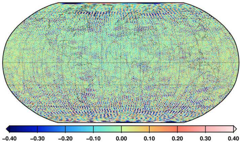
Fig. 22 Geoid height differences [m] between ITG-Grace2010s and GOCE (SPW) up to degree/order 180
