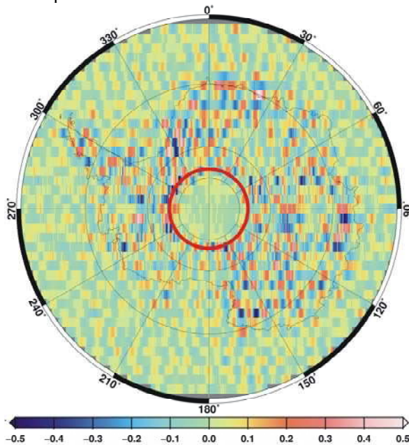
Fig. 6 Geoid height differences [m] over the south pole between the GOCE gravity field from DIR and the reference field EIGEN-51C, which has been used for the spherical cap regularization. The GOCE polar gap is indicated by a red circle
