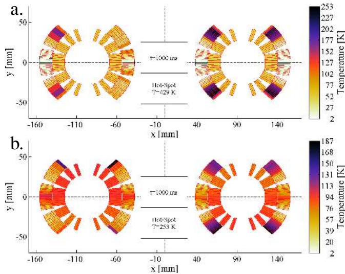
Fig. 7. Simulated magnet temperature over the cross-section of the coil windings of Apertures 1 and 2 (right and left, respectively), at 1 s after detection of a quench at nominal current. a. Triggering 4 QH. b. Triggering CLIQ and 2 QH. Note the difference in the two temperature scales.
