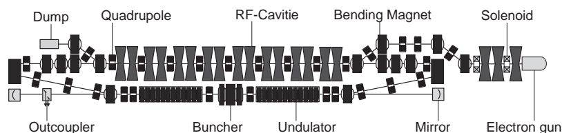
Fig. 1. Scheme of the first stage of Novosibirsk high-power free electron laser.
