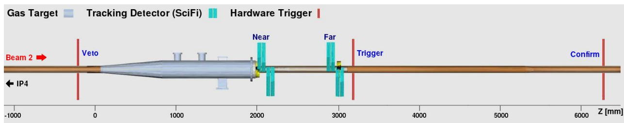
Figure 1: The BGV detector consists of three main parts: the gas target, the tracking detector & the hardware trigger.
