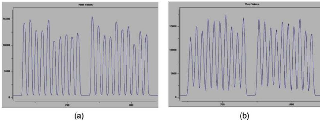
Fig. 26 (a) Plots of flux versus pixel position for a vertical cut across a fiber flat field image, zoomed in the center of the detector in the HERMES red channel. Note the flux going down to the bias level between the two slitlets, and the flux between the individual fibers goes down similarly. (b) Plots of the vertical cut in the same fiber flat, zoomed into the top of the detector. Note, here, the flux between the two slitlets goes down to bias level, but the flux level between individual fibers does not, indicating there is illumination from the adjacent fibers.
