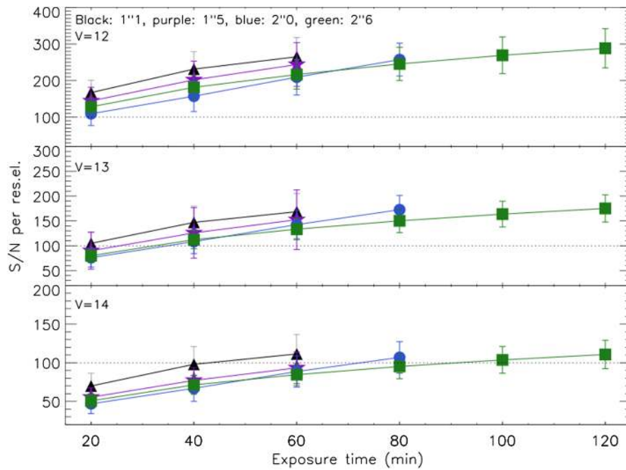
Fig. 22 HERMES can meet the design requirement that signal to noise per resolution element (S/N) should be 100 at V = 14 in 1 hour of integration time, though this is modulated by the seeing. We have chosen stars with V magnitudes near 12, 13, and 14 (top, middle, and bottom panels) from fields for which our observers recorded seeing of 1''1 (black), 1''5 (magenta), 2''0 (blue), and 2''6 (green). We measure the mean value for S/N at 60 min, V = 14 of 111.4 (seeing = 1''1 ), 93.4 (seeing = 1''5 ) and 88.6 (seeing = 2''0 ). Our observers extend the integration time by 20 min when the seeing is worse than 2'' and by 60 min when the seeing is worse than 2''5 , and it can be seen in the figure that this is effective at bringing the S/N up to the required levels.
