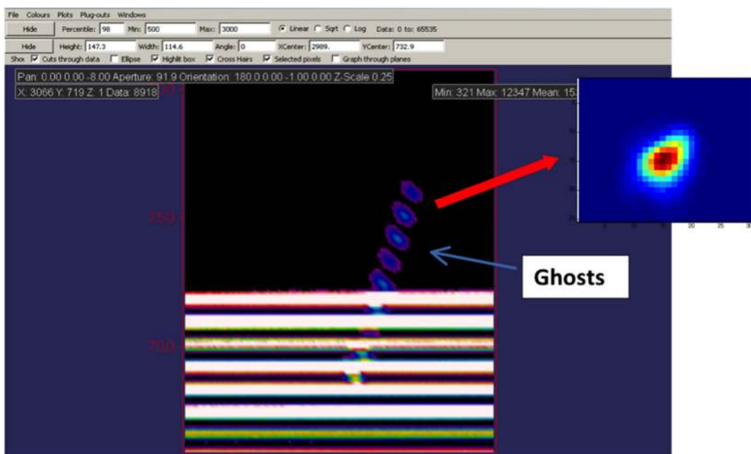
Fig. 23 A test flat field exposure with some of the fibers masked to identify the ghost.
