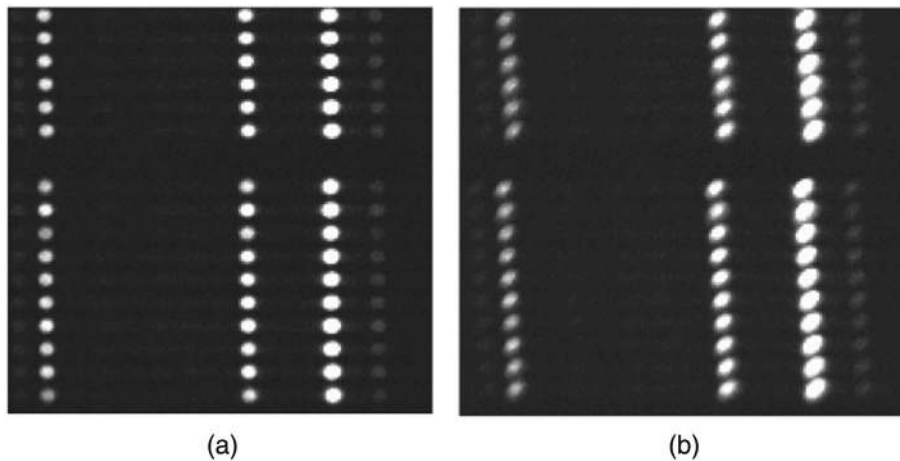
Fig. 24 (a) Image of an arc exposure zoomed in the center of the detector in the HERMES Red channel. The point spread function (PSF) convolved with a fiber images are round and the PSF convolved with a fiber images for adjacent fibers do not overlap significantly. (b) Image of the same arc exposure zoomed in the top of the detector. The PSF convolved with a fiber images is now an inclined ellipse and the PSF convolved with a fiber images for adjacent fibers do partly overlap.
