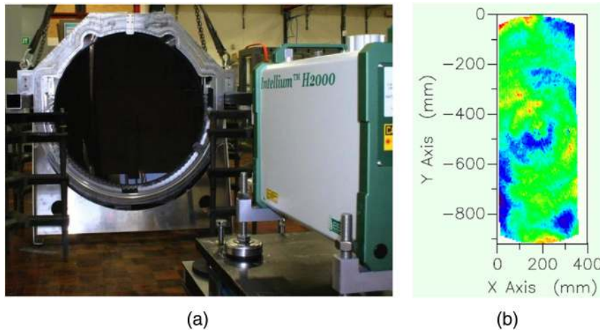
Fig. 16 (a) The mounted collimator mirror before coating and (b) its interferogram, P - V = 0.1 wave, RMS = 0.013 wave.
