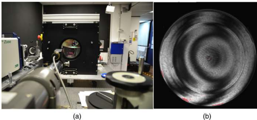
Fig. 11 (a) Camera under test with the autocollimating alignment telescope after interferometric testing, (b) IR camera transmitted wavefront using the null lens resulting in a measured wavefront of RMS 0.17 wv and PV 1.88 wv at 632.8 nm.
