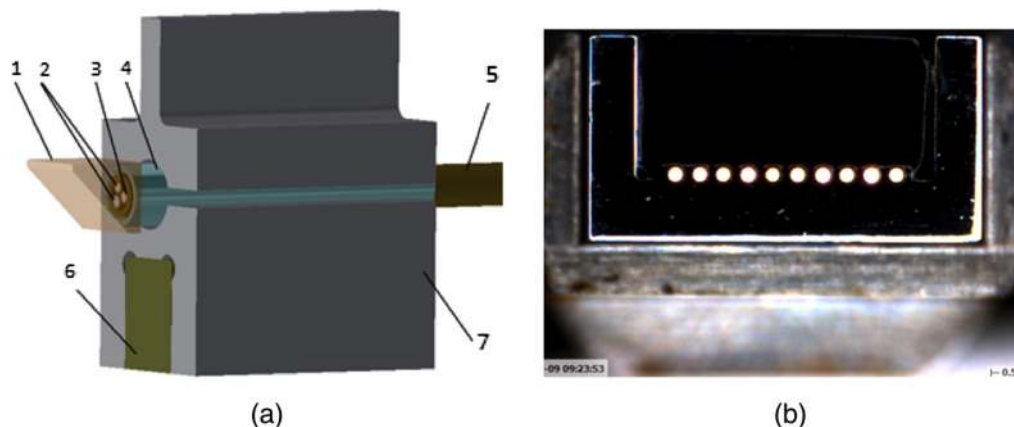
Fig. 19 (a) 2dF button; 1–prism, 2–AAOmega/HERMES science fibers, 3–dummy fiber, 4–glass ferrule, 5–polyimide tube, 6–magnet, 7–button body (prism size is 1 mm). (b) The back-illuminated output slitlet, containing 10 fibers as seen from the spectrograph.
