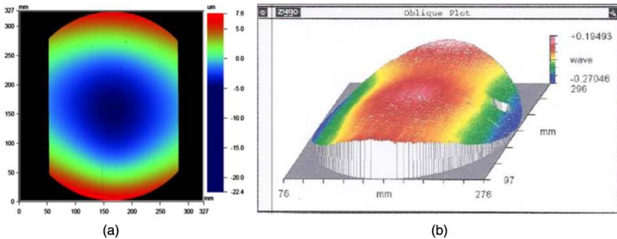
Fig. 17 (a) Red VPHG transmitted wavefront error profile before repolishing and (b) red VPHG transmitted wavefront at repolish at working angle of 62 deg.
