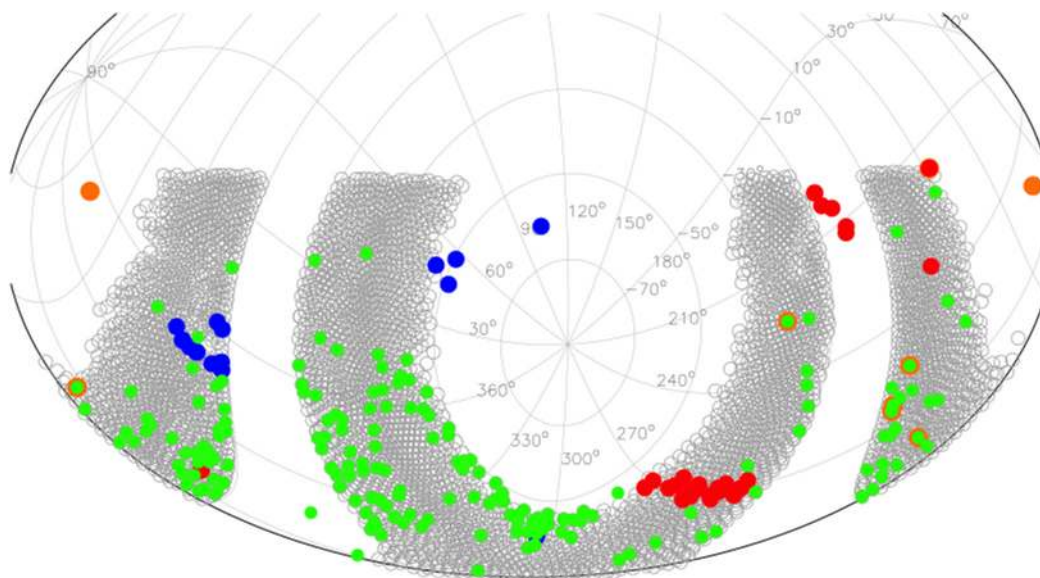
Fig. 29 The distribution across the sky of pilot survey (red), test (orange), main survey (green), and Kepler-2 (blue) fields. Main survey fields that also serve as test data are shown as green circles with an orange ring. There are 4303 field centers, shown as gray open circles, which are tiled into 6546 “configurations” containing 400 unique stars. The ultimate goal of a million-star sample requires observing 3200 of these configurations.
