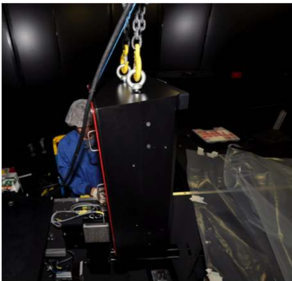
Fig. 7 Corrector lens being lowered into their kinematic mounts within the frame.
