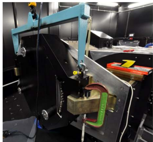
Fig. 5 Collimator mirror craned on top of the spine mount.
