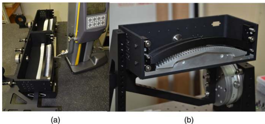
Fig. 14 (a) The two curved slit assemblies on the translation stage and (b) V-groove block for lens mounting 40 lens sets. Each lens set is used to modify the F/# output from 10 fibers to match the collimator input, including a margin for FRD. In this way the light from all 400 fibers are correctly injected into the spectrograph.
