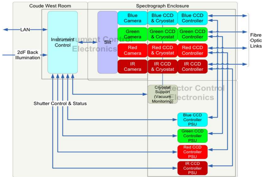
Fig. 20 Overview of the 2dF observing system software tasks when running in HERMES mode.
