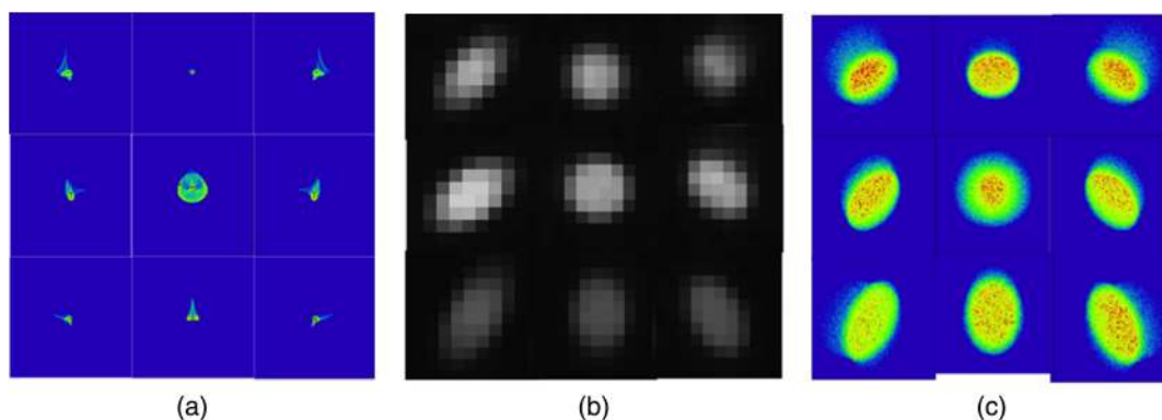
Fig. 25 (a) The design PSF of the spectrograph; (b) a mosaic of measured fiber images from the center and edges of the field for a blue camera arc exposure, compared with 25c; (c) a set of corresponding predicted images from Zemax ray-tracing done during the optical design study. The distortions seen toward the edges of the field match the predictions well. Horizontal is the spatial direction.
