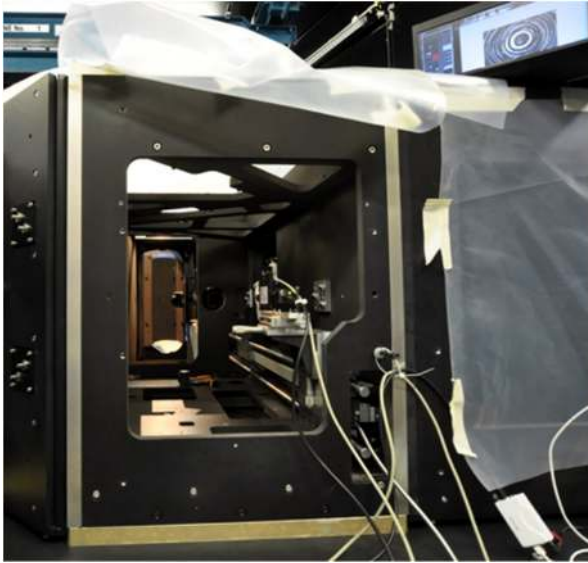
Fig. 6 View through the spine. Point source microscope in position to align collimator optics.
