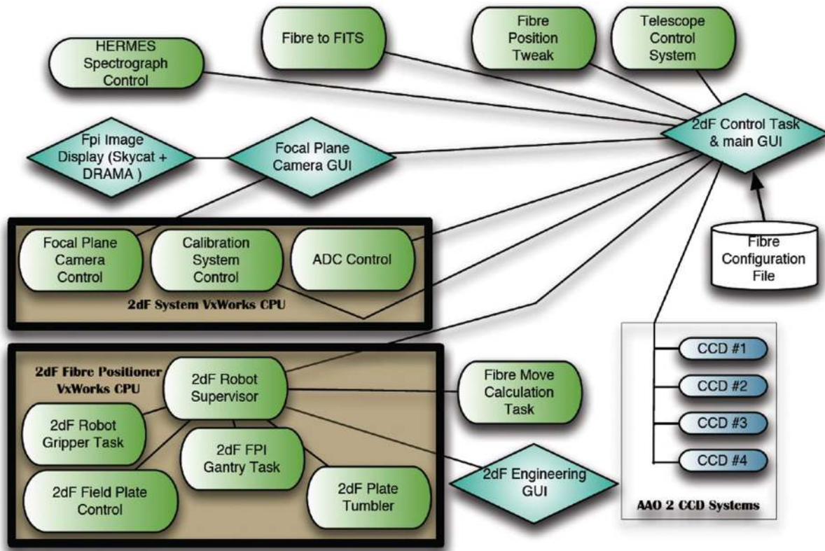
Fig. 21 Schematic overview of the HERMES electronics systems.
