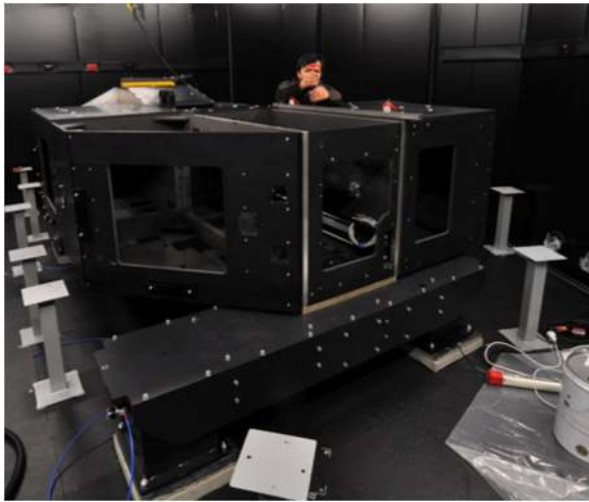
Fig. 2 HERMES structure nearing final assembly. IR box removed to allow collimator alignment.
