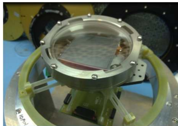
Fig. 18 The detector assembly with the field lens mounted (before blackening).
