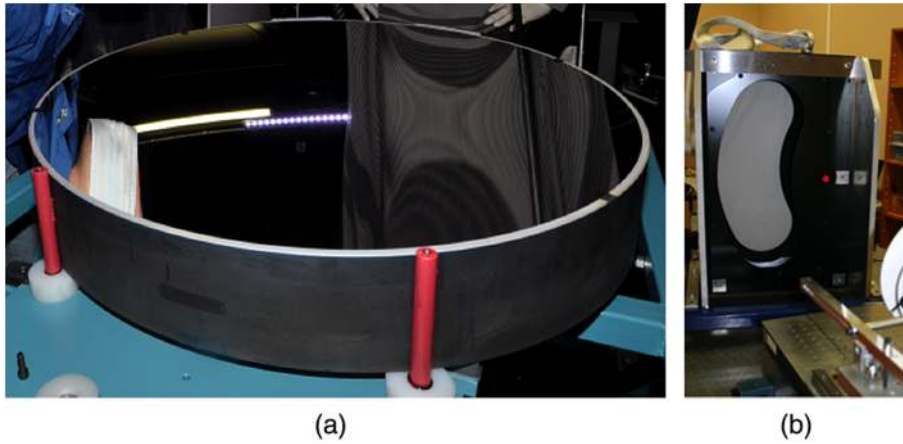
Fig. 15 (a) The HERMES collimator mirror and (b) corrector lens. The corrector lens is shown during acceptance testing, lenses are baffled to the elongated and curved clear aperture 540 mm long and 200 mm wide. Red dot identifies the location of the optical axis of the spectrograph on the corrector lens cell.
