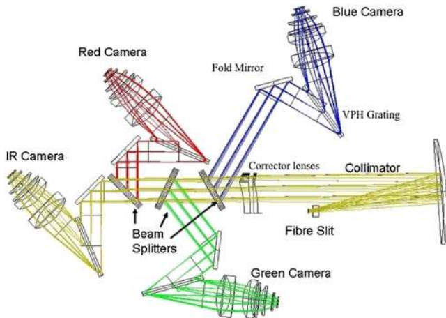
Fig. 13 Optical layout of the HERMES spectrograph. Fold mirrors are used to insure that the design is compact, free of physical interferences, and for serviceability issues such as allowing the Dewars for all four arms to be external to the enclosure.
