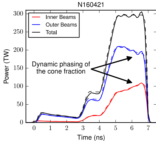
Figure 2: The laser pulse shape used in the initial liquid layer experiments requires <900\text{kJ} , less than half of the full NIF capability (dashed is the requested pulse; solid is the actual delivered pulse).
