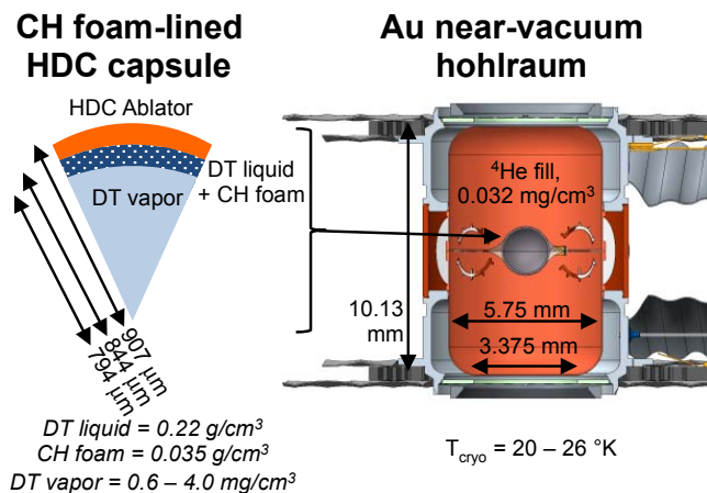
Figure 1: Illustration of the capsule and hohlraum used in the liquid layer experiments. The HDC shell thickness is 63 \mu\text{m} and outer radius is 907 \mu\text{m} .
