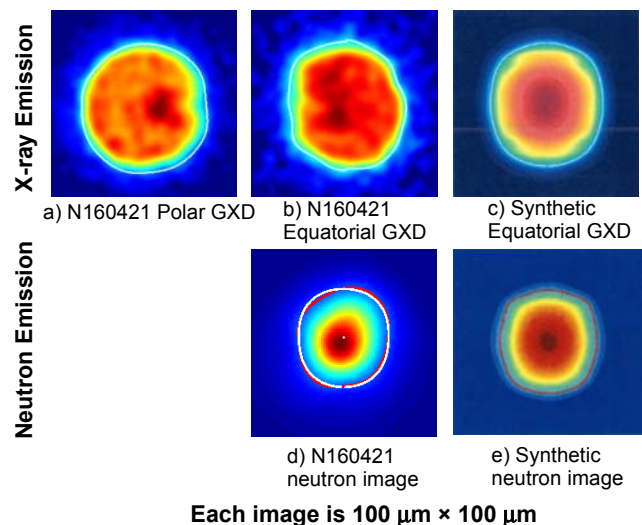
Figure 3: a) polar x-ray image of hot spot at bang time; b) equatorial x-ray image; c) synthetic x-ray image from simulation; d) neutron image of the hotspot; e) synthetic neutron image from simulation.
