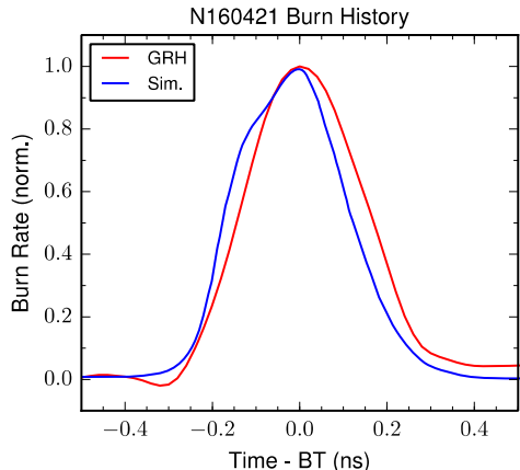
Figure 4: Thermonuclear burn history measurement compared to burn history in simulation. Time (ns) is in relation to bang time (BT).
