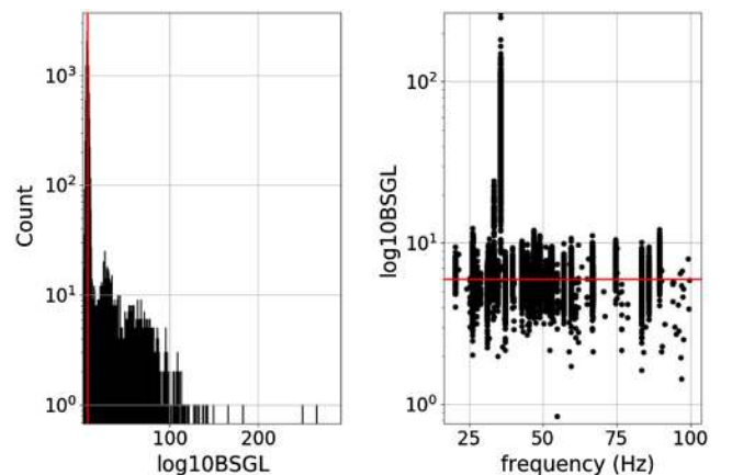
FIG. 8. Detection statistic of the loudest candidate from each stage 2 search: the distribution of their detection statistic values \hat{\beta}_{S/GL} (left) and their distribution as a function of frequency (right). The red line marks \hat{\beta}_{S/GL} = 6.0 which is the threshold at and above which candidates are passed on to stage 3.
