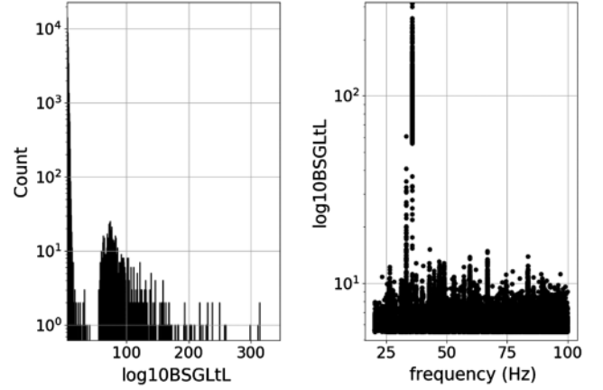
FIG. 6. Candidates that are followed up in stage 1: the distribution of their detection statistic values \hat{\beta}_{S/GLIL} (left) and their distribution as a function of frequency (right).
