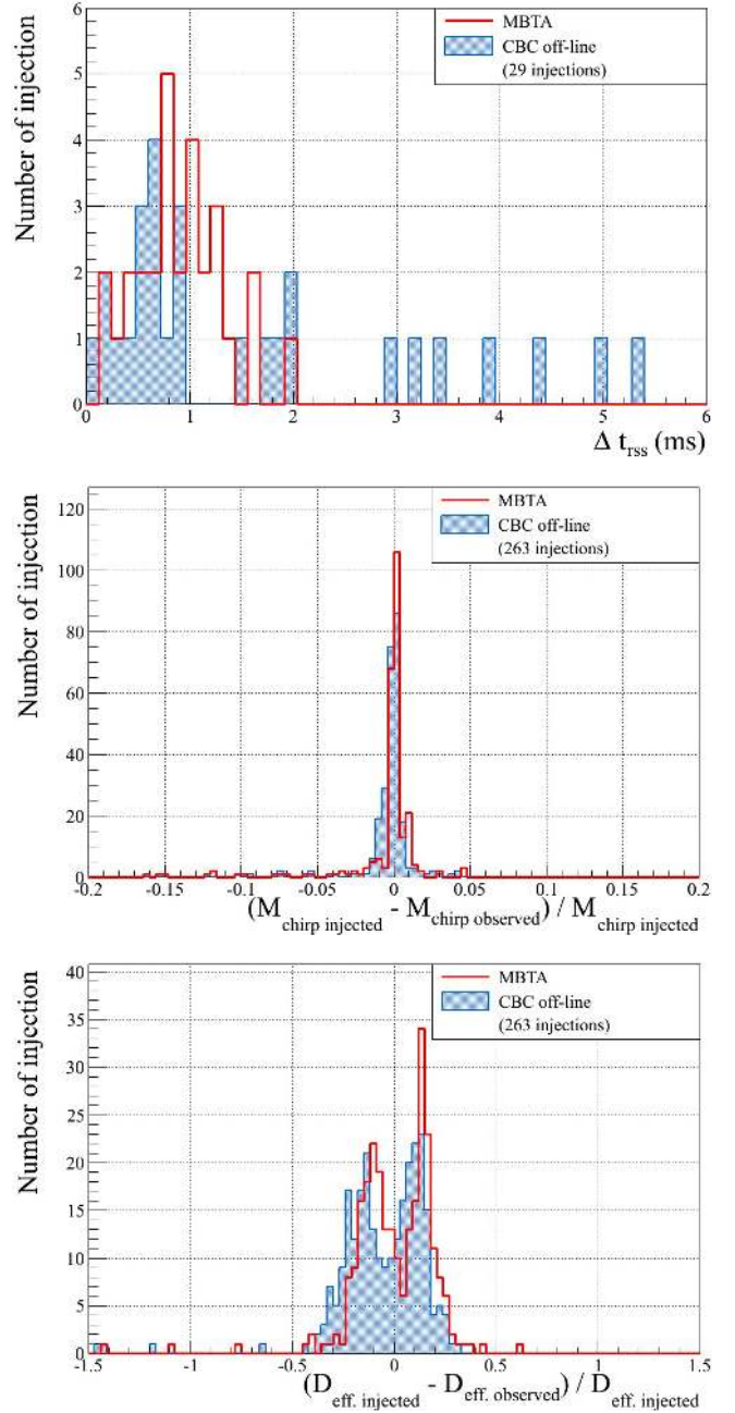
Fig. 8. These plots show the differences between the parameters of the hardware injections and those of the triggers found by both MBTA and the offline iHope pipeline. The first plot shows the timing accuracy parameter \Delta t_{\text{rss}} of all triple coincidences. The second plot corresponds to the difference between the chirp mass of the binary injected and observed. The third one corresponds to the difference between the effective distance of the binary injected and reconstructed by MBTA. The second and third plots contain all the hardware injections observed in H1, L1 or V1.
