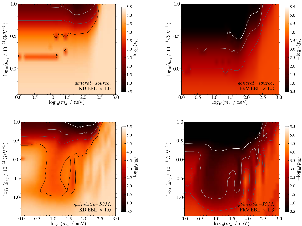
Figure 2. Significance map for the photon-ALP conversion in the (m_a, g_{a\gamma}) plane. Smaller values (brighter regions) indicate less accordance between the model and the data. Upper panel: p_t values for the general source -scenario, shown as -\log_{10}(p_t) . Lower panel: p_{95} values for the optimistic ICM case. For each pixel, 5000 realizations of the random magnetic field are simulated and p_{95} is determined from the resulting 5000 p_t values (cf. Sec. IV). In the left column, the attenuation due to the interaction of VHE \gamma -rays with the EBL is given by the KD model, whereas in the right column the FRV model is utilized. The maps are smoothed using a bilinear interpolation between the single (m_a, g_{a\gamma}) pixels.
