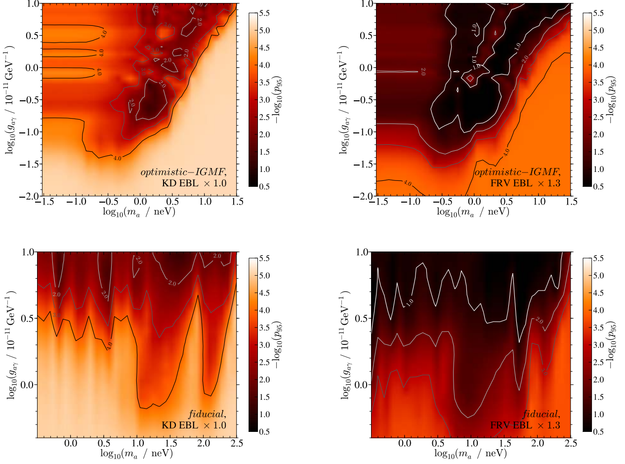
Figure 3. Significance maps for the photon-ALP-conversion. Same as the bottom row in Fig. 2, but for the optimistic IGMF -scenario (top row) and fiducial -case (bottom row).
