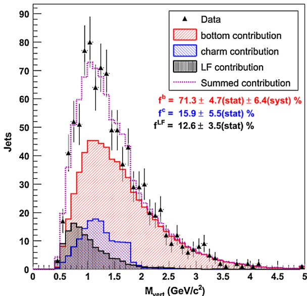
FIG. 2 (color online). Maximum likelihood fit of the vertex mass for tagged jets in the selected data sample.
