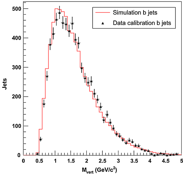
FIG. 1 (color online). Comparison of the vertex mass distributions of tagged b jets from a simulated sample and from data.
