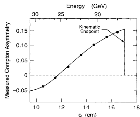
FIG. 1. The average polarized Compton scattering asymmetry as measured by seven channels of the Cherenkov detector is plotted as a function of the distance ( d ) from the trajectory of the undeflected beam. The curve represents the product of the asymmetry function and a normalization factor that has been adjusted to achieve a best fit to the measurements.
