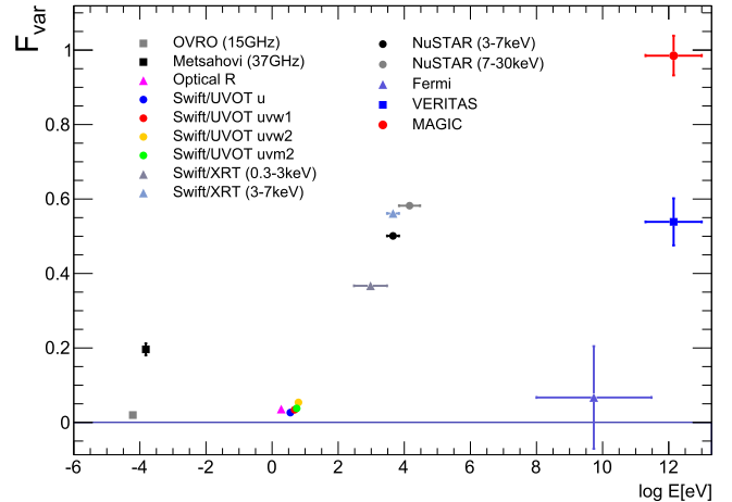
Figure 9. Fractional variability ( F_{\text{var}} ) calculated for each instrument separately.
