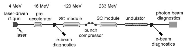
FIG. 1. Schematic layout of phase 1 of the SASE FEL at the TESLA Test Facility at DESY, Hamburg. The linac contains two 12.2 m long cryogenic modules each equipped with eight 9-cell superconducting accelerating cavities [20]. The total length is 100 m.
