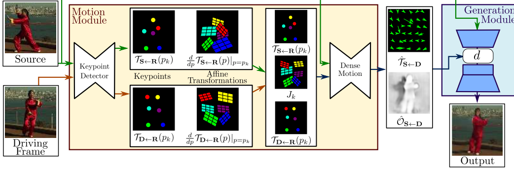
Figure 2: Overview of our approach. Our method assumes a source image S and a frame of a driving video frame D as inputs. The unsupervised keypoint detector extracts first order motion representation consisting of sparse keypoints and local affine transformations with respect to the reference frame R . The dense motion network uses the motion representation to generate dense optical flow \hat{\mathcal{T}}_{S \leftarrow D} from D to S and occlusion map \hat{\mathcal{O}}_{S \leftarrow D} . The source image and the outputs of the dense motion network are used by the generator to render the target image.
