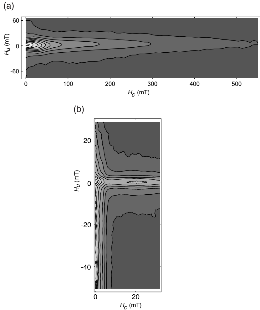
Figure 4. (a) FORC diagram for the red-bed sample 90-VAU-42 ( t_m = 0.7 s). (b) High-resolution FORC diagram for the lower left-hand portion of the FORC plane for the red-bed sample ( t_m = 1 s; SF = 3 ).
