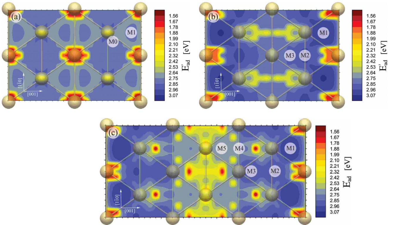
FIG. 3. (Color online) Potential-energy surfaces of (a) the O/Au(110)- (1 \times 1) surface ( \Theta=0.081 \text{ \AA}^{-2} , 2 \times 2 SUC), (b) the missing row-reconstructed O/Au(110)- (1 \times 2) surface ( \Theta=0.041 \text{ \AA}^{-2} , 2 \times 2 SUC), and (c) the missing row type reconstructed O/Au(110)- (1 \times 3) surface ( \Theta=0.027 \text{ \AA}^{-2} , 2 \times 3 SUC). The SUCs are defined in Fig. 1. The adsorption energies E'_{\text{ad}}=E_{\text{ad}}+\frac{1}{2}E_{b,\text{O}_2} , related to atomic oxygen, calculated for 35 sites in the case of Au(110)- (1 \times 1) , for 65 sites in the case of Au(110)- (1 \times 2) , and for 95 sites in the case of Au(110)- (1 \times 3) are color coded. Local adsorption energy maxima are denoted by M0, M1, \dots, M5 .
