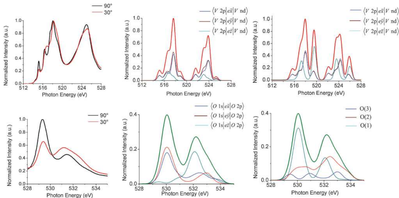
Fig. 9 Upper row: V L-edge single crystal spectra (left), B3LYP/def2-TZVP calculated V L-edge spectrum (red thick line) and transition dipole moments \langle V 2p|e\vec{x}|V nd\rangle for V_6O_{20}H_{10} (middle) and V_{10}O_{31}H_{12} (right). Bottom row: the corresponding calculated O K-edge single crystal spectra (left), and calculated spectra for V_6O_{20}H_{10} together with dipole transition moments \langle O 1s|e\vec{r}|O 2p\rangle (middle) and the individual O atoms contributions (right).
