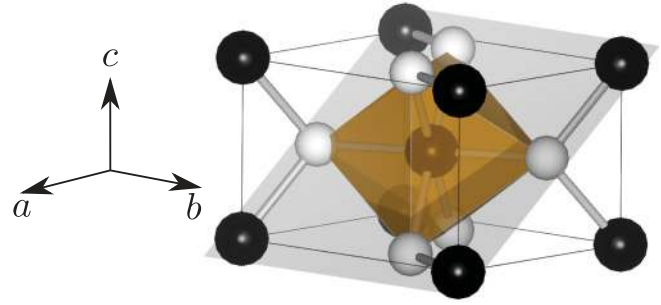
FIG. 2. (Color online) Unit cell of marcasite \text{FeS}_2 (rendered by VESTA 17 ). Black (white) spheres represent Fe (S) atoms. The (101) plane is highlighted in gray. The octahedra is edge-shared by the S atoms on the (001) faces.
