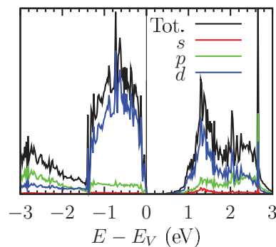
FIG. 17. (Color online) DOS of the lowest-energy pyrite (100)-marcasite (101) interface (corner-sharing, \theta = 270^\circ ) within the GGA-PBE. By comparing to Fig. 9, two key observations are made: (i) the band gap is not reduced; (ii) gap states are not found.
