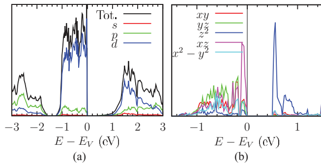
FIG. 9. (Color online) GGA-PBE DOS of pyrite (a) bulk, (b) (100) surface. In (a), both the total DOS and s - p - d decomposed DOS are shown. The CB and VB are dominated by Fe d states. We have verified that these d states within the CB and VB are e_g and t_{2g} , respectively. Due to the presence of an S p state, the CB tail extends to 0.4 eV above the VB edge. In (b), the DOS of d orbitals are shown to identify the character of intrinsic surface states. The intrinsic surface state appears at the CB edge, not within the band gap, and is of d_{z^2} character. However, ligand field splitting in the VB is not observed and d_{xy} surface states are not found, contrary to the prediction of Bronold and co-workers. 5
