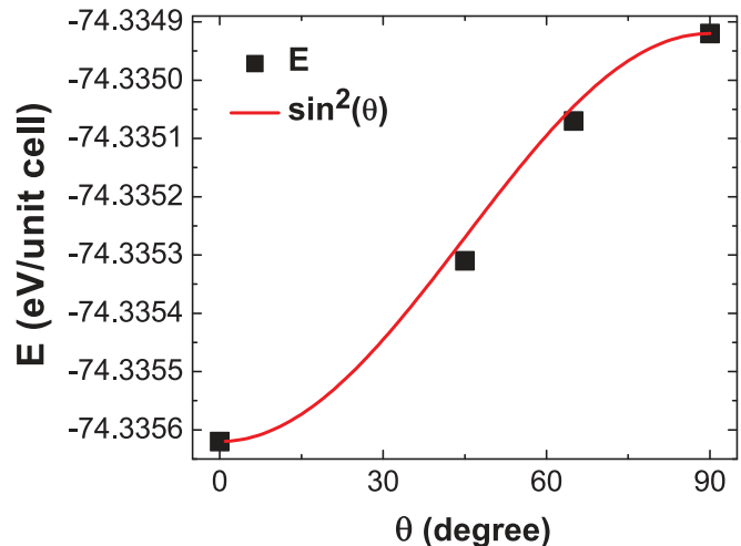
FIG. 2. (Color online) Angular dependence of the magnetic energy, where \theta is the angle between the magnetization direction and the normal to the interface plane.
