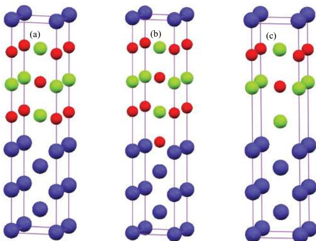
FIG. 1. (Color online) Schematics of the calculated crystalline structures for (a) pure, (b) overoxidized, and (c) underoxidized geometries. Fe, Mg, and O are represented by blue, green, and red balls, respectively.
