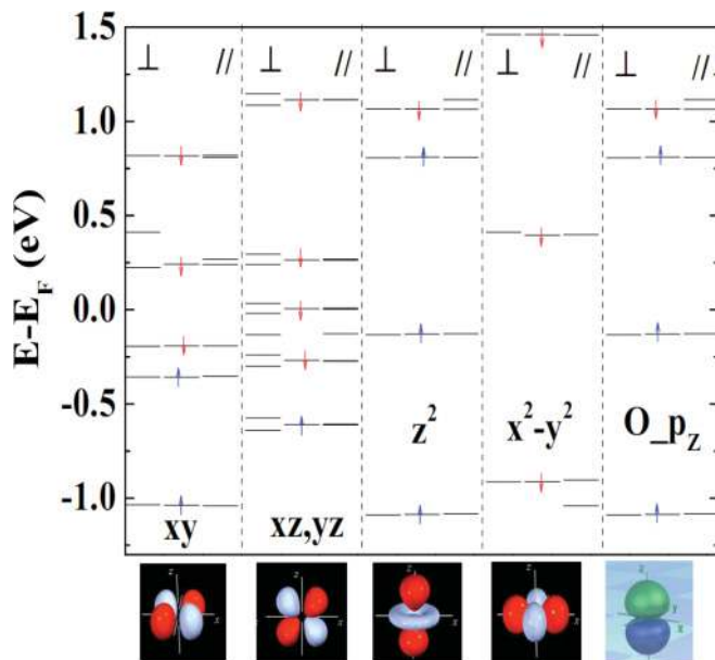
FIG. 4. (Color online) The same as Fig. 3, for an overoxidized Fe|MgO interface.
