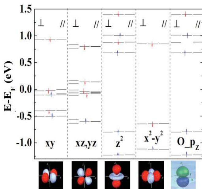
FIG. 5. (Color online) The same as Fig. 3, for an underoxidized Fe|MgO interface.
