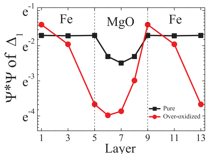
FIG. 6. (Color online) \Delta_1 Bloch state character at the \Gamma point around the Fermi level as a function of layer number in the pure and overoxidized Fe|MgO interfaces shown in Figs. 1(a) and 1(b), respectively. The \Delta_1 Bloch state is absent around the Fermi level in the underoxidized case shown in Fig. 1(c).
