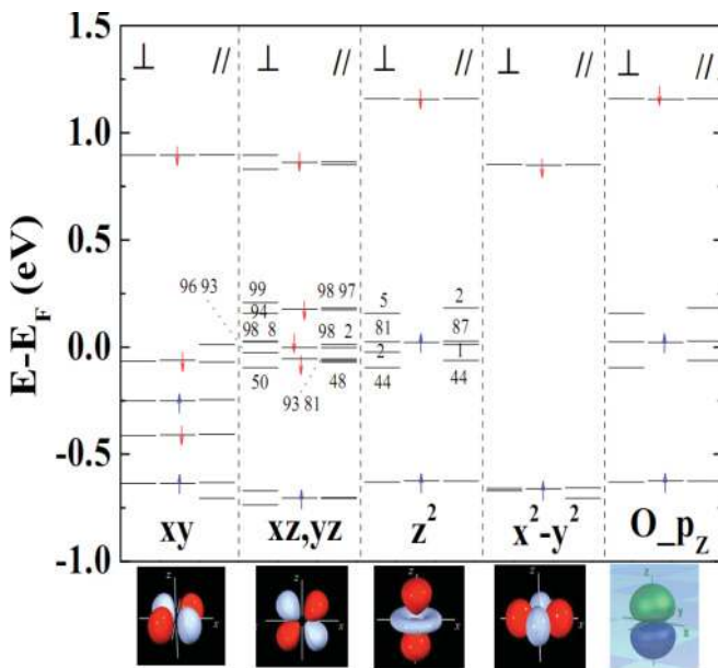
FIG. 3. (Color online) Spin-orbit coupling effects on wave function character at the \bar{\Gamma} point of interfacial Fe d and neighbor oxygen p_z orbitals for the pure Fe|MgO interface shown in Fig. 1(a). The three subcolumns in each column show the band levels for out-of-plane (left) and in-plane (right) orientations of magnetization as well as for the case with no spin-orbit interaction included (middle). Numbers are the percentage of orbital character components within Wigner-Seitz spheres around interfacial atoms.
