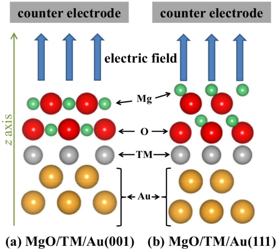
Fig. 1. (Color online) Schematic diagram of (a) MgO/TM/Au(001) and (b) MgO/TM/Au(111) systems where TM=Fe, Co. The system consists of the MgO insulating layer, the TM monolayer, and the Au substrate. The electric field is applied by introducing the counter electrode far above the system. The direction of the electric field is defined in such a way that a positive (negative) electric field decreases (increases) the number of electrons in the system, pointing upward (downward) along the positive (negative) z axis direction.
