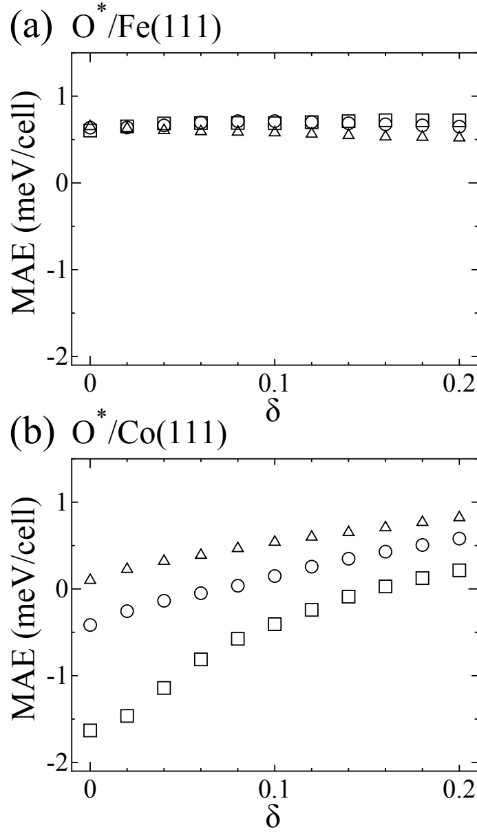
Fig. 3. Magnetic anisotropy energy, MAE, as a function of the oxidation number \delta of the TM atom (TM=Fe, Co) in (a) O*/Fe(111) and (b) O*/Co(111) bilayer systems with the lattice constant taken to match the Au(111) substrate, a=2.88 \text{ \AA} , and the interlayer distance fixed at d=2.0 \text{ \AA} . The triangles, the circles, and the squares represent the results for \Delta N=-0.1 , 0.0 , and 0.1 , respectively. The electric field is given by -0.252 \Delta N \times 10^3 \text{ V/nm} with the definition that a positive (negative) electric field decreases (increases) the number of electrons in a system.
