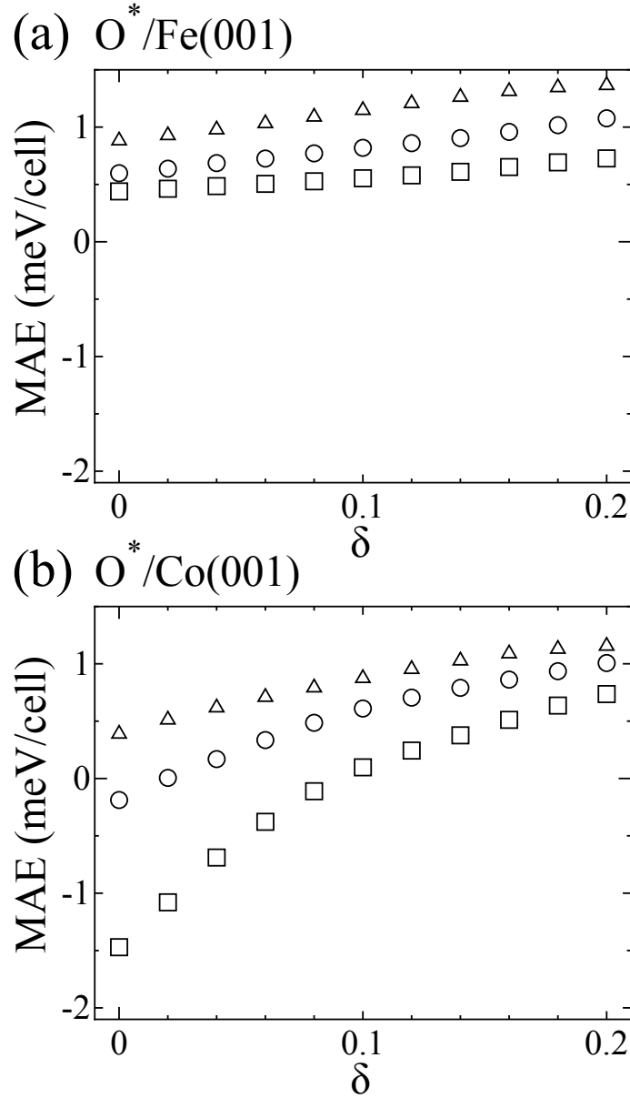
Fig. 2. Magnetic anisotropy energy, MAE, as a function of the oxidation number \delta of the TM atom (TM=Fe, Co) in (a) O^*/Fe(001) and (b) O^*/Co(001) bilayer systems with the lattice constant taken to match the Au(001) substrate, a=2.88 \text{ \AA} , and the interlayer distance fixed at d=2.0 \text{ \AA} . The triangles, the circles, and the squares represent the results for \Delta N=-0.1, 0.0, and 0.1, respectively. The electric field is given by -0.218 \Delta N \times 10^3 \text{ V/nm} with the definition that a positive (negative) electric field decreases (increases) the number of electrons in a system.
