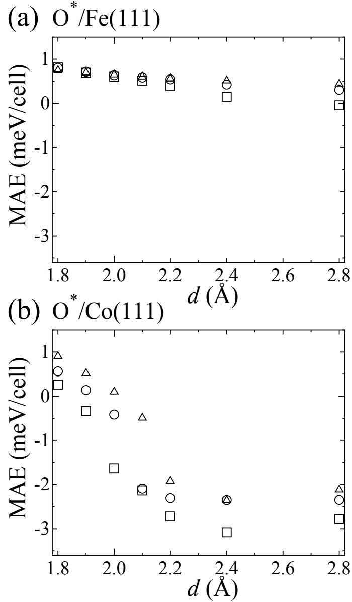
Fig. 5. Magnetic anisotropy energy, MAE, as a function of the distance d between the O* and TM (TM=Fe, Co) layers in (a) O*/Fe(111) and (b) O*/Co(111) bilayer systems with the lattice constant taken to match the Au(111) substrate, a=2.88 Å, and the oxidation number of the TM atom fixed at \delta=0.0 . The triangles, the circles, and the squares represent the results for \Delta N=-0.1 , 0.0, and 0.1, respectively. The electric field is given by -0.252 \Delta N \times 10^3 V/nm with the definition that a positive (negative) electric field decreases (increases) the number of electrons in a system.
