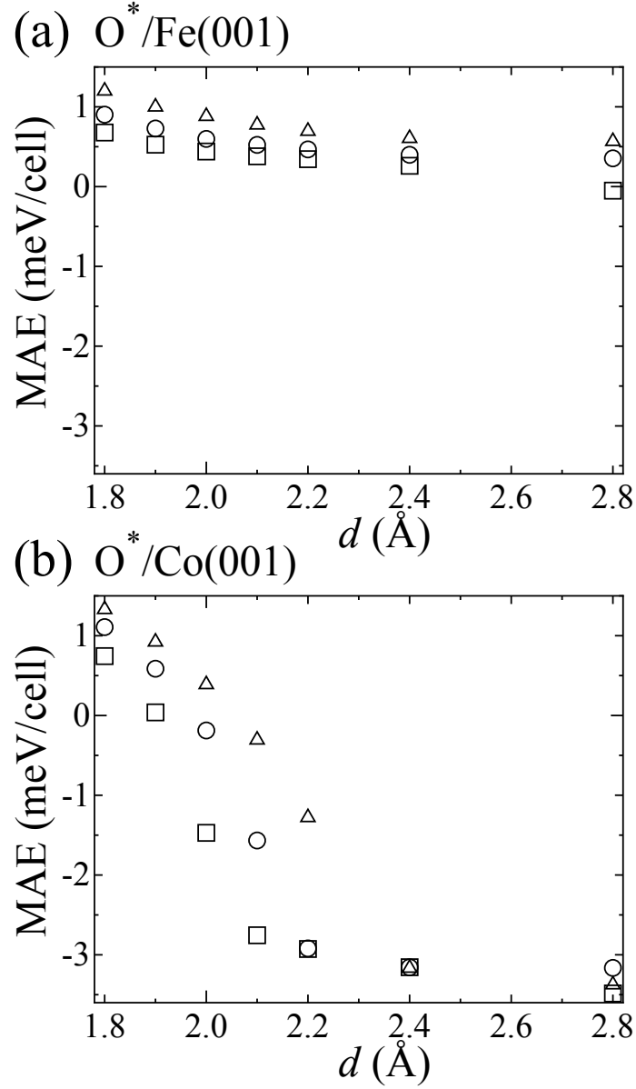
Fig. 4. Magnetic anisotropy energy, MAE, as a function of the distance d between the O* and TM (TM=Fe, Co) layers in (a) O*/Fe(001) and (b) O*/Co(001) bilayer systems with the lattice constant taken to match the Au(001) substrate, a=2.88 Å, and the oxidation number of the TM atom fixed at \delta=0.0 . The triangles, the circles, and the squares represent the results for \Delta N=-0.1 , 0.0, and 0.1, respectively. The electric field is given by -0.218 \Delta N \times 10^3 V/nm with the definition that a positive (negative) electric field decreases (increases) the number of electrons in a system.
