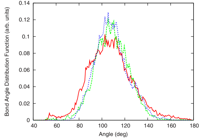
FIG. 3. (Color online) The Si-Si-Si bond angle distribution of three structures prepared by fast (solid red line), normal (dashed green line), and slow (dotted blue line) cooling rates (sample A).
