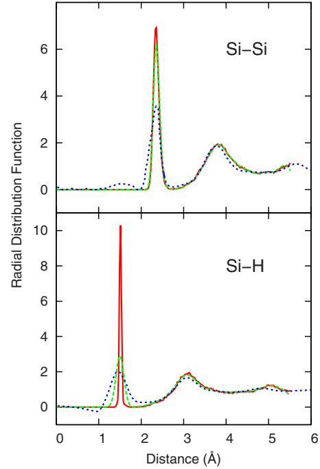
FIG. 6. (Color online) Partial radial distributions averaged over 500 MD configurations (red solid line), calculated radial distributions with quantum corrections (dashed green line), and neutron-scattering measurements (blue dotted line) (Ref. 28). Both types of calculated curves are averages over five slow quench samples. All curves refer to systems at 300 K.
