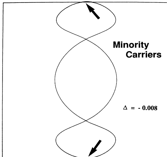
FIG. 13. Influence of the \Delta parameter on the Fermi surface. Minority carriers are obtained when the value of the \Delta parameter is increased to the experimental value of Dresselhaus (Refs. 1 and 24). This cut is the intersection between the Fermi surface and the plane containing the c axis and perpendicular to the K - \Gamma direction.
