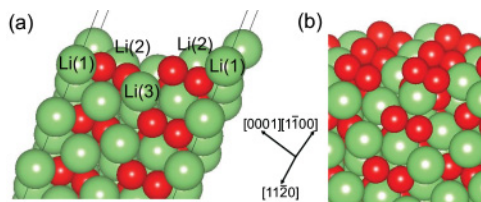
FIG. 5. (Color online) (a) The surface unit cell and (b) the relaxed structure of the most stable termination of the (1\bar{1}01) surface. Red and green atoms are oxygen and lithium, respectively.
