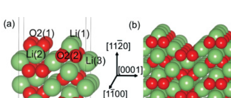
FIG. 2. (Color online) (a) The surface unit cell and (b) the relaxed structure of the most stable termination of the (11 \bar{2} 0) surface. Red and green atoms are oxygen and lithium, respectively.
