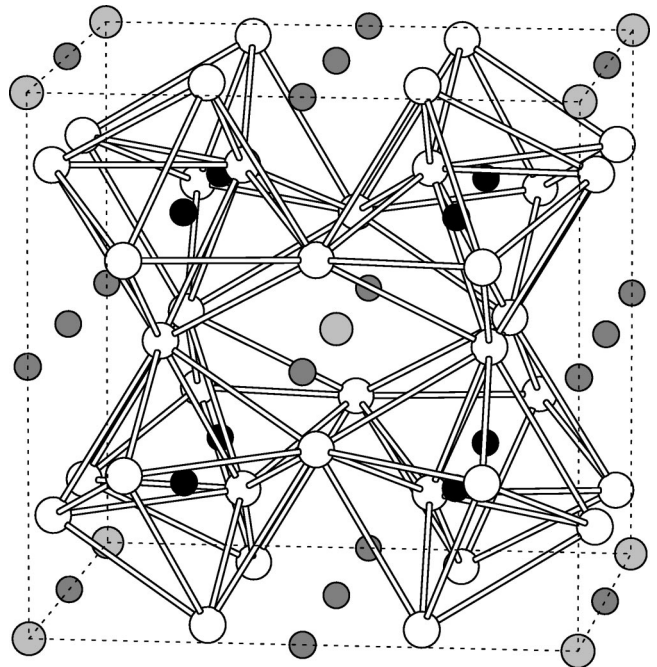
FIG. 1. Structure of \text{CaCu}_3\text{Ti}_4\text{O}_{12} (CCTO), showing tilted oxygen octahedra. White, light, dark, and black atoms are O, Ca, Cu, and Ti, respectively. Dashed lines indicate 40-atom primitive cell of antiferromagnetic spin structure.
