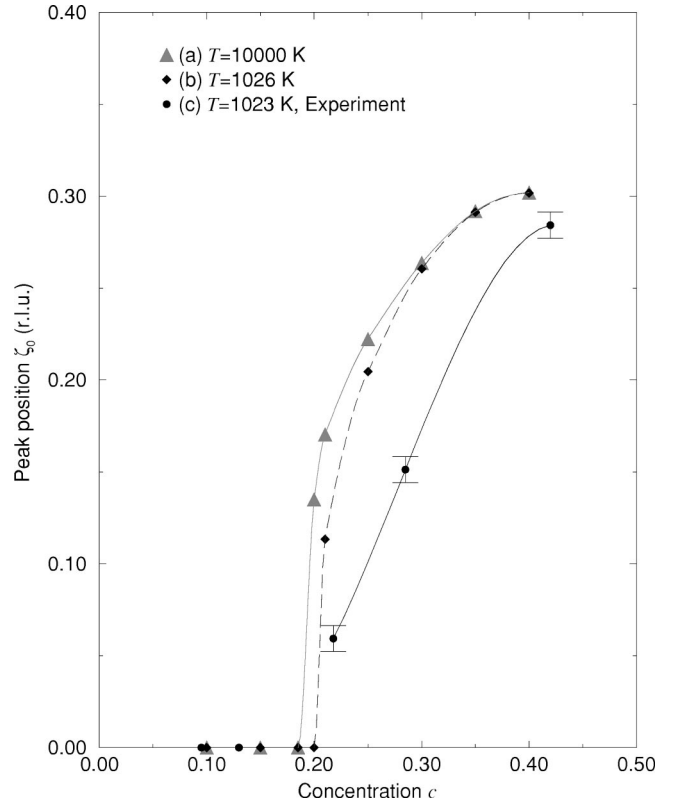
FIG. 6. The dependence of the peak position \zeta_0 of \alpha_{\mathbf{k}} with respect to the concentration c calculated for disordered fcc \text{Cu}_{1-c}\text{Pd}_c alloy at (a) T=10\,000 K and (b) T=1026 K. (c) Experimental data (Ref. 7).
