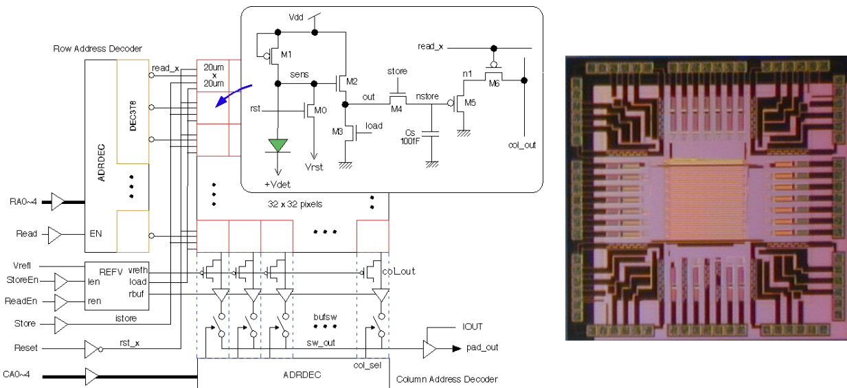
Fig. 5. Block diagram (left) and photograph (right) of the pixel detector. Pixel size is 20 \mu\text{m} by 20 \mu\text{m} , arranged into a 32 x 32 array of pixels. Chip size is 2.5 mm by 2.5 mm.
