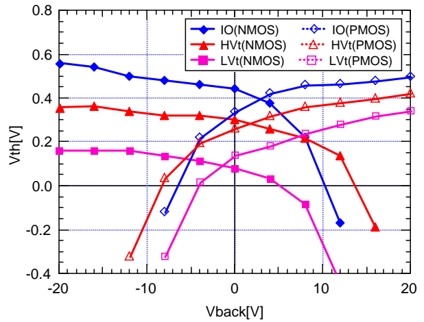
Fig. 8. Measured threshold Voltage ( V_{th} ) shifts due to back gate voltage ( V_{back} ) for NMOS and PMOS transistors of the three different types available.
