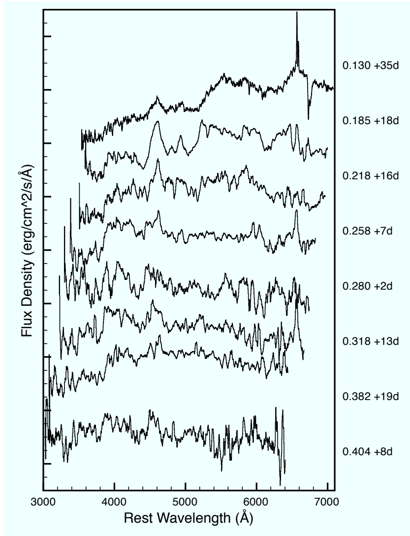
Fig. 3.— A sample of observed Ia spectra from the Fall 2005 run with significant host-galaxy contamination. All spectra have been shifted to the rest frame (numbers at right give the redshifts and epochs relative to B -band maximum) and have been normalized for display purposes. The top spectrum (from Subaru) has not been corrected for telluric absorption.
