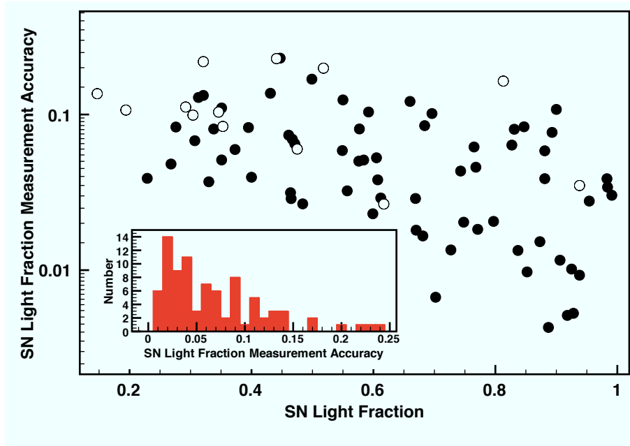
Fig. 7.— The accuracy of the SN component measurement (defined as the statistical error of SN light flux divided by the fraction of SN light flux) plotted vs. SN fraction. “Type Ia?” (empty circles) tend to have relatively low accuracy. In most cases, the SN fraction is measured to within < 10\% .
