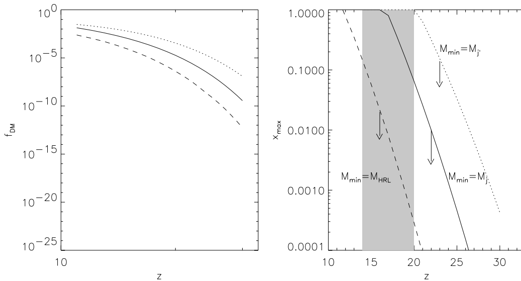
FIG. 10.— Left : Fraction of the universe in bound objects with mass greater than M^{\text{HRL}} (dashed line), M^{\text{J}} = 10^6 M_{\odot} (solid line), and M^{\text{J}^i} (dotted line) in a model with a running spectral index. The curves were computed for the 1\sigma upper limit parameters for this model (see Fig. 9). These should be viewed as upper limits on the mass fraction in collapsed objects. Right : Ionization fraction as a function of redshift and is based on the assumptions described in § 4.7. As in the left panel, we use the 1\sigma upper limit estimate of the power spectrum so that we obtain “optimistic” estimates of the reionization fraction. In the context of a running spectral index fit to the data, the WMAP detection of reionization appears to require that \text{H}_2 cooling played an important role in early star formation.
