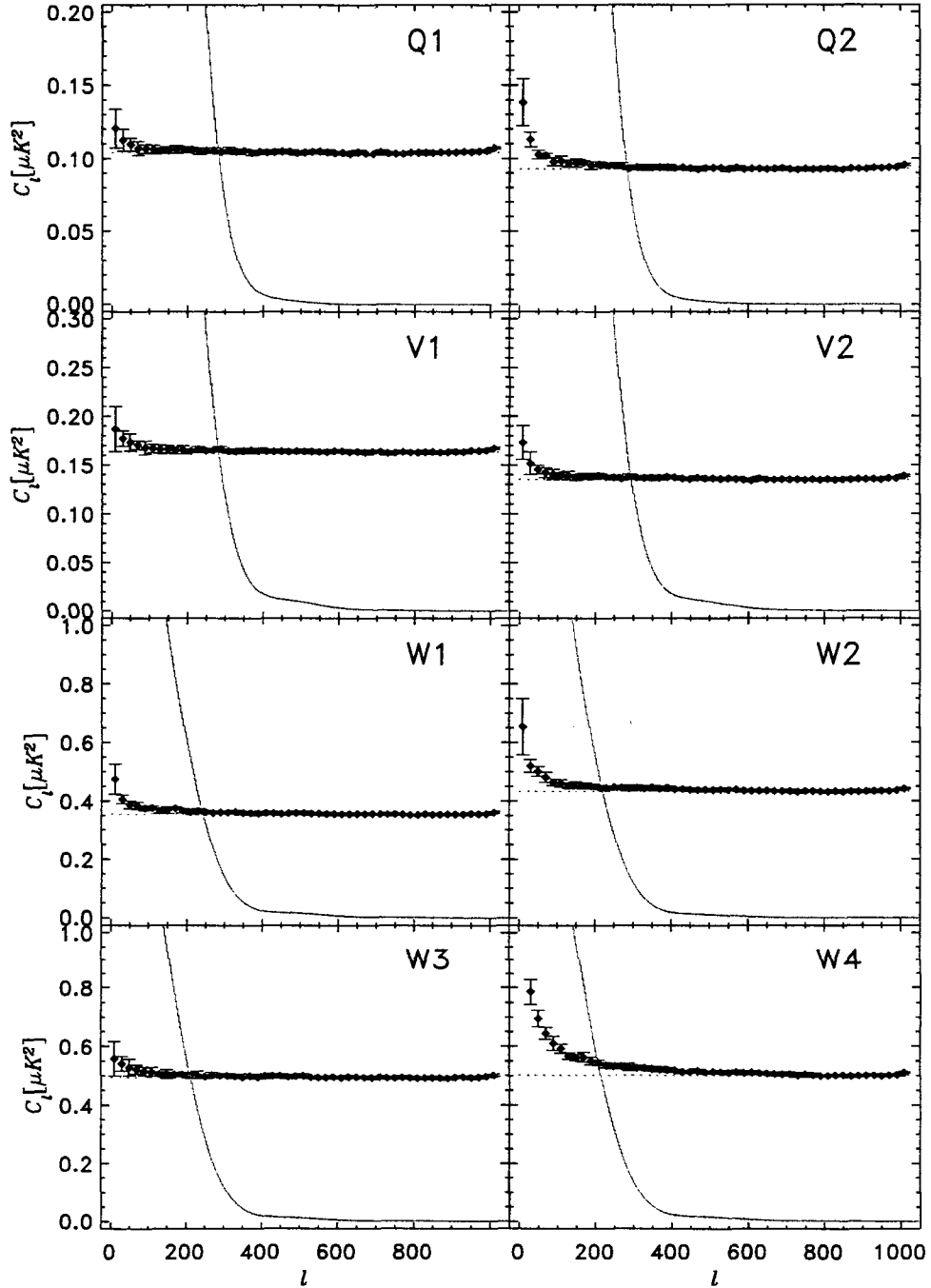
Fig. 1.— The effective noise as a function of l for the 8 differencing assemblies used in the combined power spectrum analysis. These spectra were computed from end-end simulations of noise maps, as discussed in §2.2. For illustration, the spectra shown here were computed using the quadratic estimator with uniform pixel weights. The actual noise model uses three separate weighting schemes in three separate l ranges, and thus has discontinuities where the effective noise level changes. The weights are defined in Appendix A.1.2.
