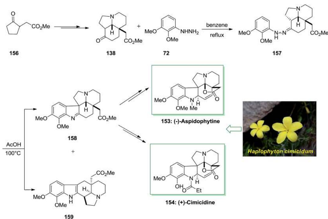
Scheme 31 Total synthesis of (-)-aspidoptytine 153 and (+)-cimicidine 154.
