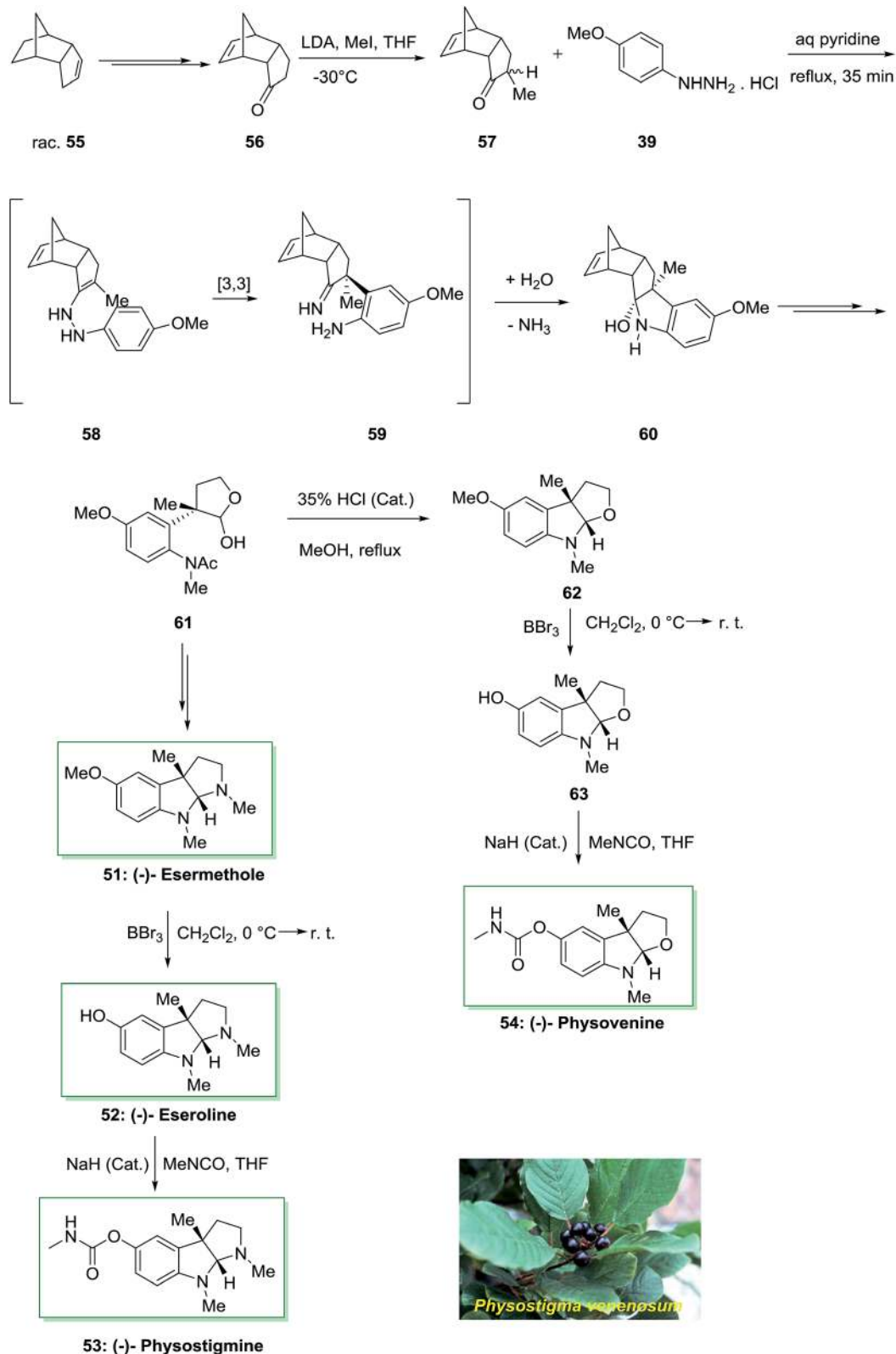
Scheme 9 Total synthesis of (–)-esermethole 51 , (–)-eseroline 52 , (–)-physostigmine 53 and (–)-physoveneine 54 .
