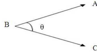
Fig. 2: The angle between two vectors
