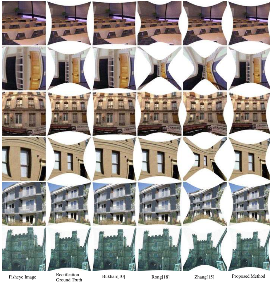
Fig. 3. Qualitative results on our synthesized datasets. From left to right, we show the input, the ground truth, results of three state of the art methods ([10, 15, 18]), and the result of our proposed approach. Our method achieves the best overall visual quality of all the compared methods.
