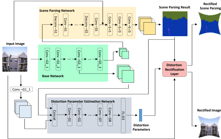
Fig. 2. The overview of the proposed joint network architecture. This composite architecture consists of four cooperative components: a base network, a distortion estimation network, a distortion rectification layer, and a scene parsing network. The distortion parameter estimation network takes as input a concatenation of multiple feature maps from the base network and generates corresponding distortion parameters. Meanwhile, the scene parsing network extracts high-level semantic information to further improve the accuracy of distortion parameter estimation as well as rectification. The estimated parameters are then used by the distortion rectification layer to perform rectification on both the input fisheye image and the corresponding scene parsing results.
