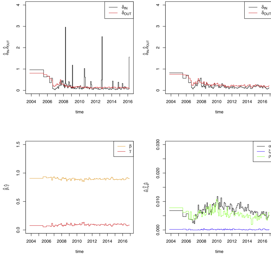
FIG 6.2. Local parameter estimates of the linear preferential attachment model for the full and reduced Wiki talk network. Upper left: (\hat{\delta}_{in}, \hat{\delta}_{out}) for the full network. Upper right, lower left, lower right: (\hat{\delta}_{in}, \hat{\delta}_{out}) , (\hat{\beta}, \hat{\gamma}) , (\hat{\alpha}, \hat{\xi}, \hat{\rho}) for the reduced network, respectively.
