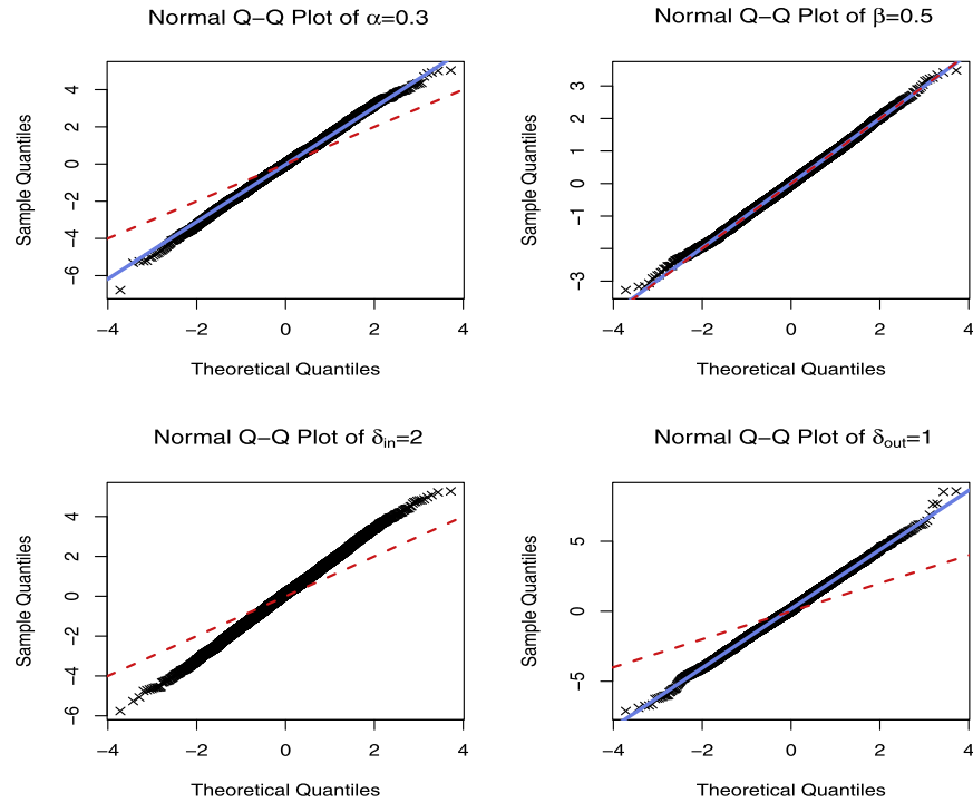
FIG 5.2. Normal QQ-plots for the normalized estimates in (5.3) under 5000 replications of a preferential attachment network with 10^5 edges and \theta = (0.3, 0.5, 2, 1) . The fitted lines in blue are the traditional qq-lines used to check normality of the estimates. The red dashed line represents the y = x line in all plots.
