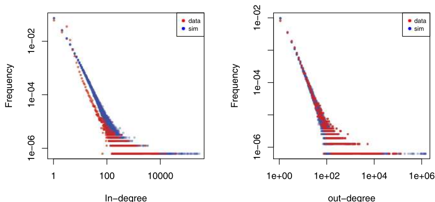
FIG 6.4. Empirical in- and out-degree frequencies of the full Wiki talk network (red) and that from 20 realizations of the linear preferential attachment network with fitted parameter values (6.3) from the snapshot estimator (blue).
