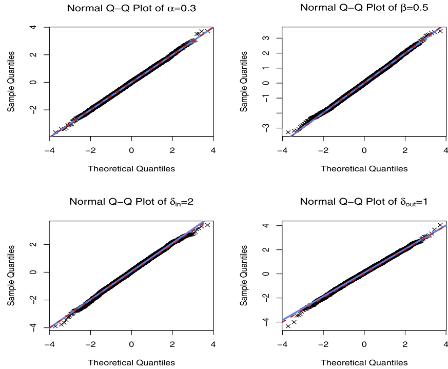
FIG 5.1. Normal QQ-plots in black for normalized estimates in (5.2) under 5000 replications of a preferential attachment network with 10^5 edges and \theta = (0.3, 0.5, 2, 1) . The fitted lines in blue are the traditional qq-lines (given by R ) used to check normality of the estimates. The red dashed line represents the y = x line in all plots.
