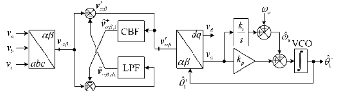
Fig. 29. Block diagram description of the CCF-PLL
