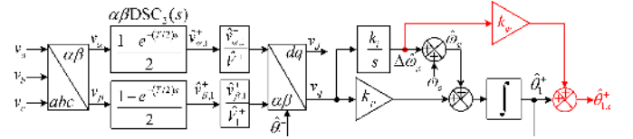
Fig. 15. \alpha\beta DSC -PLL with phase-error compensator (PEC).
