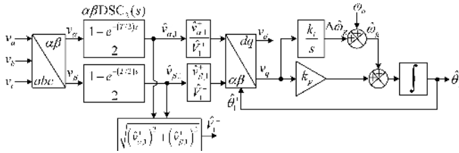
Fig. 14. Block diagram description of \alpha\beta DSC -PLL.
