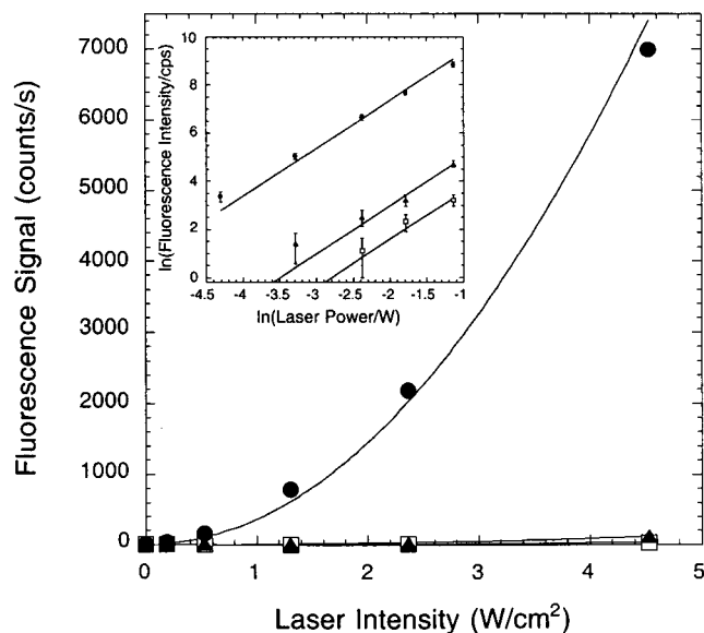
Figure 3. Laser power dependence of the two-photon-excited fluorescence intensity from a polymer/silver-cluster composite film (circles), neat polymer film (squares), and silver cluster film (triangles). Experiments were conducted using a 3 mm diameter collimated laser beam. Inset shows the same data on a double logarithmic plot. The solid lines are quadratic fits to the data.
