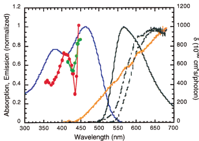
Figure 2. One-photon and two-photon spectra of polymer (A), composite, and metal cluster films. One-photon absorption spectrum of polymer in toluene solution (blue). Two-photon fluorescence excitation spectrum of polymer in toluene solution (femtosecond data in red, nanosecond data in green), calibrated against Coumarin 307 in methanol (ref 25) and plotted against half the excitation wavelength. One-photon-excited fluorescence spectrum of polymer in toluene solution (solid black line). Two-photon-excited emission spectra ( \lambda_{\text{exc}} = 800 nm) of the neat polymer film (dashed black line), the polymer/cluster composite film (dash-dotted black line), and the neat metal cluster film (orange).
