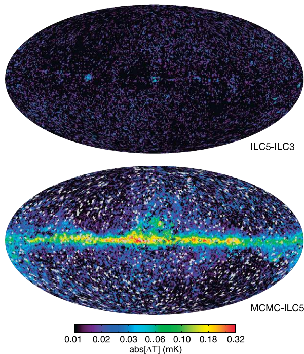
Figure 21. Difference maps between the 5 year and 3 year ILC maps (top), and the MCMC fit for the CMB and the 5 year ILC map (bottom). For the former, the most prominent large-scale difference is from the reduction of noise with WMAP ’s observational pattern. Even for the latter, the variance outside the KQ85 analysis mask is 116 \mu\text{K}^2 , lower than the CMB power at large scales.
