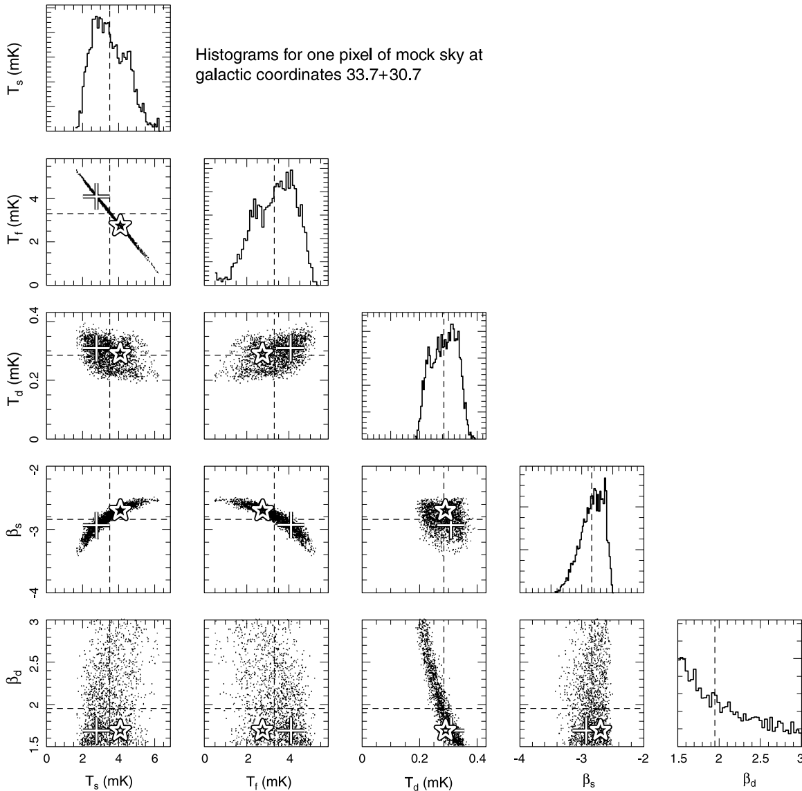
Figure 7. Histograms for foreground parameters for a single pixel of mock sky reconstruction. The mock foregrounds were designed to have the same statistical behavior as the true sky but do not match in detail. The same pixel is examined for the true sky in Figure 8. Dashed lines indicate the mean of the chain, crosses indicate the best-fit point, and stars indicate the input values for the parameters. The strong T_s – T_f degeneracy and the curved T_s – \beta_s degeneracy are typical for high S/N pixels. Other parameter correlations are minor. Both the mean and best-fit parameters of the chain are within the expected error range from the input values.
