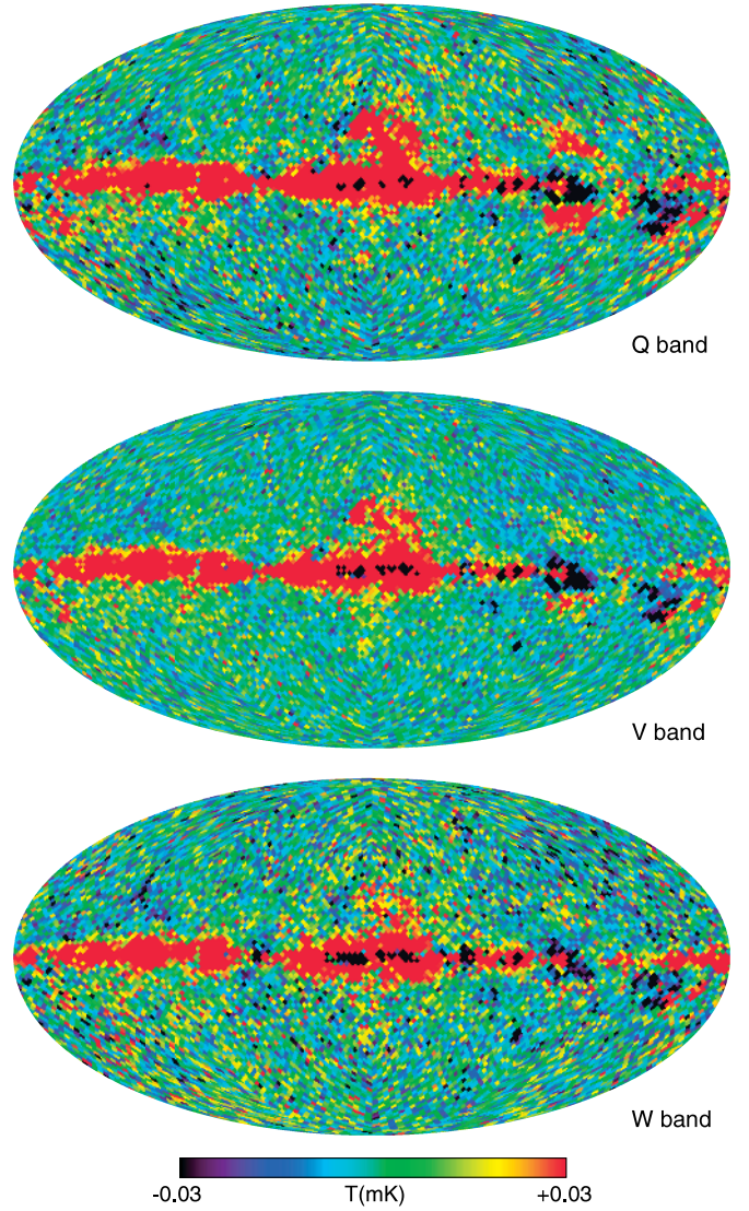
Figure 4. 5 year temperature maps with foregrounds reduced via template cleaning. All maps have had the 5 year ILC estimate for the CMB subtracted, and have been degraded to N_{\text{side}} = 32 . Frequency bands shown are Q, V, and W. Compare to Figure 10 of Hinshaw et al. (2007). Outside the Galactic mask, the template cleaning reduces foregrounds to \sim 15 \mu\text{K} or less.
