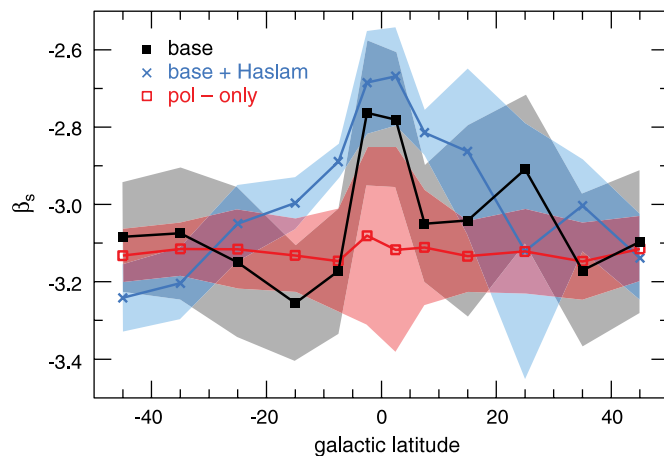
Figure 16. Synchrotron index plotted as a function of latitude for several fits. Pixels are binned by latitude, and only longitudes between 350^\circ and 10^\circ are included. Error regions indicate the 68% scatter within each bin. Solid black squares (gray region) are for the “base” model, blue crosses (blue region) are for the “base” model with 408 MHz data, and red empty squares (red region) are for a fit using only WMAP’s polarization data. Fits where the dust spectral index was fixed to 1.7 and 2.0 are almost identical to the “base” fit. The trend to a flatter spectral index in the plane does not appear when only polarization data are used, but the signal to noise is not high enough for the discrepancy to be significant.
