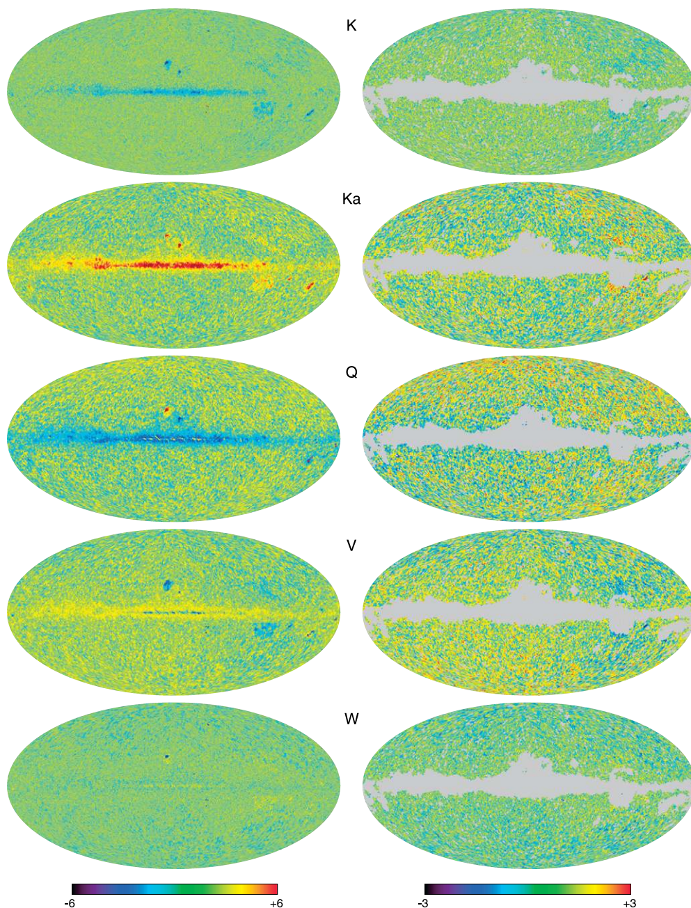
Figure 10. Residuals of the “base” model foreground fit subtracted from the data. The left column shows the residuals in units of noise sigma, from -6 to 6 . The right column has the 85% mask applied and a scale of -3 to 3 . Frequency bands are (from top to bottom) K, Ka, Q, V, W. The main feature is that the model underestimates Galactic flux in the Ka band and overestimates it in the Q band by a factor of 3–5 times the pixel noise. Outside the analysis mask, the residuals to the model are consistent with noise at the expected level.
