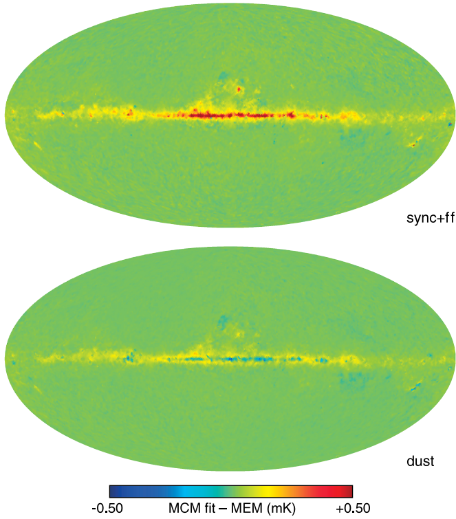
Figure 11. Difference between the MCMC fit and MEM maps. The top panel is the difference (at the K band) in synchrotron plus free–free emission. Differences between these two components separately are larger due to the degeneracy direction. The bottom panel is the difference (at the W band) in the dust maps. The differences are roughly 1% of total emission at the K band and a few percent at the W band.
