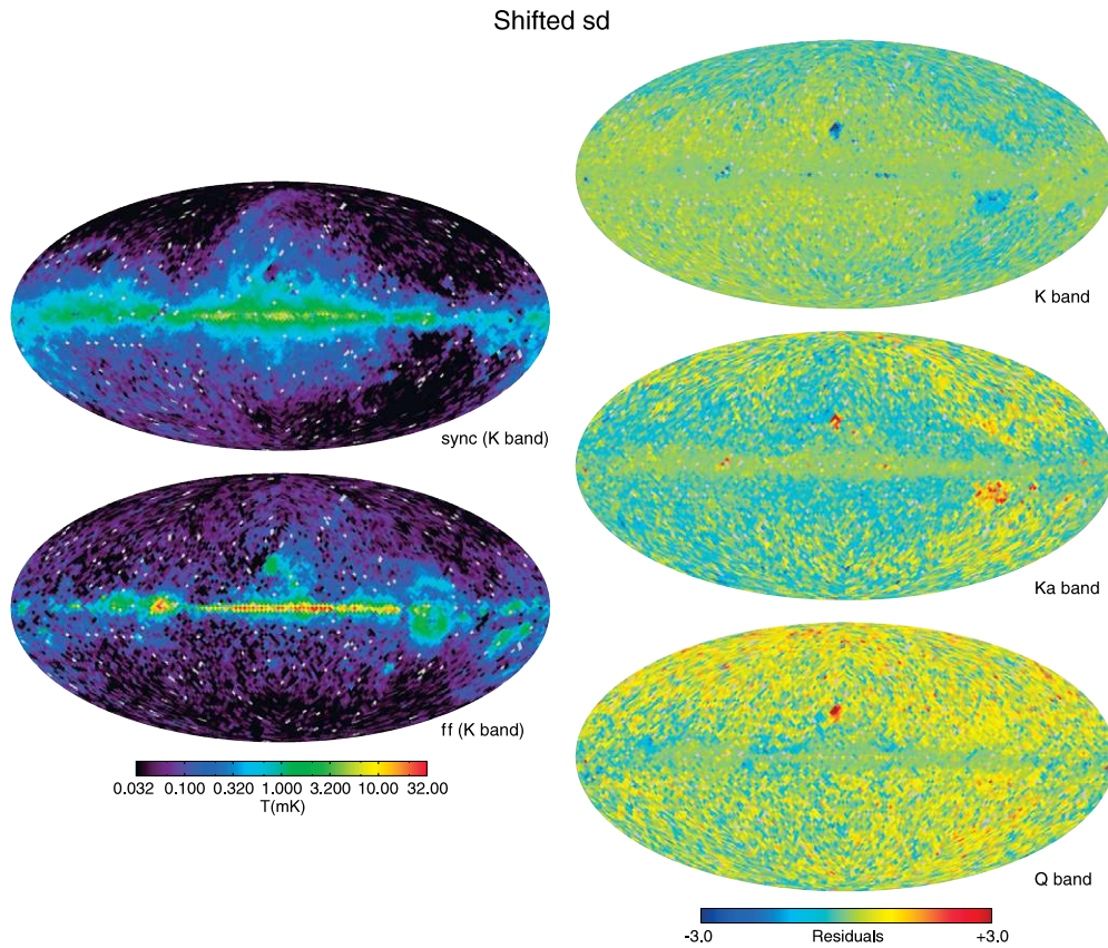
Figure 19. Foreground components and residual maps as determined by the MCMC fitting process for the “shifted sd” model. This model adds a spinning dust component (not required by the fit) at low frequencies where the peak emission frequency has been lowered in an attempt to match the data. Synchrotron and free-free temperatures are measured at the K band, and gray pixels are those masked due to point sources or flagged as problematic. The spinning dust component of the fit is shown in Figure 20. This model does not differ from the “base” model at high frequencies and thus the thermal dust emission is unaffected and not shown here. Left: synchrotron and free-free maps, right: residuals (in dimensionless units of noise sigma) to the fit at K, Ka, and Q bands.
