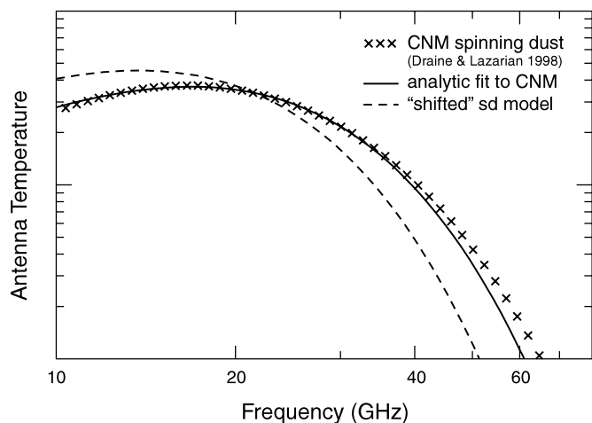
Figure 5. Exact CNM spinning dust spectrum as calculated by Draine & Lazarian (1998), an analytical fit to the model, and the ad hoc “shifted” model, which better fits radio observations in the Galactic plane. The shifted model may represent a mix of warm neutral medium and warm ionized medium models, or another emission process entirely. The vertical axis is in units of antenna temperature, but the overall scale is arbitrary. Agreement between the exact model and the analytic approximation is better than 5% over the frequency range from 15 to 35 GHz. This is smaller than the fractional error from fits that include a spinning dust component.
