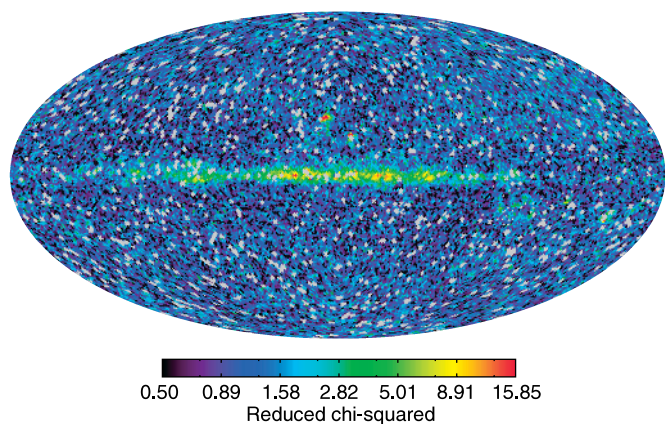
Figure 14. Map of the reduced \chi^2 per pixel achieved by the “base” fit. Except for a slight excess of high \chi^2 values from the plane, the overall statistical distribution is that of an ideal \chi^2 distribution.
