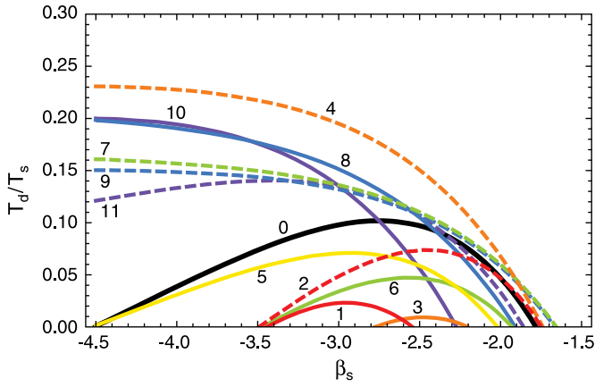
Figure 2. Slice in parameter space of the surface nulled by the ILC coefficients, assuming a three-component foreground model with power-law spectral behavior, T(\nu) = T_s \nu^{\beta_s} + T_f \nu^{2.14} + T_d \nu^{\beta_d} . Each line is for a single ILC region, denoted by a number. The parameter space is T_f/T_s , T_d/T_s , \beta_s , \beta_d . For this plot, the x -axis is \beta_s and the y -axis is T_d/T_s . The parameters T_f/T_s and \beta_d are fixed at 0.7 and 1.8, respectively. Each color is a different ILC region. Despite the variety amongst ILC coefficients, they often null similar regions of parameter space.
