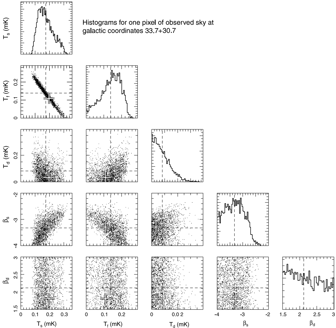
Figure 8. Histograms for foreground parameters for a single pixel of the observed sky from actual WMAP data, and not simulation. Dashed lines indicate the mean of the chain and crosses indicate the best-fit point. The observed sky shows the same basic behavior as the simulated sky used for testing.
