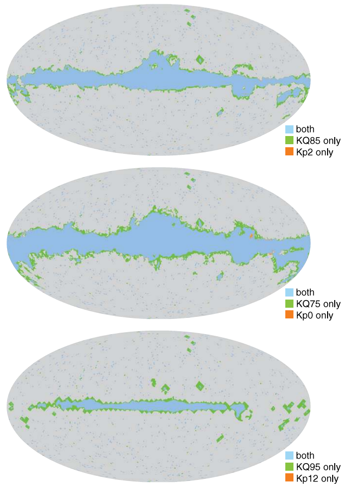
Figure 1. Comparison maps of the 5 year masks vs. the 3 year masks. The new masks cover slightly more of the Galactic plane and cover more regions with low synchrotron but high free–free emission. The diamond-shaped features arise because the new processing mask has been defined to correspond to low-resolution ( N_{\text{side}} = 16 ) pixels, so that the same processing mask can be used at all resolutions. Top: comparison of KQ85 with the 3 year Kp2 mask. Middle: comparison of KQ75 with the 3 year Kp0 mask. Bottom: comparison of KQ95 with the 3 year Kp12 mask.
