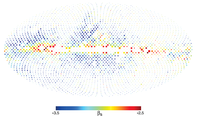
Figure 13. Map of the synchrotron spectral index for the “base” fit, binned to N_{\text{side}} = 16 . Color shows the value of the spectral index and the circle area indicates the weight \sigma_{\beta}^{-2} given by the fit. Pixels with \chi^2 > 2 were explicitly deweighted.
