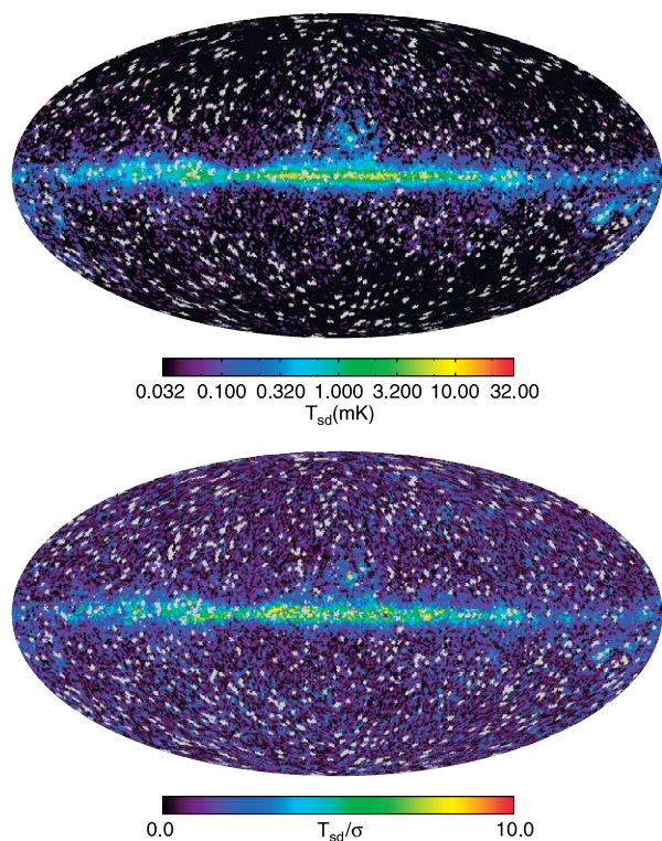
Figure 20. Top: map of possible spinning dust antenna temperature T_{sd} (as measured at the K band) for the “shifted” spinning dust model fit. While the model is based on a spinning dust spectrum, the data are insufficient for distinguishing the physical emission mechanism from other possibilities mentioned in the text. Maps of the other three foregrounds are qualitatively similar to that of the “base” model, with the synchrotron amplitude reduced somewhat to accommodate the additional low-frequency component. Bottom: map of spinning dust temperature divided by the marginalized temperature error as calculated by the MCMC chain. This is statistical error only and does not include uncertainties in the model.
