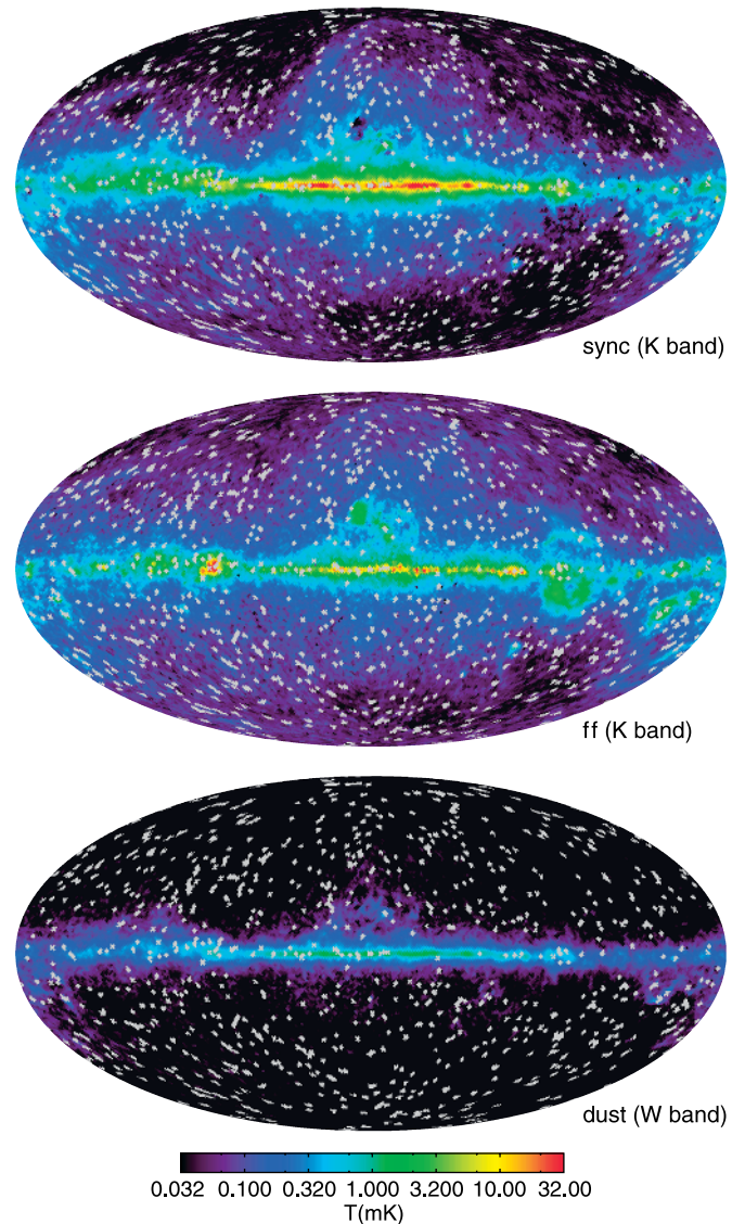
Figure 9. Temperature maps for foreground components as determined by the MCMC fitting process for the “base” model. Maps from other models are qualitatively similar. Synchrotron and free–free temperatures are as measured at the K band; dust is measured at the W band. Gray pixels are those masked due to point sources or flagged as problematic. Top: synchrotron, middle: free–free, bottom: dust.
