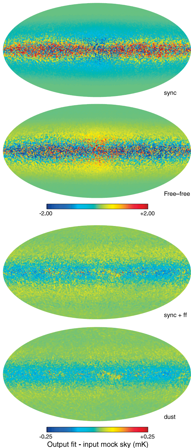
Figure 6. Difference maps between input and output foregrounds for the mock sky reconstruction. For comparison, the peak temperature for synchrotron plus free-free inputs was 17 mK, and for the input dust, the peak was 1.9 mK. The degeneracy between synchrotron and free-free emission means that their sum is much better constrained than either component individually. The scatter is larger than the bias, which is small compared to the input signal and within the error estimate given by the fit. These degeneracy issues are also illustrated in Figure 7. Synchrotron and free-free antenna temperatures are defined as measured at the K band and dust as measured at the W band.
