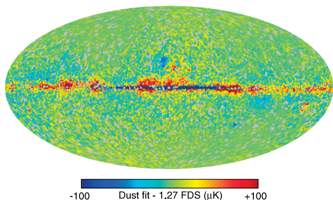
Figure 15. Residuals between the best-fit dust map from the “base” model and 1.27 times the “model 8” dust map of Finkbeiner et al. (1999) extrapolated to 94 GHz. Pixels with \chi^2_v > 5 or covered by the point-source mask are colored gray. The MCMC fit prefers less dust emission directly toward the Galactic center (deep blue pixels) and somewhat more emission further away (red and orange pixels). Units are antenna temperature at 94 GHz.
