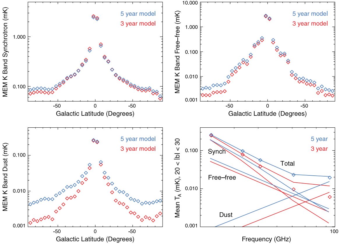
Figure 3. Comparison of MEM foreground modeling results from the WMAP 3 year and 5 year analyses. The first three panels show latitude profiles of antenna temperature for the individual foreground model components. The last panel compares the observed foreground emission spectrum (diamonds) with spectra of the total MEM model and the individual model components (line segments between WMAP frequencies), averaged over 20^\circ < |b| < 30^\circ . The differences between the 3 year and 5 year model results are mainly due to differences in zero levels between the 3 year and 5 year maps, and are consistent with the 3 year estimated error of \sim 4 \mu\text{K} . The mean model brightness exceeds the mean observed brightness at the higher frequencies because the observed brightness is negative for some pixels and the model is constrained to be positive for each pixel. This is less apparent in the 5 year results because there are fewer negative pixels.
