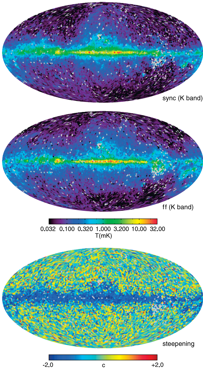
Figure 18. Maps for foreground components as determined by the MCMC fitting process for the “steep” model. This model has a frequency-dependent synchrotron spectral index \beta_s(\nu) = \beta_s + c \ln(\nu/\nu_K) . Synchrotron and free-free temperatures are measured at the K band, and gray pixels are those masked due to point sources or flagged as problematic. Since this model does not differ from the “base” model at high frequencies, the thermal dust emission is unaffected and is not shown. Note that the steepening parameter tends toward large negative values in the Galactic plane. Top: synchrotron, middle: free-free, bottom: steepening parameter c .
