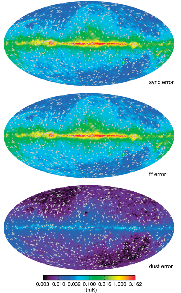
Figure 12. Error maps for foreground components as determined from the marginalized variance given by the MCMC fitting process. Error maps for synchrotron and free–free emission are similar due to the parameter degeneracy between them. Synchrotron and free–free temperatures are as measured at the K band; dust is measured at the W band. Gray pixels are those masked due to point sources or flagged as problematic. Top: synchrotron, middle: free–free, bottom: dust.
