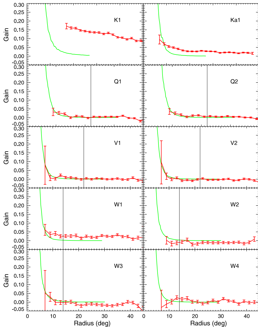
Figure 6. A-side augmented beam profiles ( green ) compared to Moon sidelobe data ( red ). K1 and Ka1 appear to be dominated by diffuse reflection rather than the extended main beam, and so are excluded from the fit. Conspicuous DA-to-DA differences are seen in the quality of the fit, e.g., W1 and W2 as compared to V1 and V2. Contamination of the fit by diffuse reflected light cannot be ruled out even in DAs other than K1 and Ka1; thus, the Moon data are best considered as upper limits. Vertical line: maximum radius of Moon data included in fit, for DAs Q1–W4.
